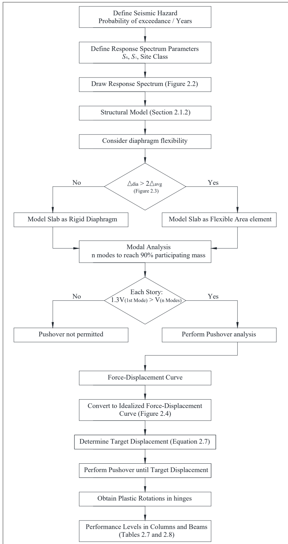
Figure 2.5: Performance Assessment Procedure in ASCE-41-13.
