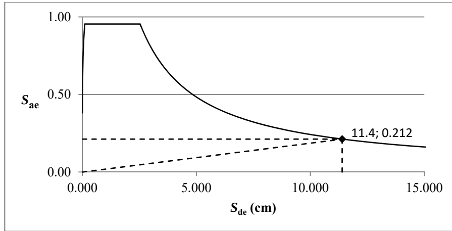
Figure 3.57: Target displacement computation, TBDY-16, Structure 5, direction y.
