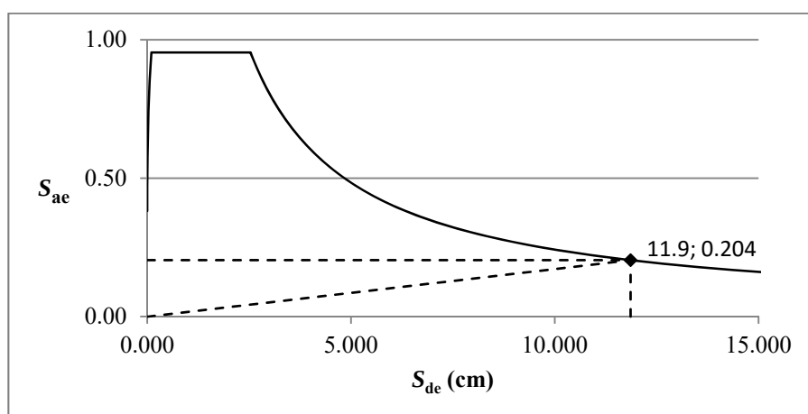
Figure 3.53: Target displacement computation, TBDY-16, Structure 3, direction y.
