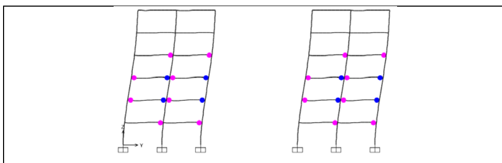
Figure A1.24: Hinge status at performance point, EN 1998-3, Structure 1, Frame 4.
