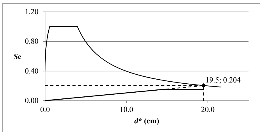
Figure 3.40: Target displacement computation, EN 1998-3, Structure 2, direction x.
