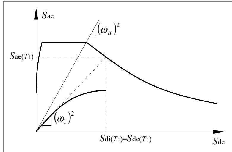
Figure 2.14: Determination of Inelastic displacement demand ( T_1 > T_B ).
