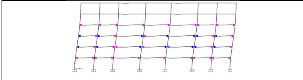
Figure A1.1: Hinge status at performance point, ASCE-41-13, Structure 1, Frame B.
