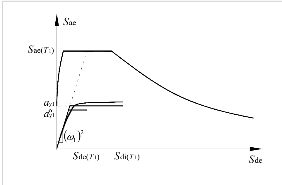
Figure 2.16: Determination of Inelastic displacement demand ( T_1 < T_B ).
