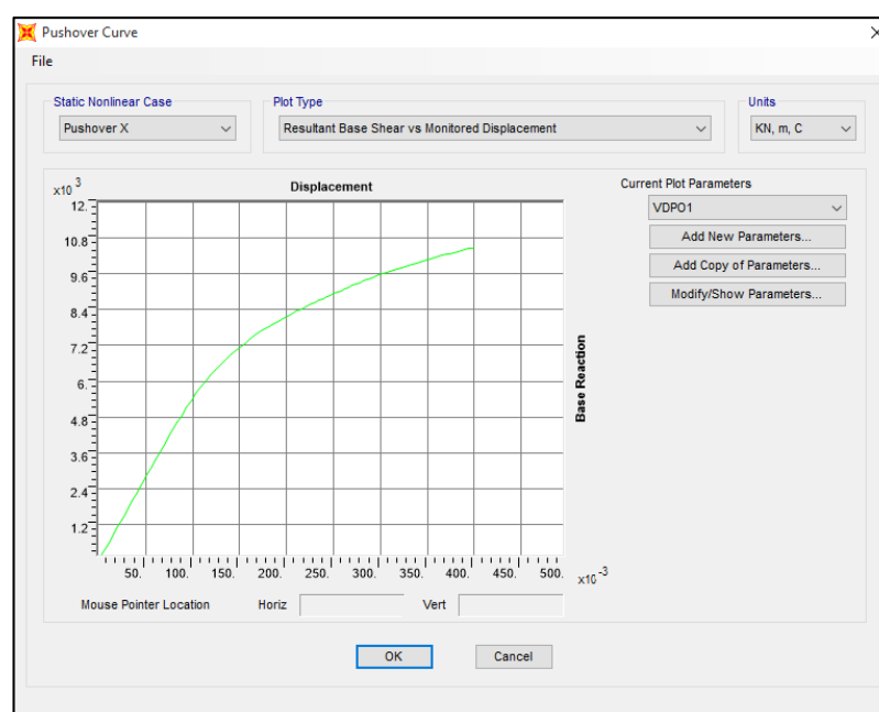
Figure 3.20: Pushover curve from SAP2000, Structure 1, direction x, ASCE-41-13.
