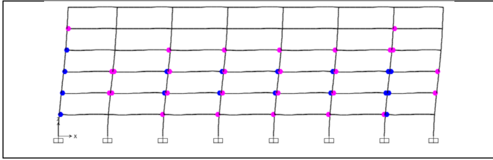
Figure A1.53: Hinge status at performance point, TBDY-16, Structure 4, Frame A.
