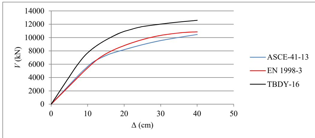
Figure 3.26: Pushover curve, Structure 3, Mode 2 (y direction).
