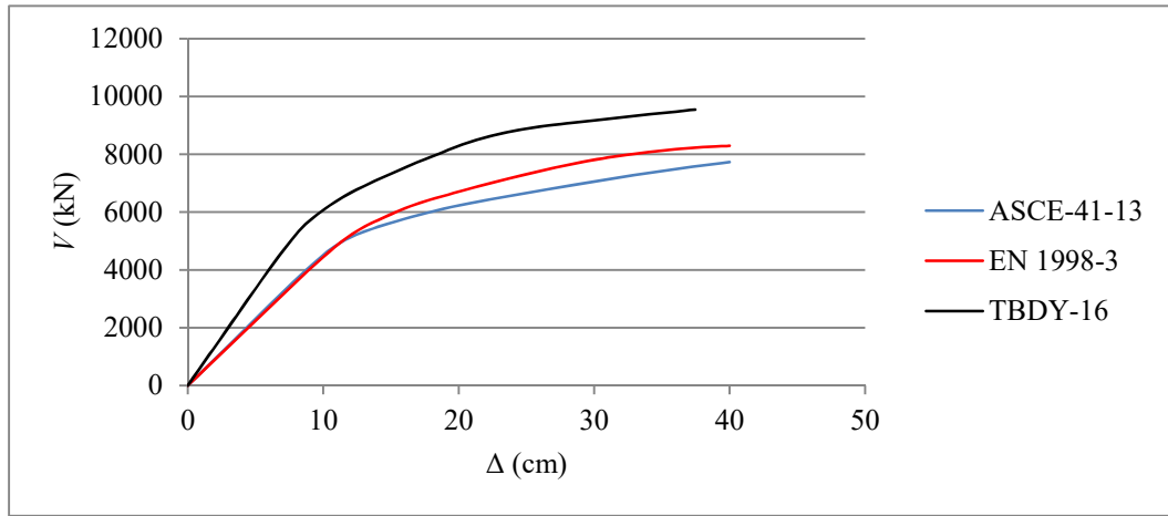
Figure 3.24: Pushover curve, Structure 2, Mode 2 (y direction).
