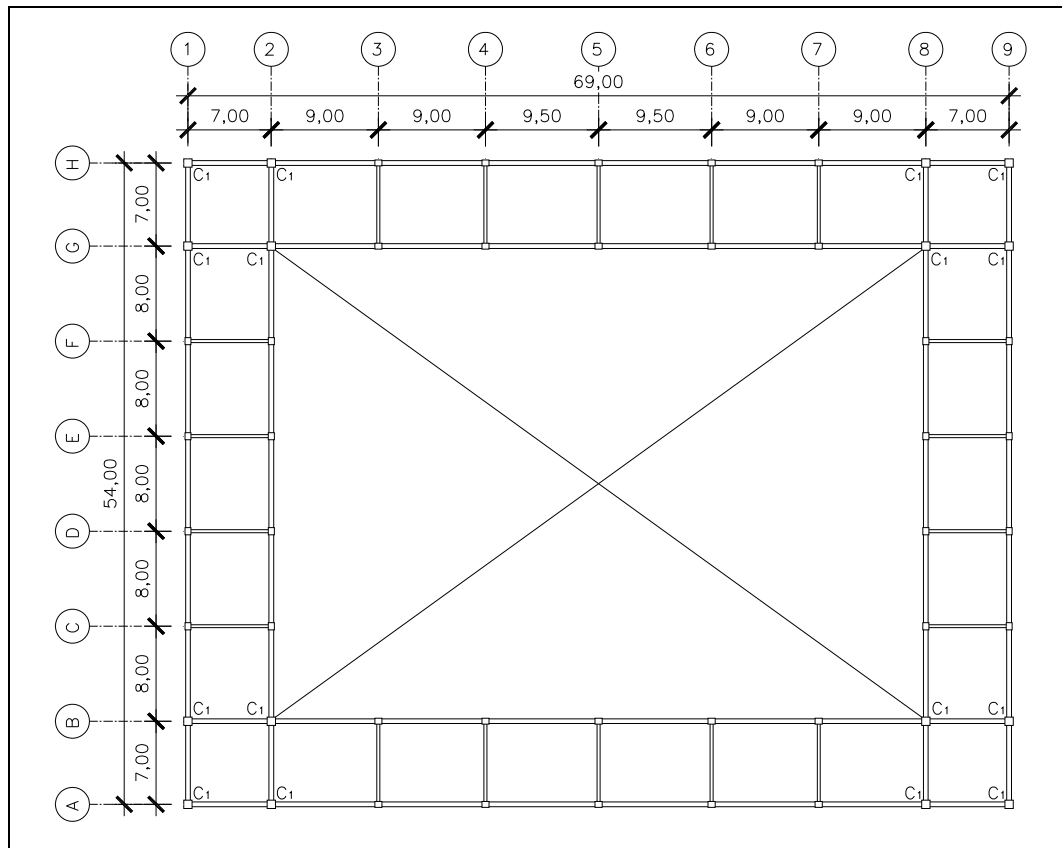
Figure 3.9: Typical floor plan for 6 story Structure 5 (60%).
