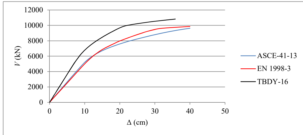
Figure 3.22: Pushover curve, Structure 1, Mode 2 (x direction).
