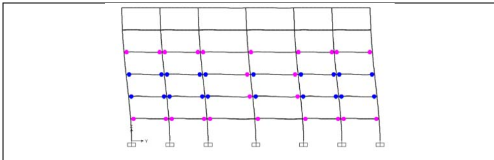
Figure A1.43: Hinge status at performance point, TBDY-16, Structure 1, Frame 2.
