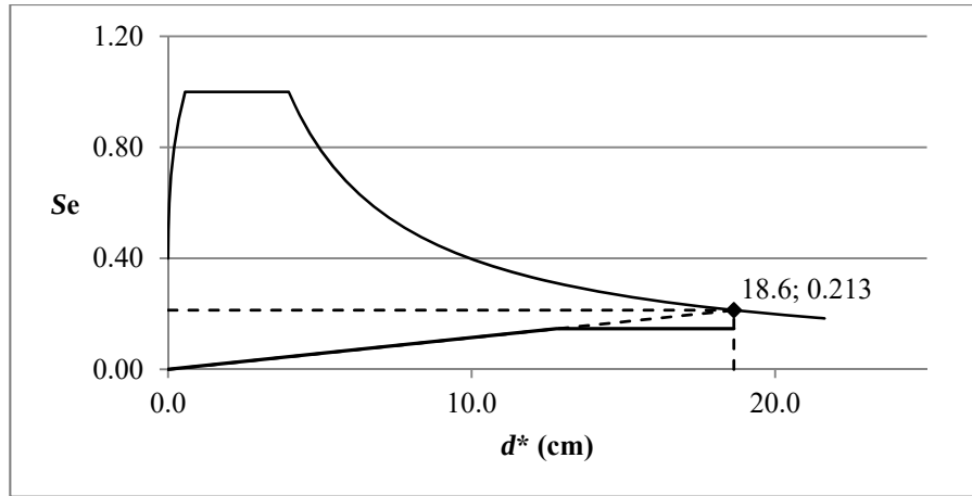
Figure 3.47: Target displacement computation, EN 1998-3, Structure 5, direction y.
