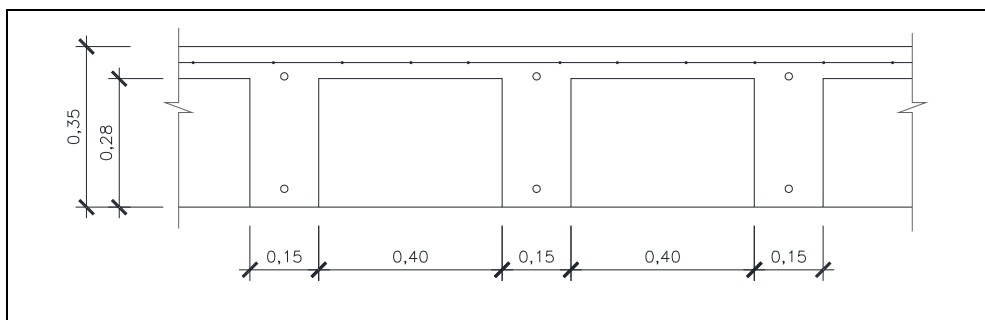
Figure 3.13: Slab section in Structure 4 and Structure 5.
