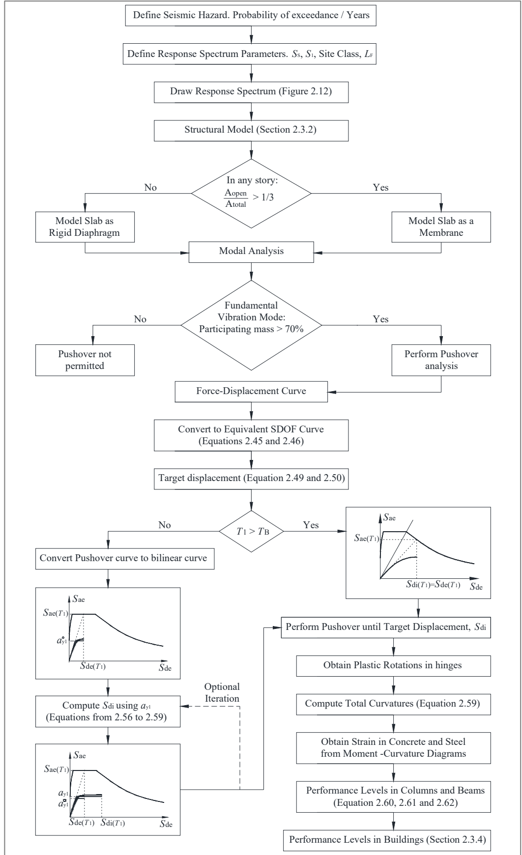
Figure 2.18: Performance Assessment Procedure in TBDY-16.
