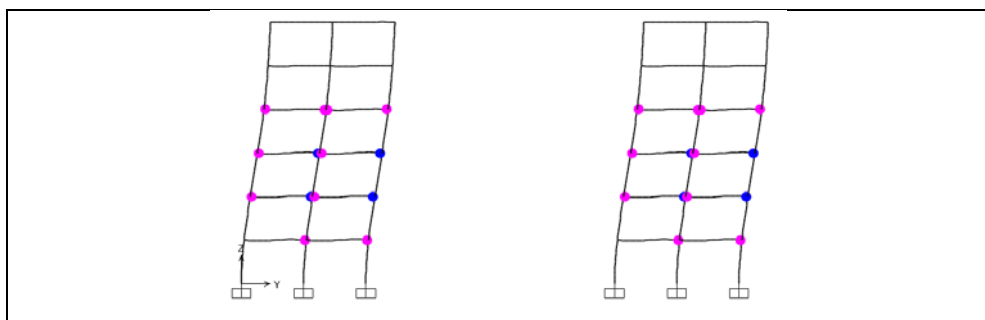
Figure A1.28: Hinge status at performance point, EN 1998-3, Structure 2, Frame 5.
