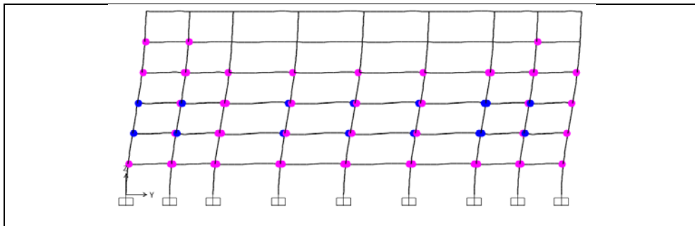
Figure A1.11: Hinge status at performance point, ASCE-41-13, Structure 3, Frame 2.
