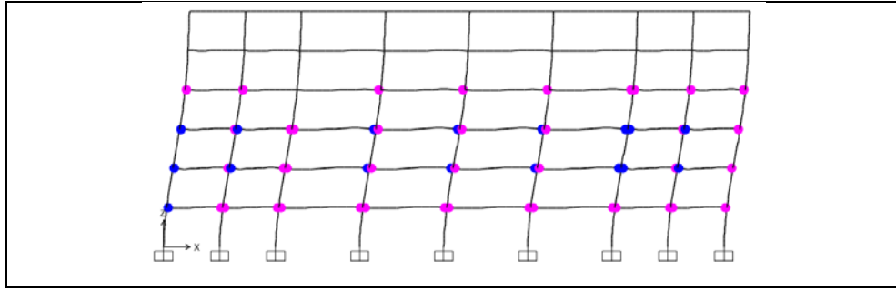
Figure A1.5: Hinge status at performance point, ASCE-41-13, Structure 2, Frame B.
