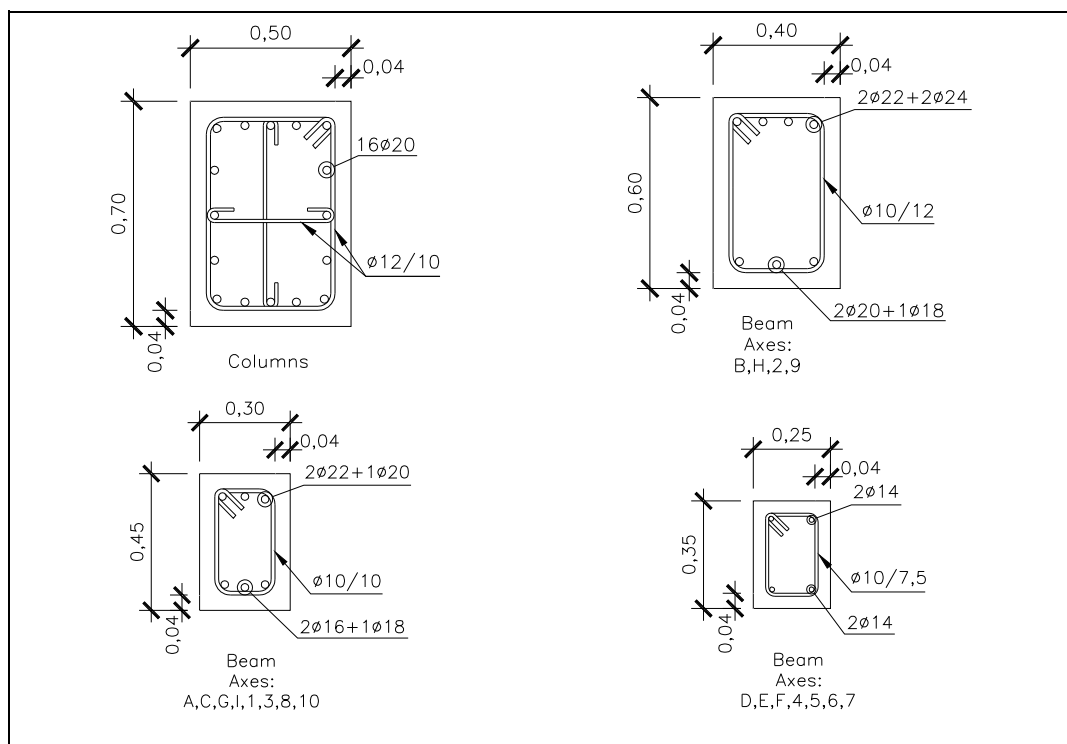
Figure 3.6: Section of the Elements in Structure 3 (40%).
