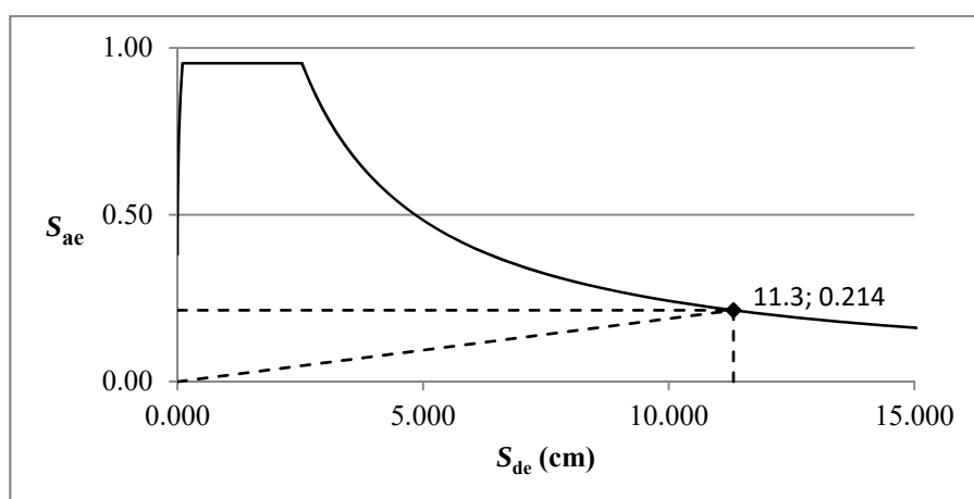
Figure 3.56: Target displacement computation, TBDY-16, Structure 5, direction x.
