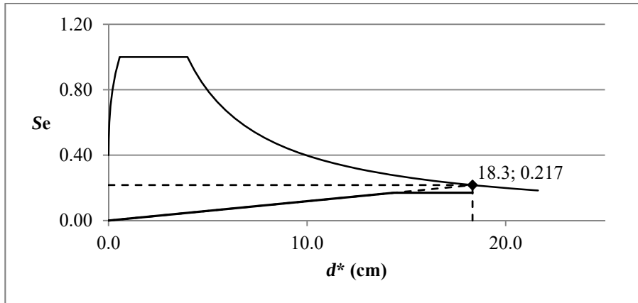
Figure 3.37: Target displacement computation, Structure 1, direction x, third iteration.
