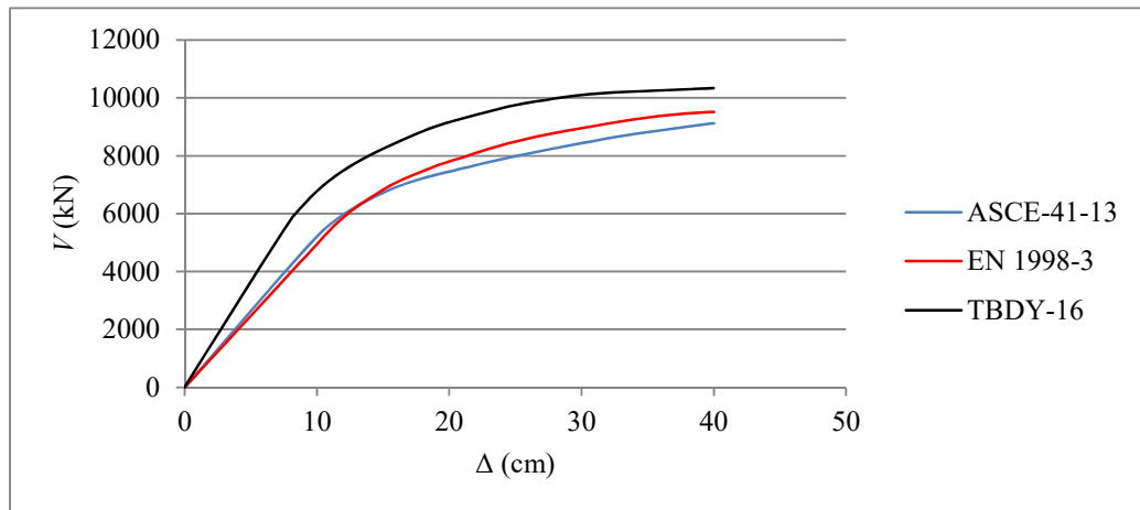
Figure 3.27: Pushover curve, Structure 4, Mode 1 (y direction).
