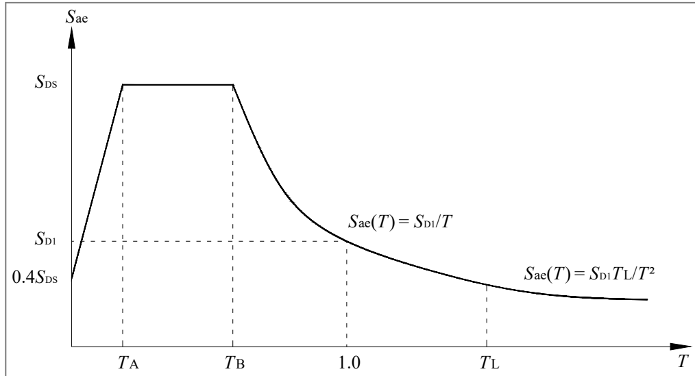
Figure 2.12: General Horizontal Response Spectrum.
