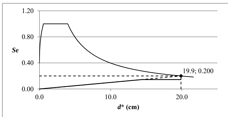
Figure 3.45: Target displacement computation, EN 1998-3, Structure 4, direction y.
