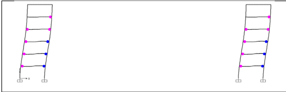
Figure A1.18: Hinge status at performance point, ASCE-41-13, Structure 5,Frame D.
