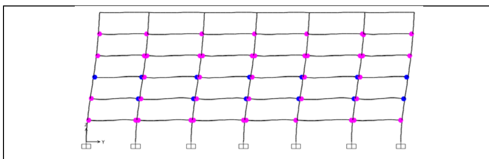
Figure A1.35: Hinge status at performance point, EN 1998-3, Structure 4, Frame 1.
