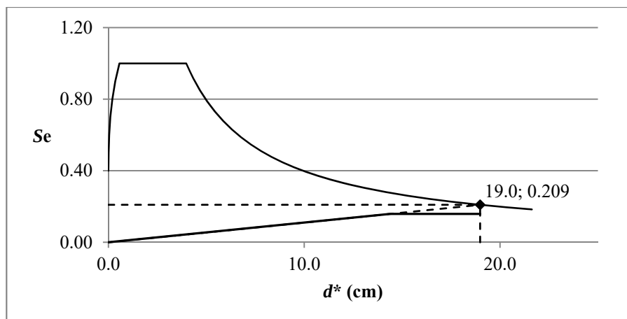
Figure 3.44: Target displacement computation, EN 1998-3, Structure 4, direction x.
