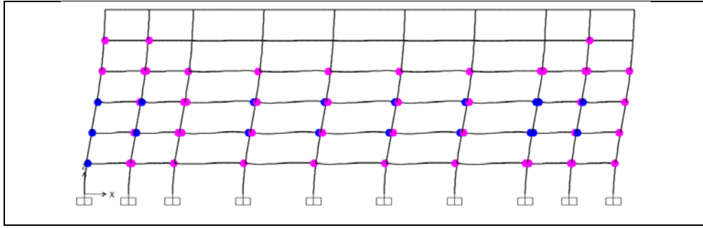
Figure A1.9: Hinge status at performance point, ASCE-41-13, Structure 3, Frame B.
