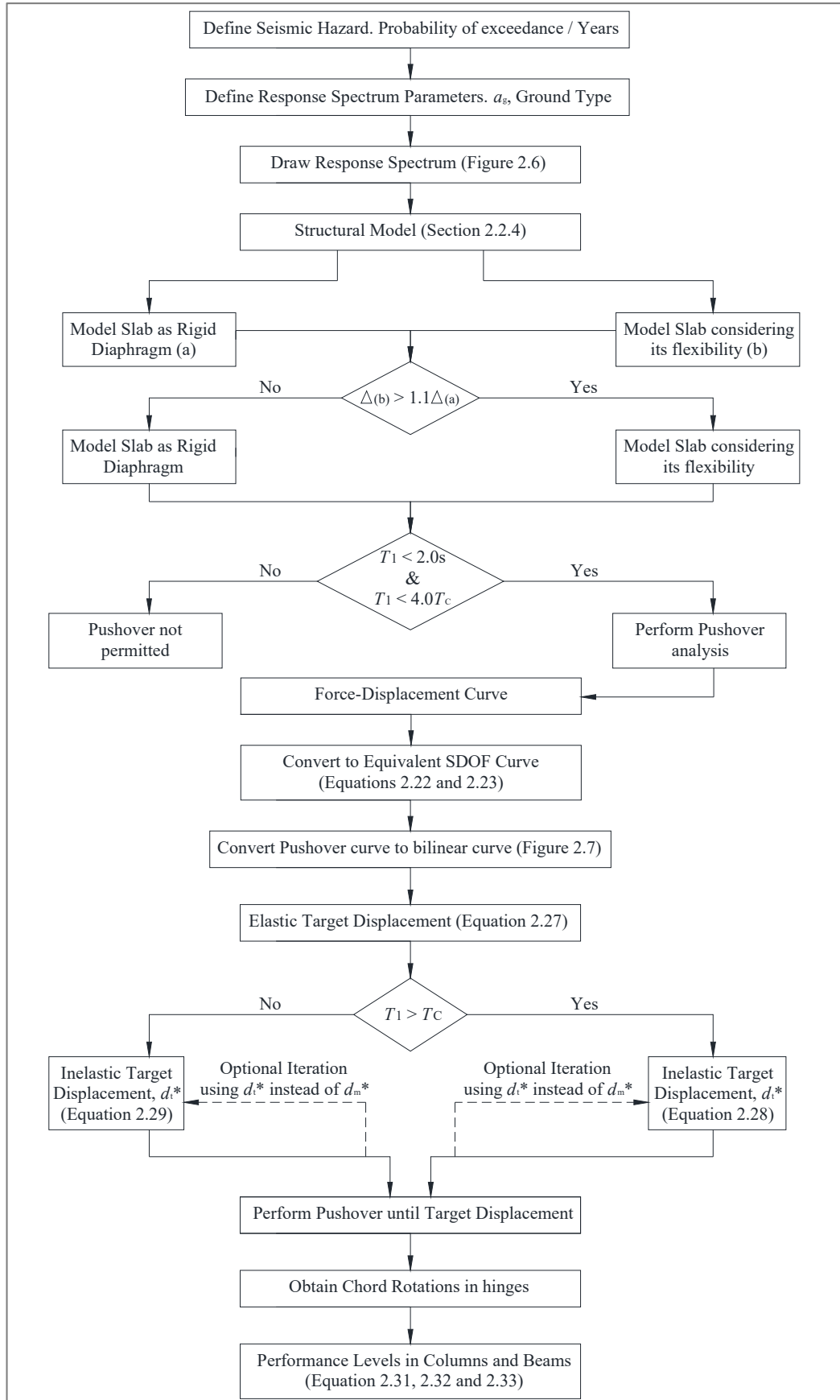
Figure 2.11: Performance Assessment Procedure in EN 1998-3.
