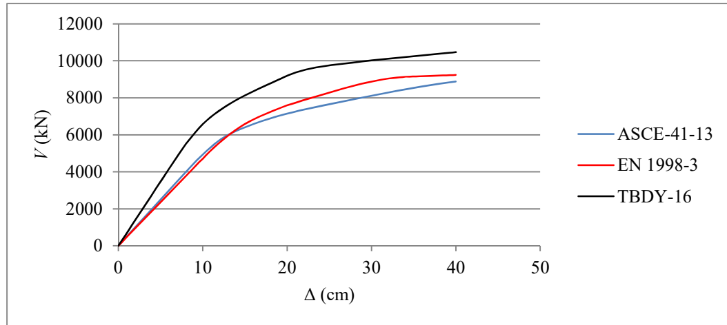
Figure 3.21: Pushover curve, Structure 1, Mode 1 (y direction).
