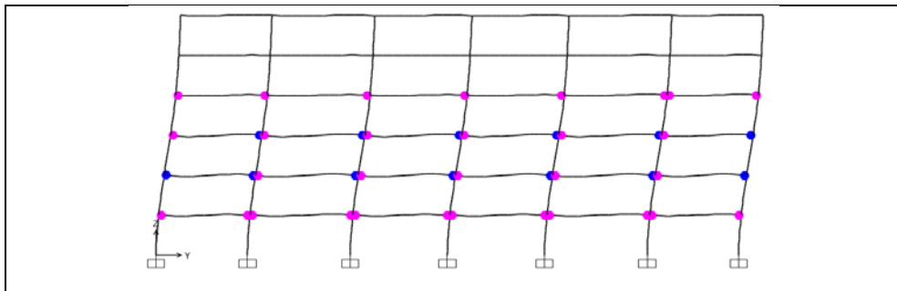
Figure A1.15: Hinge status at performance point, ASCE-41-13, Structure 4, Frame 1.
