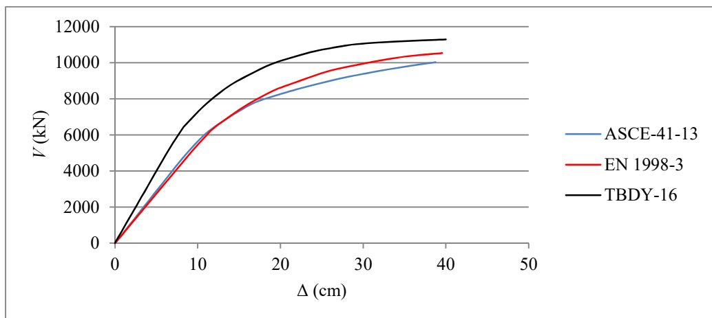
Figure 3.28: Pushover curve, Structure 4, Mode 2 (x direction).
