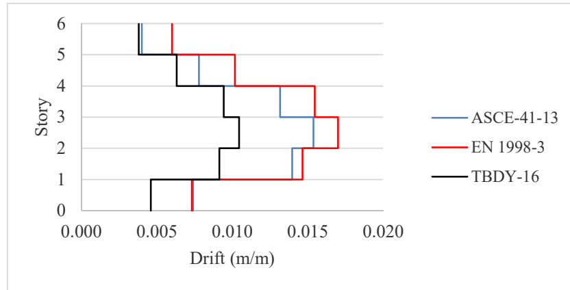
Figure 3.58: Drift ( \Delta/h ), Structure 1, x direction.
