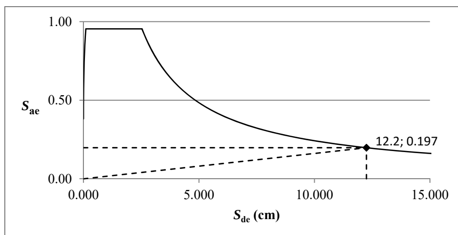
Figure 3.55: Target displacement computation, TBDY-16, Structure 4, direction y.
