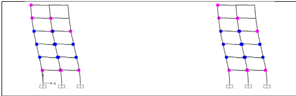
Figure A1.50: Hinge status at performance point, TBDY-16, Structure 3, Frame E.
