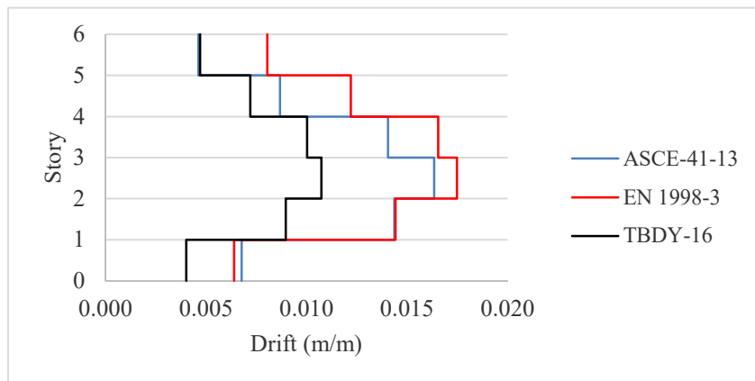
Figure 3.63: Drift ( \Delta/h ), Structure 3, y direction.
