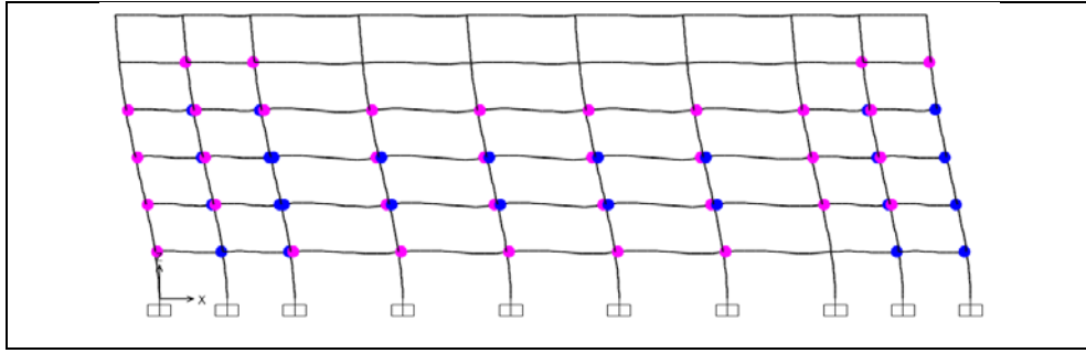
Figure A1.49: Hinge status at performance point, TBDY-16, Structure 3, Frame B.
