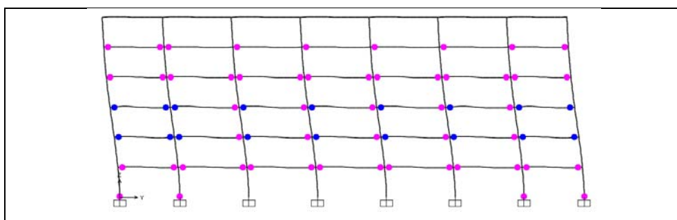
Figure A1.39: Hinge status at performance point, EN 1998-3, Structure 5, Frame 1.
