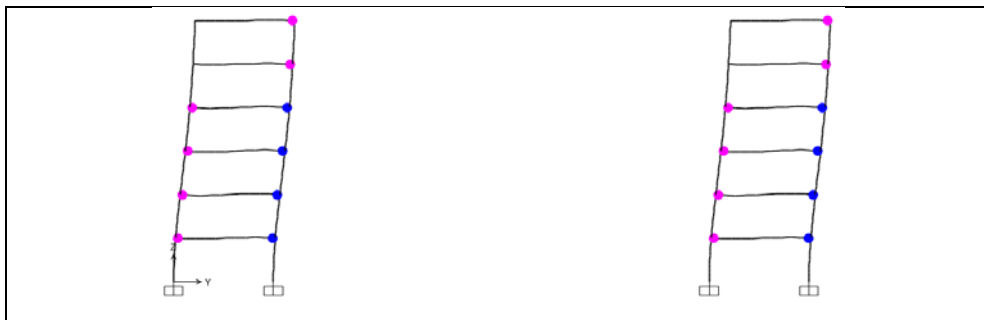
Figure A1.56: Hinge status at performance point, TBDY-16, Structure, 4, Frame 4.
