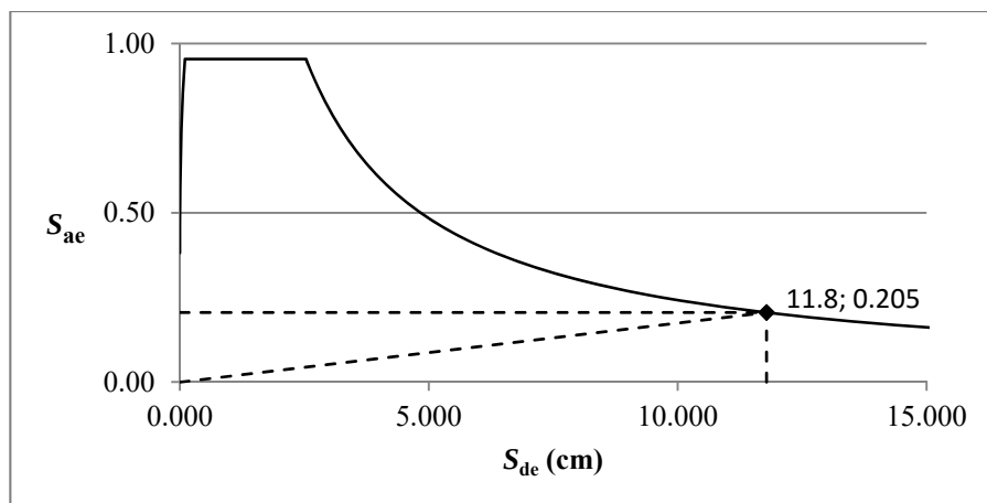
Figure 3.51: Target displacement computation, TBDY-16, Structure 2, direction y.
