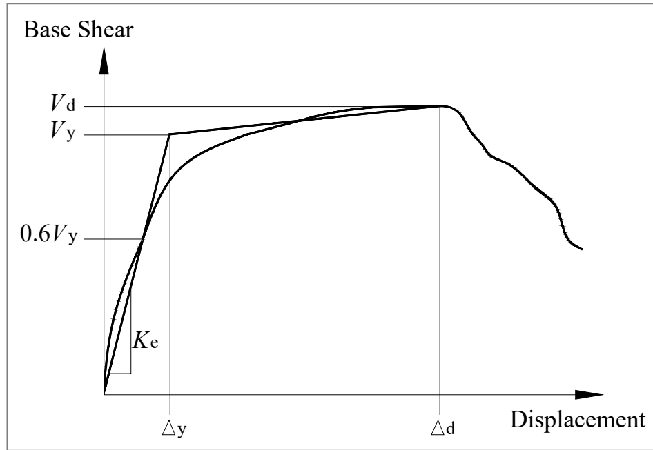
Figure 2.4: Idealized Force-Displacement Curve.
