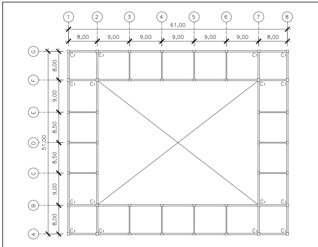
Figure 3.7: Typical floor plan for 6 story Structure 4 (50%).
