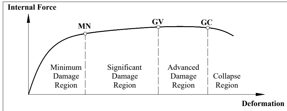
Figure 2.17: Damage levels in sections and elements.
