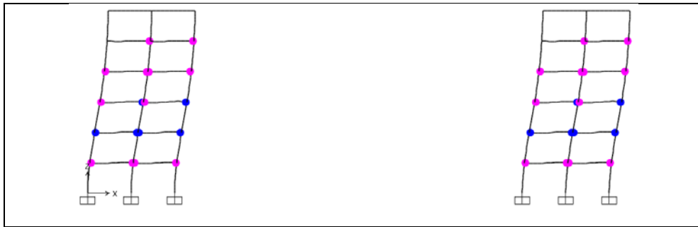
Figure A1.10: Hinge status at performance point, ASCE-41-13, Structure 3, Frame E.
