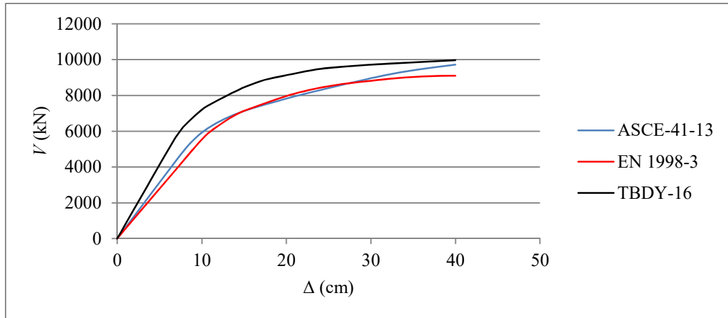
Figure 3.29: Pushover curve, Structure 5, Mode 1 (y direction).
