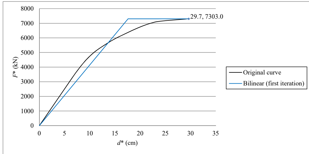
Figure 7.33: Bilinear Pushover curve, Structure 1, direction x, first iteration.
