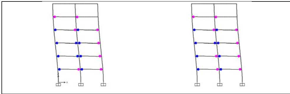
Figure A1.42: Hinge status at performance point, TBDY-16, Structure 1, Frame D.
