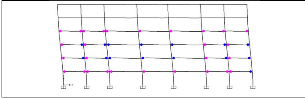
Figure A1.41: Hinge status at performance point, TBDY-16, Structure 1, Frame B.
