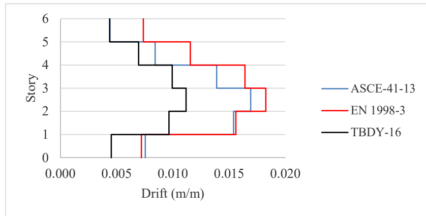
Figure 3.62: Drift ( \Delta/h ), Structure 3, x direction.
