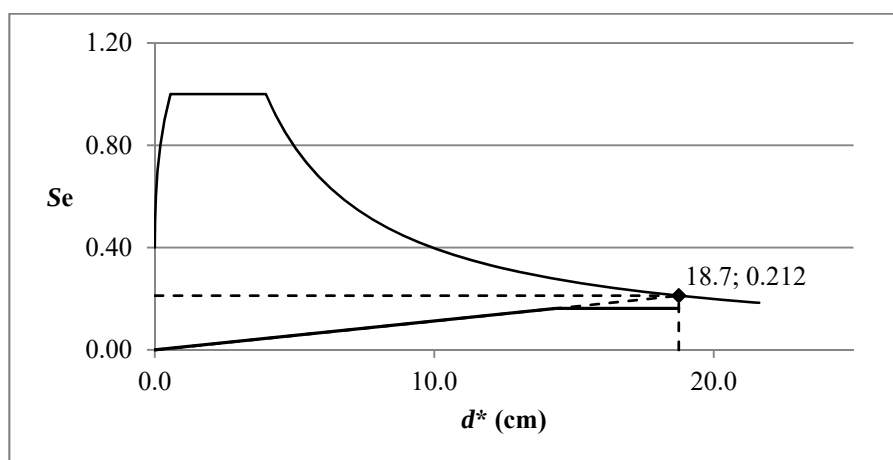
Figure 3.39: Target displacement computation, EN 1998-3, Structure 1, direction y.
