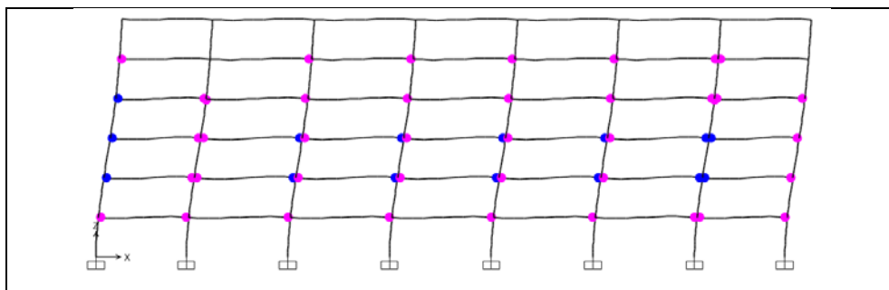
Figure A1.33: Hinge status at performance point, EN 1998-3, Structure 4, Frame A.
