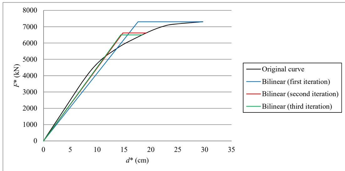
Figure 3.35: Bilinear Pushover curve, Structure 1, direction x, first, second and third iteration.
