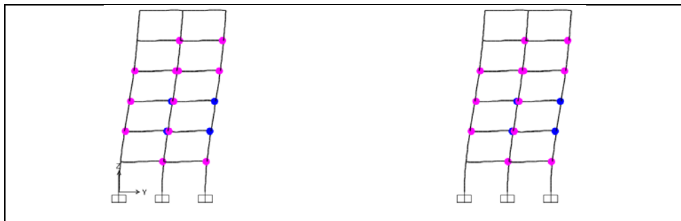
Figure A1.32: Hinge status at performance point, EN 1998-3, Structure, 3, Frame 5.
