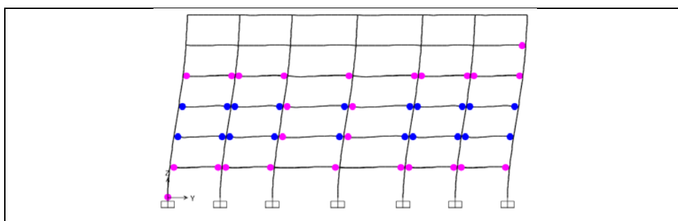
Figure A1.23: Hinge status at performance point, EN 1998-3, Structure 1, Frame 2.
