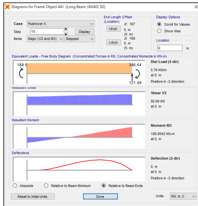
Figure 3.69 Deformed shape and internal forces in element 443.
