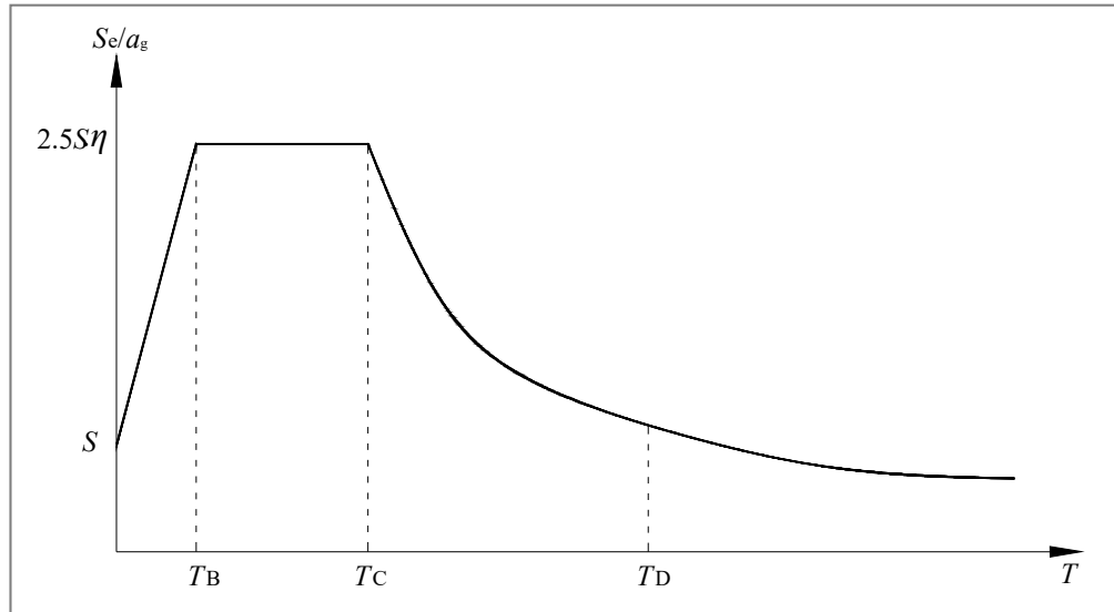
Figure 2.6: Shape of the Elastic Response Spectrum.
