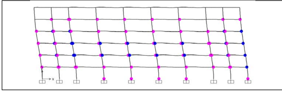
Figure A1.29: Hinge status at performance point, EN 1998-3, Structure 3, Frame B.
