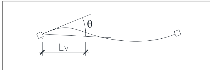
Figure 2.10: Chord Rotation.
