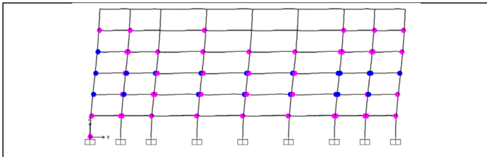
Figure A1.51: Hinge status at performance point, TBDY-16, Structure 3, Frame 2.
