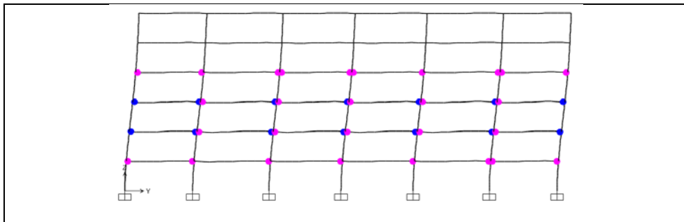
Figure A1.55: Hinge status at performance point, TBDY-16, Structure 4, Frame 1.
