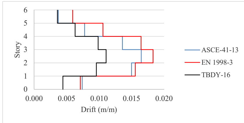
Figure 3.61: Drift ( \Delta/h ), Structure 2, y direction.
