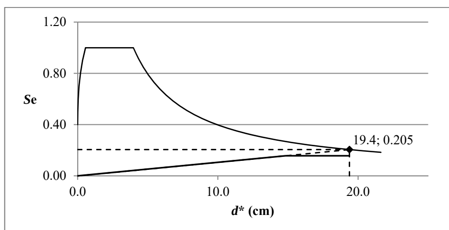
Figure 3.43: Target displacement computation, EN 1998-3, Structure 3, direction y.
