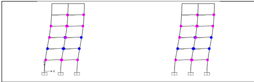
Figure A1.6: Hinge status at performance point, ASCE-41-13, Structure 2, Frame D.
