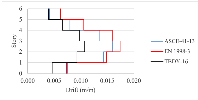
Figure 3.59: Drift ( \Delta/h ), Structure 1, y direction.
