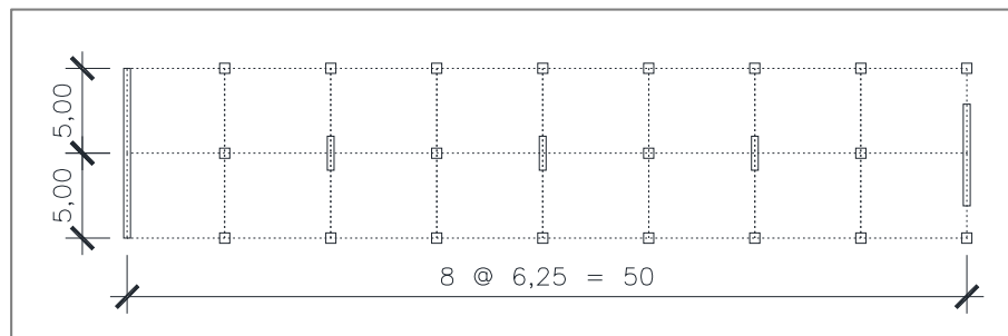
Figure 1.2: Typical floor plan of Three-Story Building.
