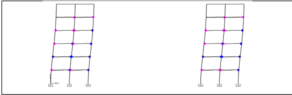
Figure A1.46: Hinge status at performance point, TBDY-16, Structure 2, Frame D.
