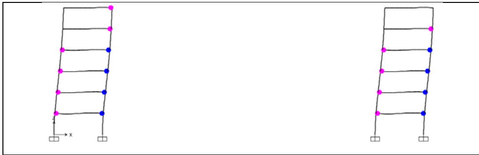
Figure A1.54: Hinge status at performance point, TBDY-16, Structure 4, Frame D.
