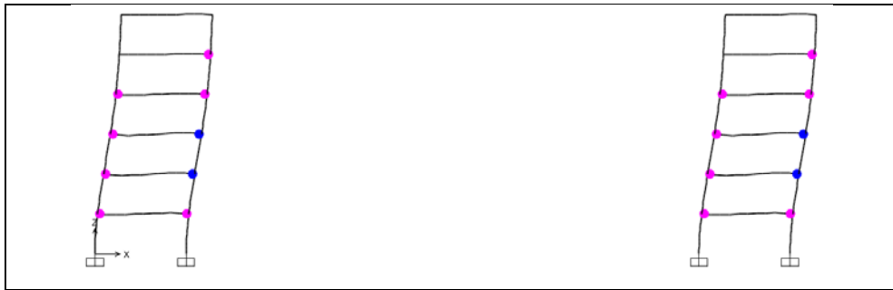
Figure A1.14: Hinge status at performance point, ASCE-41-13, Structure 4,Frame D.
