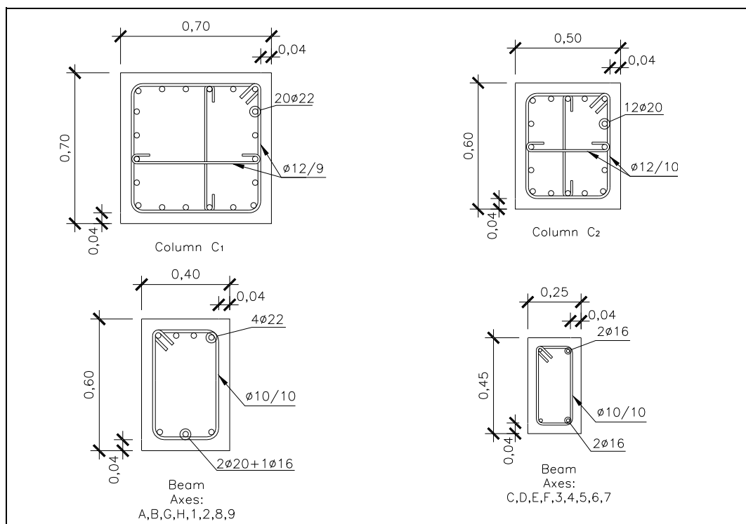
Figure 3.10: Section of the Elements in Structure 5 (60%).
