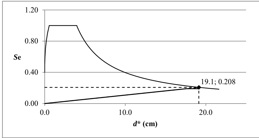
Figure 3.34: Target displacement computation, Structure 1, direction x, first iteration.
