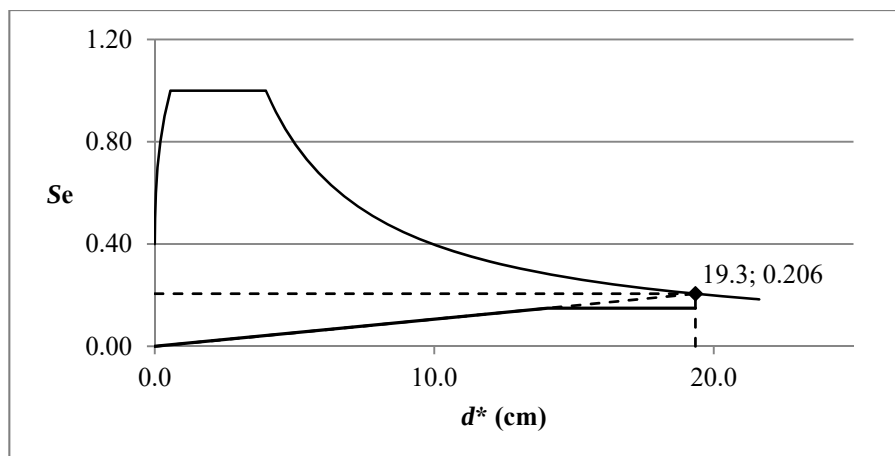
Figure 3.41: Target displacement computation, EN 1998-3, Structure 2, direction y.
