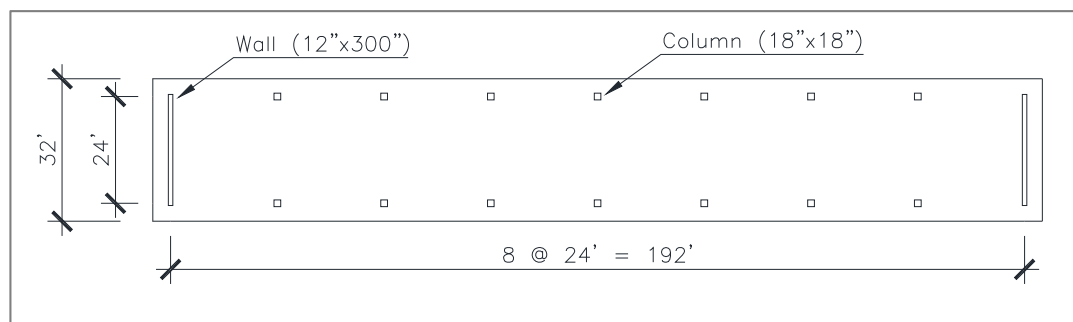
Figure 1.1: Typical floor plan of Eight-Span Three-Story Structure.
