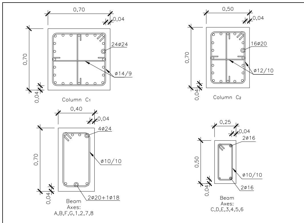
Figure 3.8: Section of the Elements in Structure 4 (50%).
