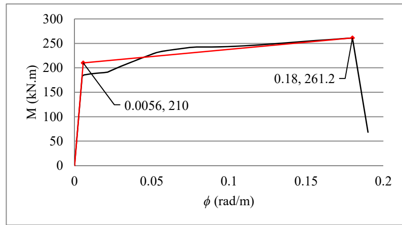
Figure 3.72 Moment-curvature diagram in 40x60cm section beam.
