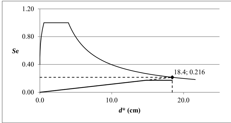
Figure 3.36: Target displacement computation, Structure 1, direction x, second iteration.
