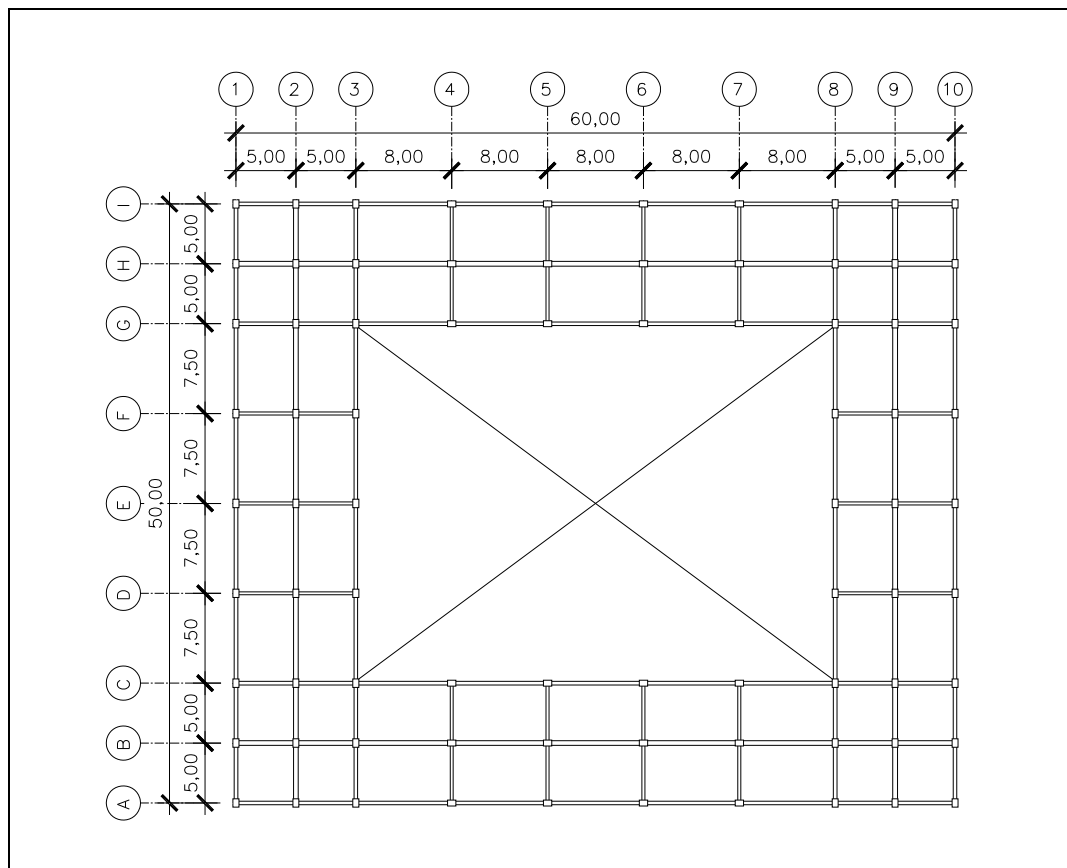
Figure 3.5: Typical floor plan for 6 story Structure 3 (40%).
