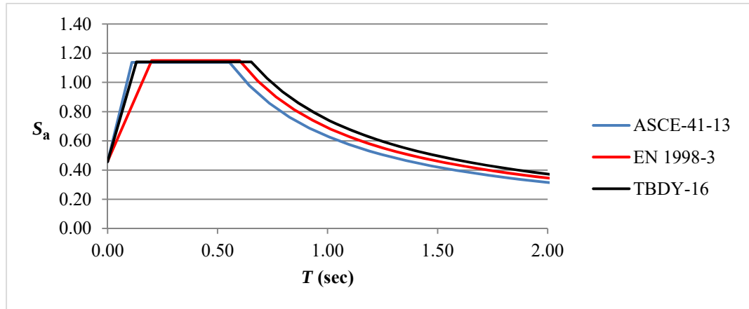
Figure 2.20: Response Spectrum Comparison ( S_s=1.06 , S_1=0.39 , a_g=0.4 , Soil: Sand).
