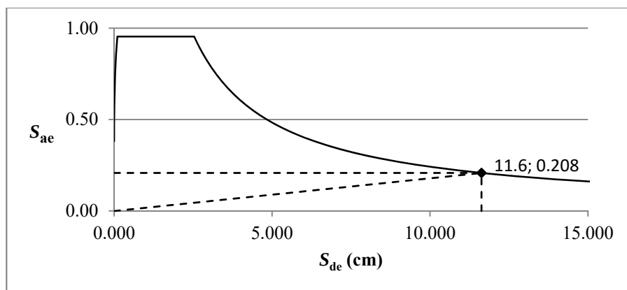
Figure 3.49: Target displacement computation, TBDY-16, Structure 1, direction y.
