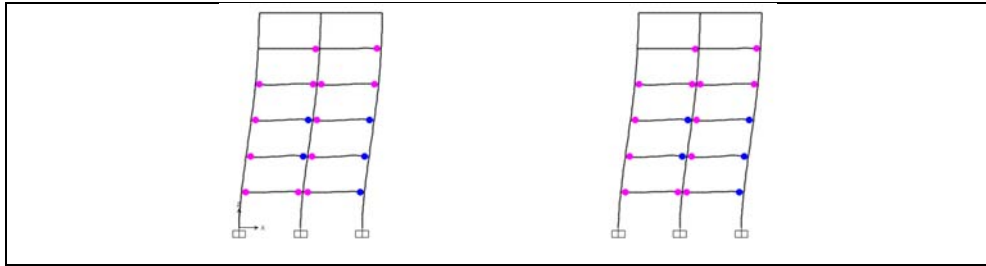
Figure A1.2: Hinge status at performance point, ASCE-41-13 Structure 1, Frame D.
