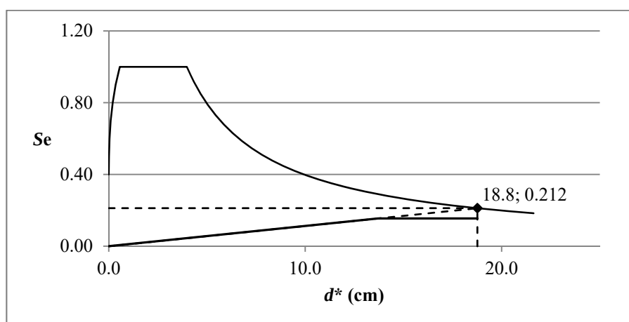
Figure 3.46: Target displacement computation, EN 1998-3, Structure 5, direction x.
