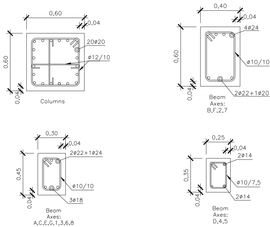
Figure 3.2: Section of the Elements in Structure 1 (20%).
