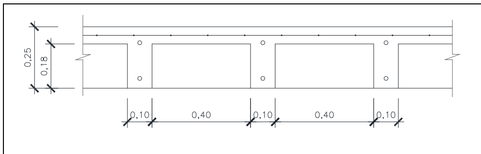
Figure 3.12: Slab section in Structure 1, Structure 2 and Structure 3.
