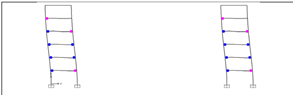
Figure A1.60: Hinge status at performance point, TBDY-16, Structure, 5, Frame 5.
