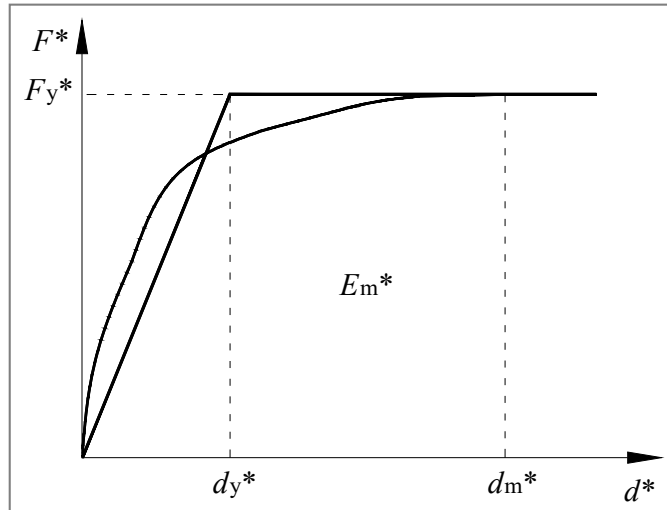
Figure 2.7: Bilinear equivalent SDOF Force-Displacement curve.
