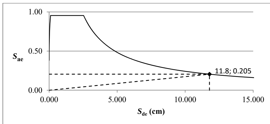
Figure 3.50: Target displacement computation, TBDY-16, Structure 2, direction x.
