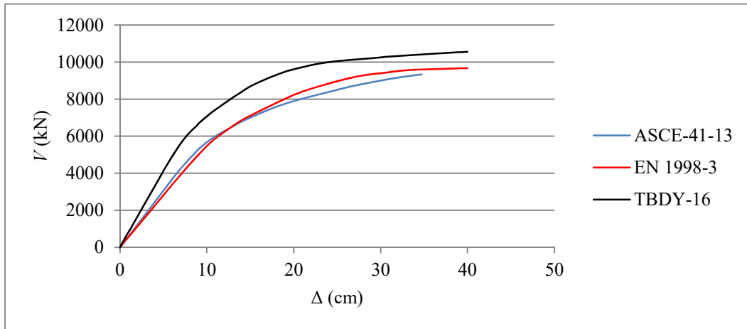
Figure 3.30: Pushover curve, Structure 5, Mode 2 (x direction).
