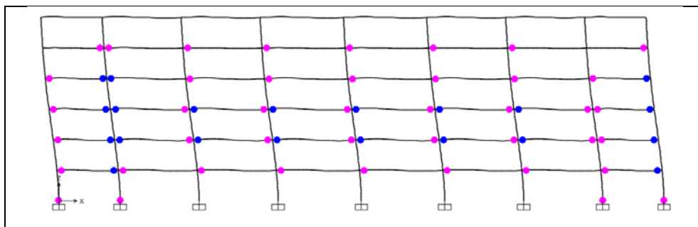
Figure A1.37: Hinge status at performance point, EN 1998-3, Structure 5, Frame A.
