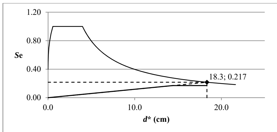
Figure 3.38: Target displacement computation, EN 1998-3, Structure 1, direction x.
