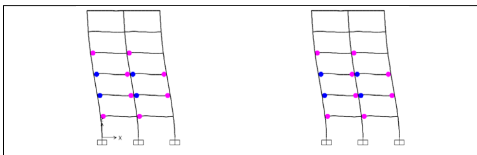
Figure A1.22: Hinge status at performance point, EN 1998-3, Structure 1, Frame D.
