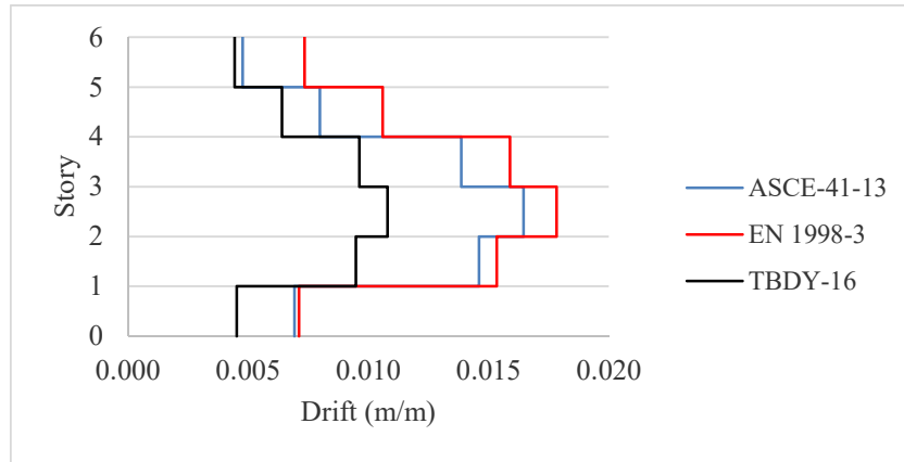
Figure 3.64: Drift ( \Delta/h ), Structure 4, x direction.
