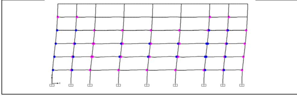
Figure A1.45: Hinge status at performance point, TBDY-16, Structure 2, Frame B.
