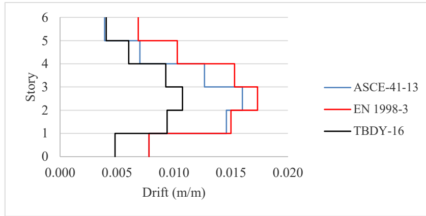
Figure 3.67: Drift ( \Delta/h ), Structure 5, y direction.
