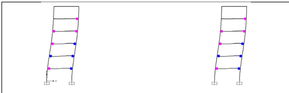
Figure A1.20: Hinge status at performance point, ASCE-41-13, Structure 5, Frame 5.
