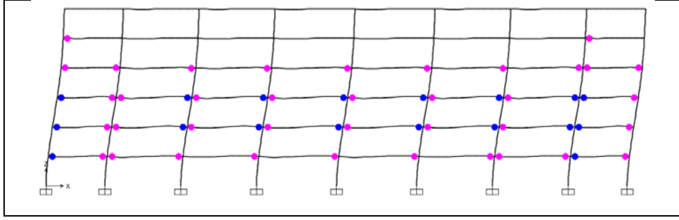
Figure A1.17: Hinge status at performance point, ASCE-41-13, Structure 5,Frame A.
