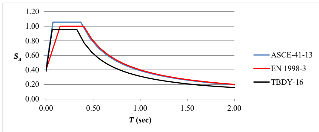
Figure 2.19: Response Spectrum Comparison ( S_s=1.06 , S_1=0.39 , a_g=0.4 , Soil: Rock).
