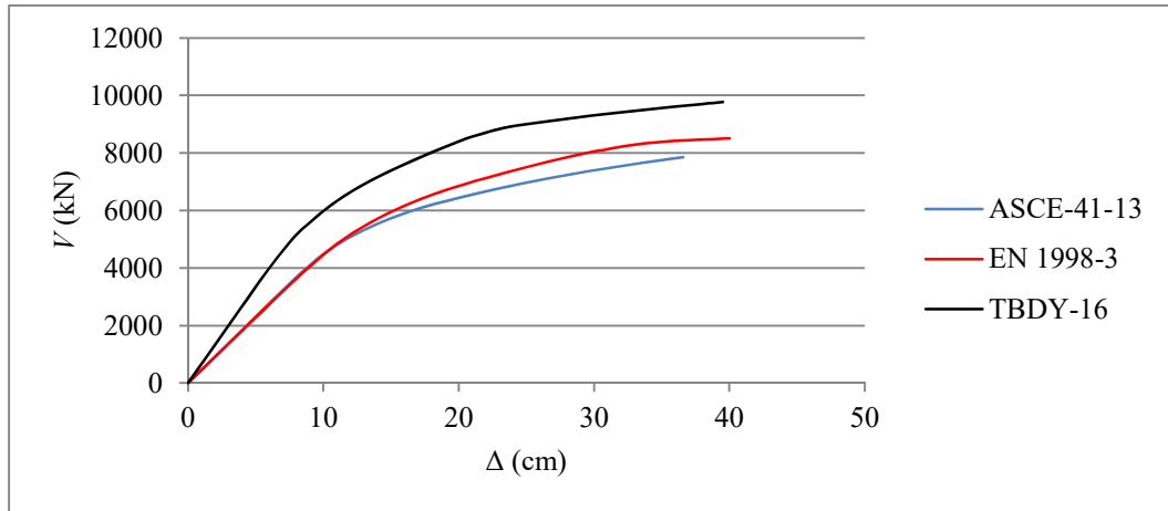
Figure 3.23: Pushover curve, Structure 2, Mode 1 (x direction).
