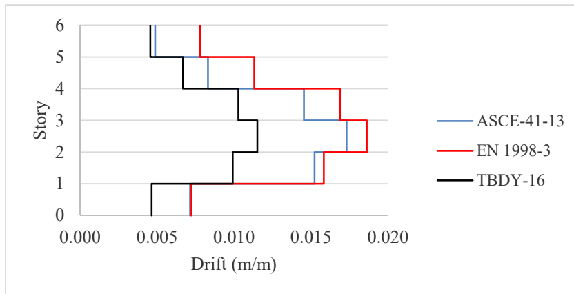
Figure 3.65: Drift ( \Delta/h ), Structure 4, y direction.
