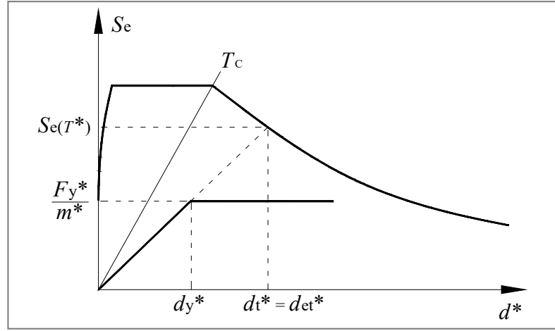
Figure 2.8: Determination of target displacement for the equivalent SDOF system (Medium and long period range).
