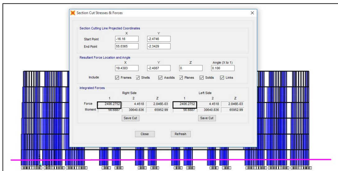
Figure 3.19: Shear story resulting from ten modes, Structure 3, direction x.
