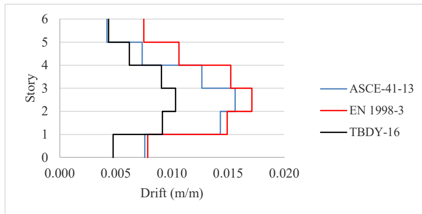
Figure 3.66: Drift ( \Delta/h ), Structure 5, x direction.
