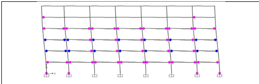
Figure A1.59: Hinge status at performance point, TBDY-16, Structure 5, Frame 1.
