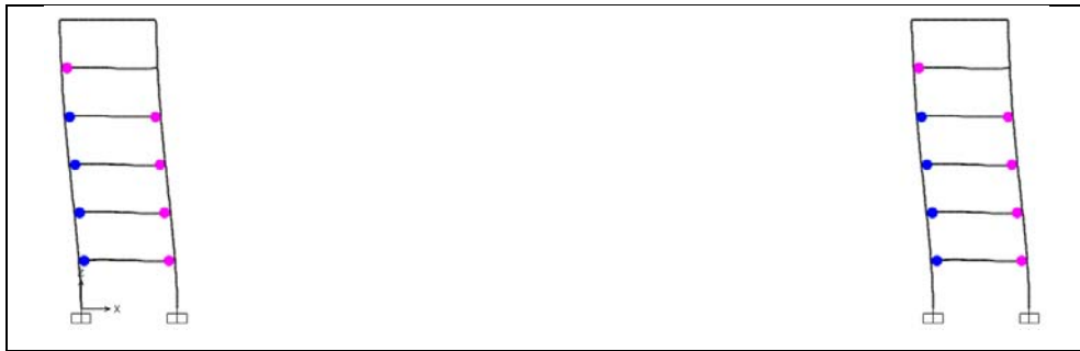
Figure A1.58: Hinge status at performance point, TBDY-16, Structure 5, Frame D.
