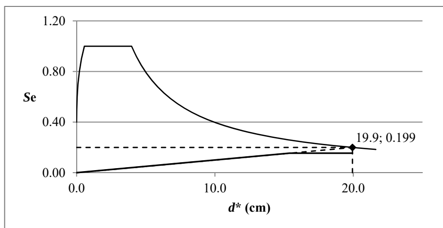
Figure 3.42: Target displacement computation, EN 1998-3, Structure 3, direction x.
