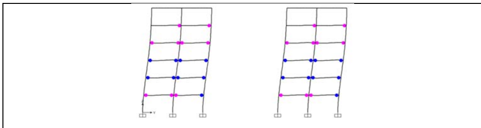
Figure A1.4: Hinge status at performance point, ASCE-41-13, Structure 1, Frame 4.
