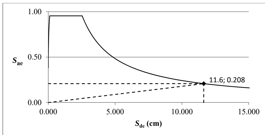
Figure 3.54: Target displacement computation, TBDY-16, Structure 4, direction x.
