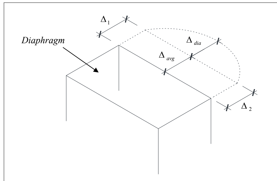
Figure 2.3: Deformation in diaphragms.
