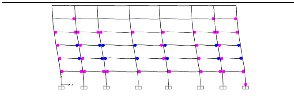
Figure A1.21: Hinge status at performance point, EN 1998-3, Structure 1, Frame B.
