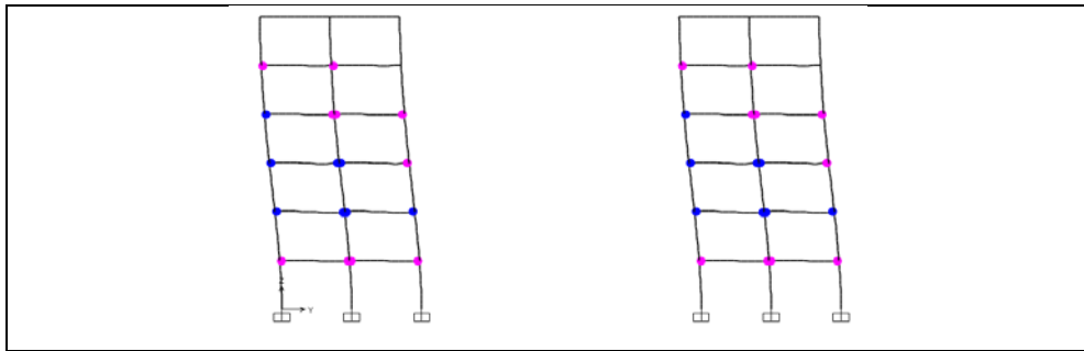
Figure A1.48: Hinge status at performance point, TBDY-16, Structure, 2, Frame 5.
