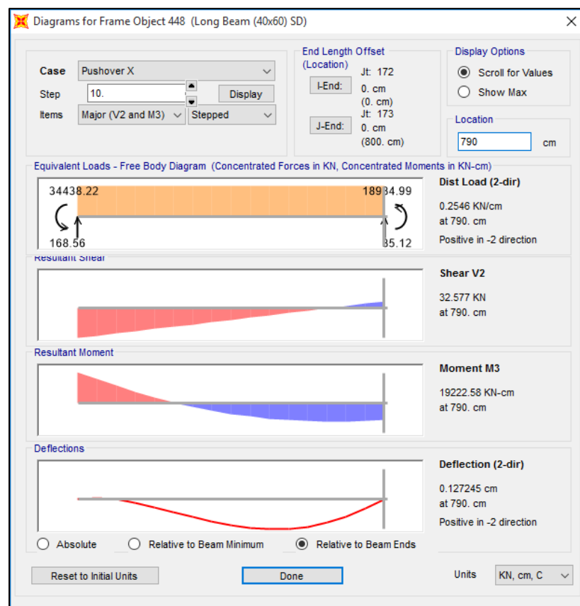
Figure 3.71: Deformed shape and internal forces in element 448.
