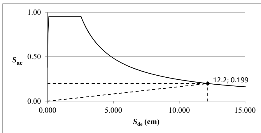
Figure 3.52: Target displacement computation, TBDY-16, Structure 3, direction x.
