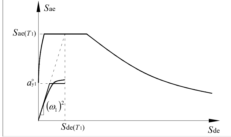
Figure 2.15: Bilinear SDOF Force-Displacement Curve.
