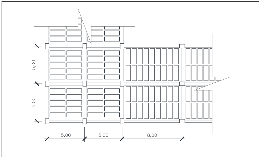
Figure 3.11: Typical Slab Plan.
