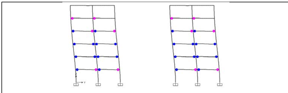
Figure A1.44: Hinge status at performance point, TBDY-16, Structure, 1, Frame 4.
