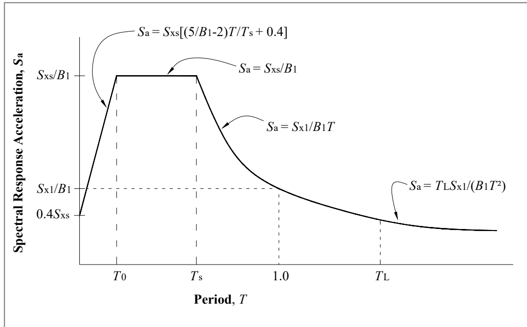
Figure 2.2: General Horizontal Response Spectrum.
