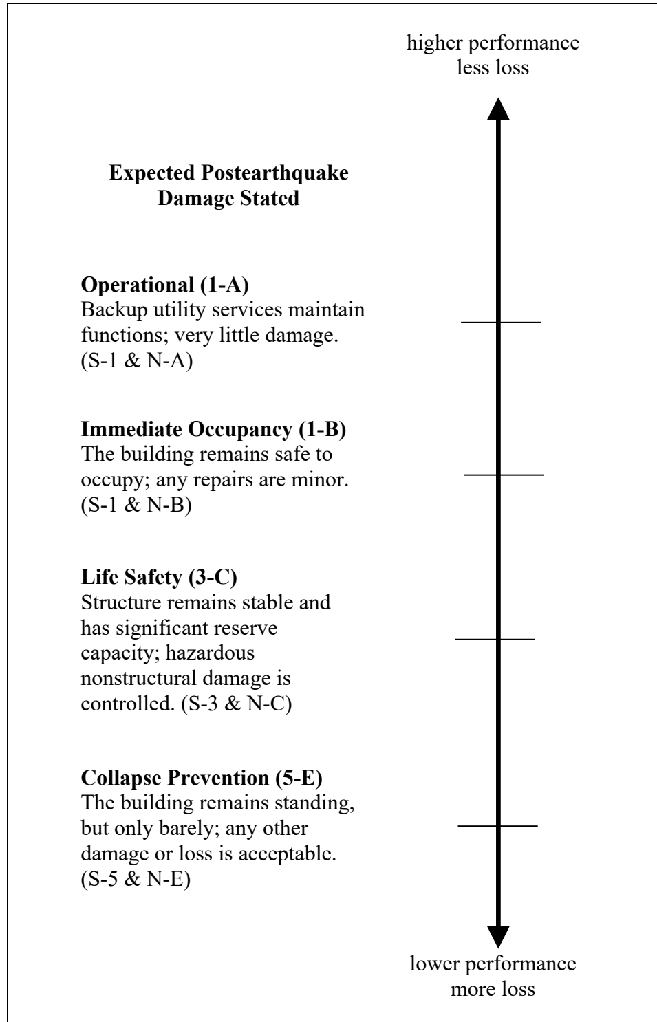
Figure 2.1: Target building Performance Levels.
