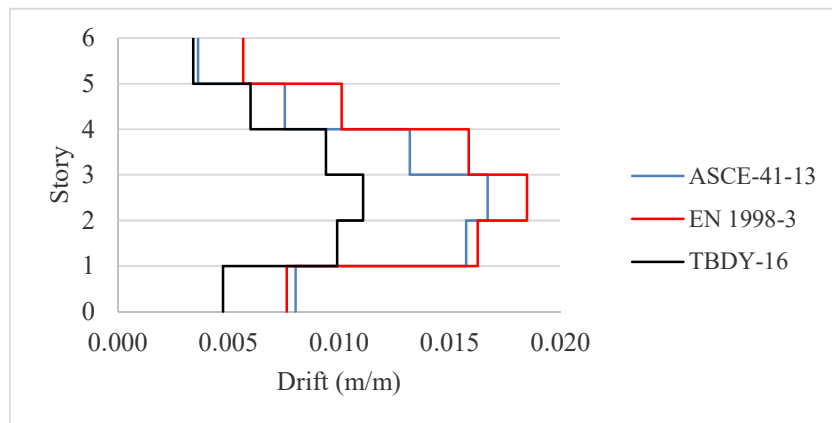
Figure 3.60: Drift ( \Delta/h ), Structure 2, x direction.
