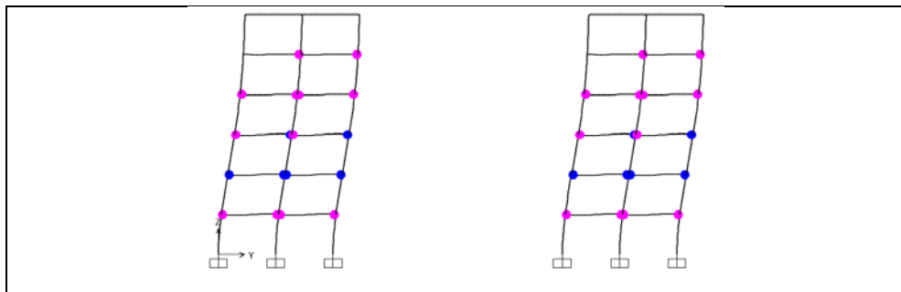
Figure A1.8: Hinge status at performance point, ASCE-41-13, Structure 2, Frame 5.
