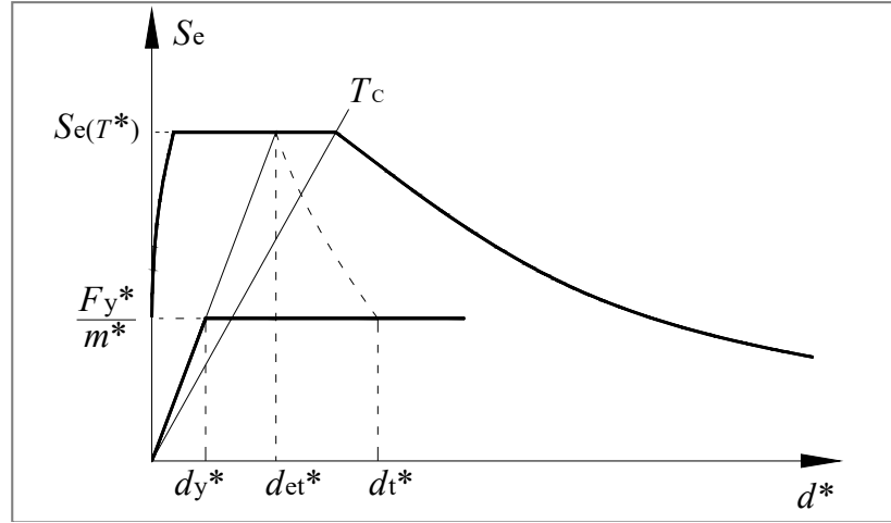
Figure 2.9: Determination of target displacement for the equivalent SDOF system (Short period range).
