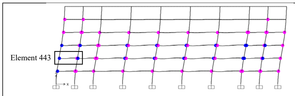
Figure 3.68: Deformed shape, Structure 3, Frame B.
