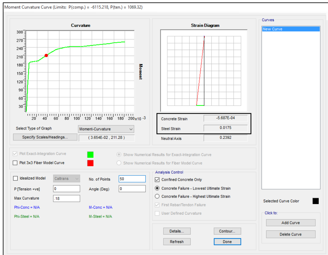
Figure 3.74: Strains in concrete and steel for 0.037rad/m curvature.
