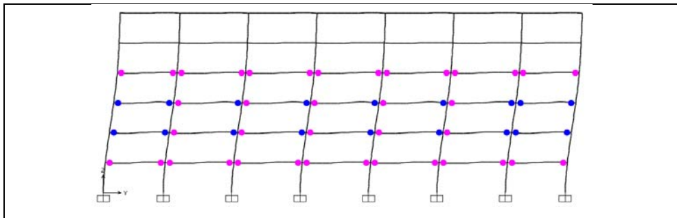
Figure A1.19: Hinge status at performance point, ASCE-41-13, Structure 5, Frame 1.
