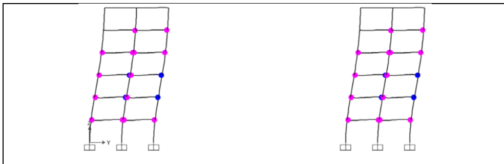
Figure A1.12: Hinge status at performance point, ASCE-41-13, Structure 3, Frame 5.
