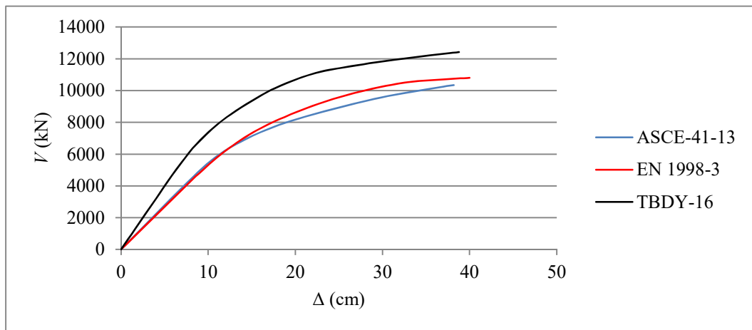
Figure 3.25: Pushover curve, Structure 3, Mode 1 (x direction).
