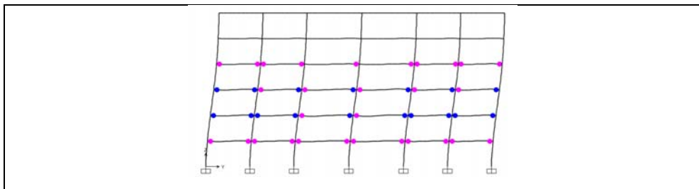
Figure A1.3: Hinge status at performance point, ASCE-41-13, Structure 1, Frame 2.
