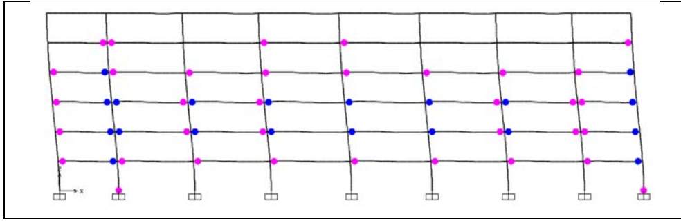
Figure A1.57: Hinge status at performance point, TBDY-16, Structure 5, Frame A.
