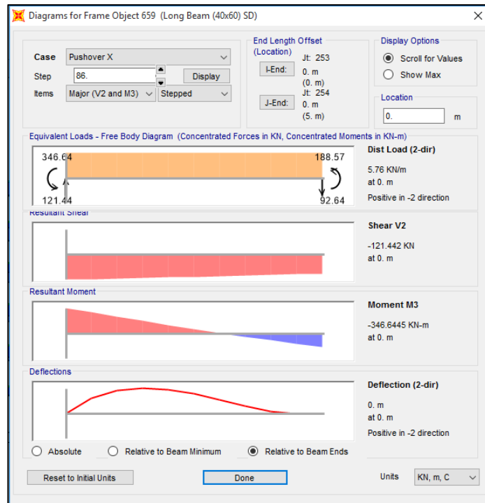
Figure 3.73: Deformed and internal forces in element 659.
