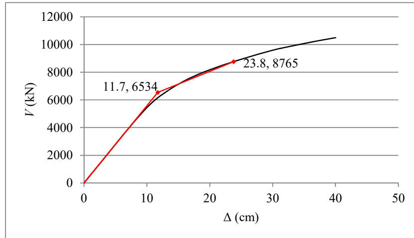
Figure 3.32: Bilinear Pushover curve, Structure 3, direction x, second iteration.
