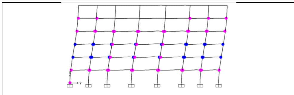
Figure A1.27: Hinge status at performance point, EN 1998-3, Structure 2, Frame 2.
