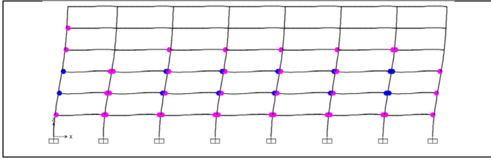
Figure A1.13: Hinge status at performance point, ASCE-41-13, Structure 4,Frame A.
