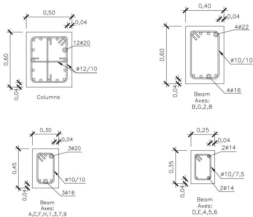
Figure 3.4: Section of the Elements in Structure 2 (30%).
