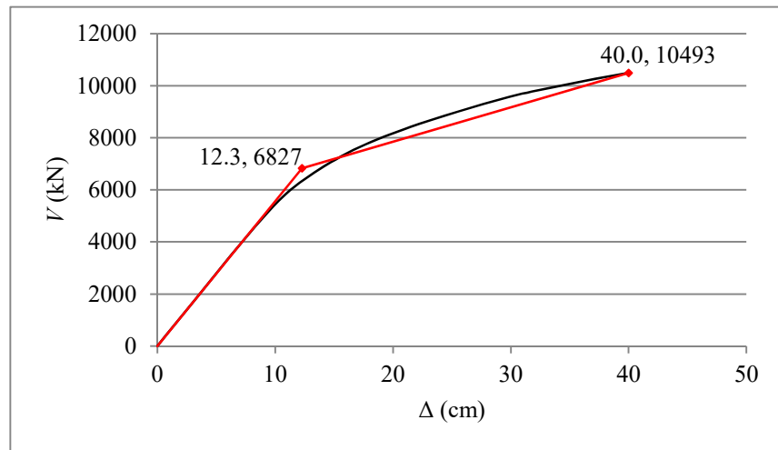
Figure 3.31: Bilinear Pushover curve, Structure 3, direction x, first iteration.
