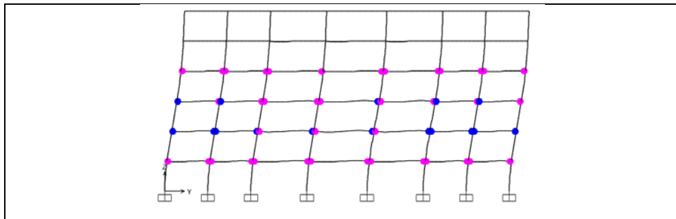
Figure A1.7: Hinge status at performance point, ASCE-41-13, Structure 2, Frame 2.
