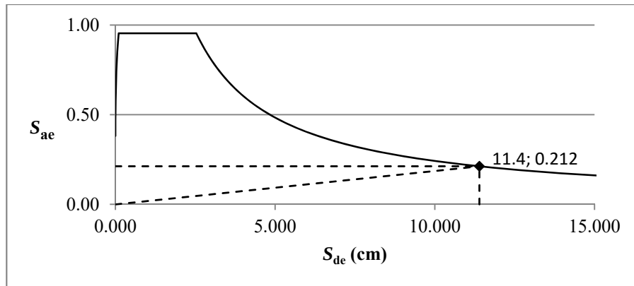
Figure 3.48: Target displacement computation, TBDY-16, Structure 1, direction x.
