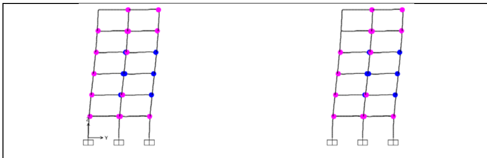
Figure A1.52: Hinge status at performance point, TBDY-16, Structure, 3, Frame 5.
