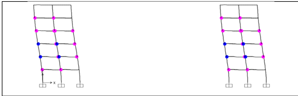
Figure A1.30: Hinge status at performance point, EN 1998-3, Structure 3, Frame E.
