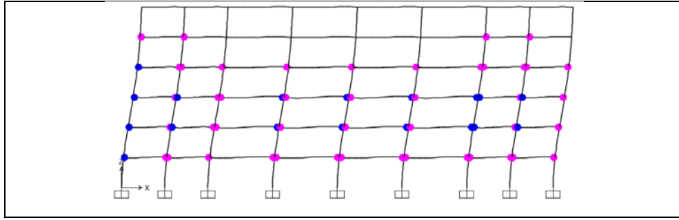
Figure A1.25: Hinge status at performance point, EN 1998-3, Structure 2, Frame B.
