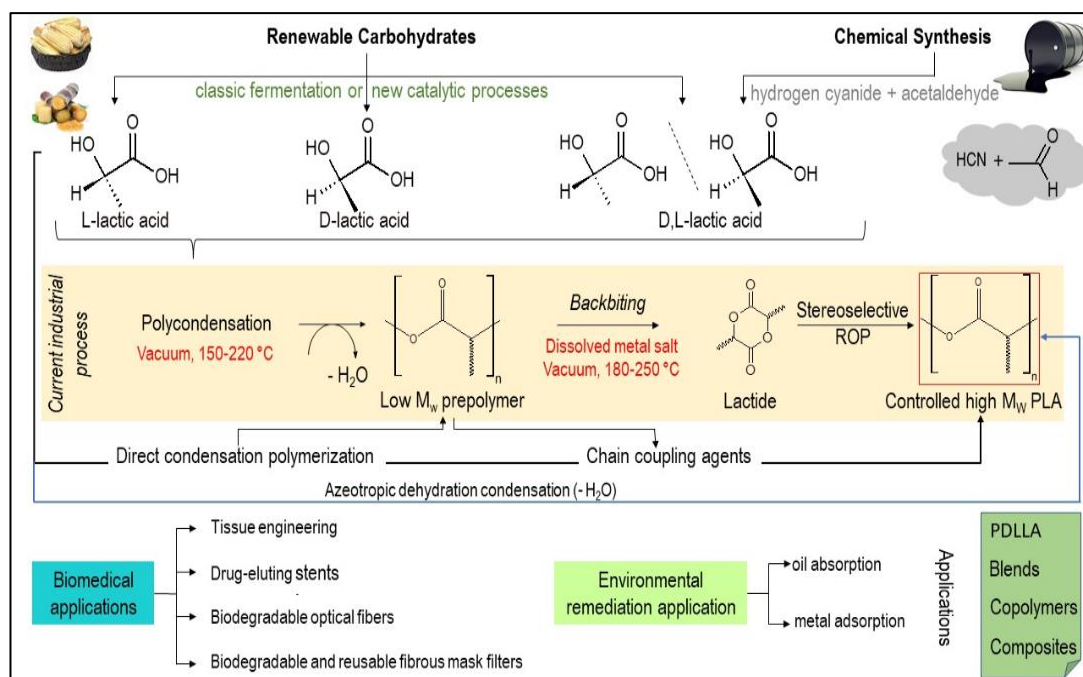
Figure 1.2: Synthesis of PLA [de França et al, 2022].
