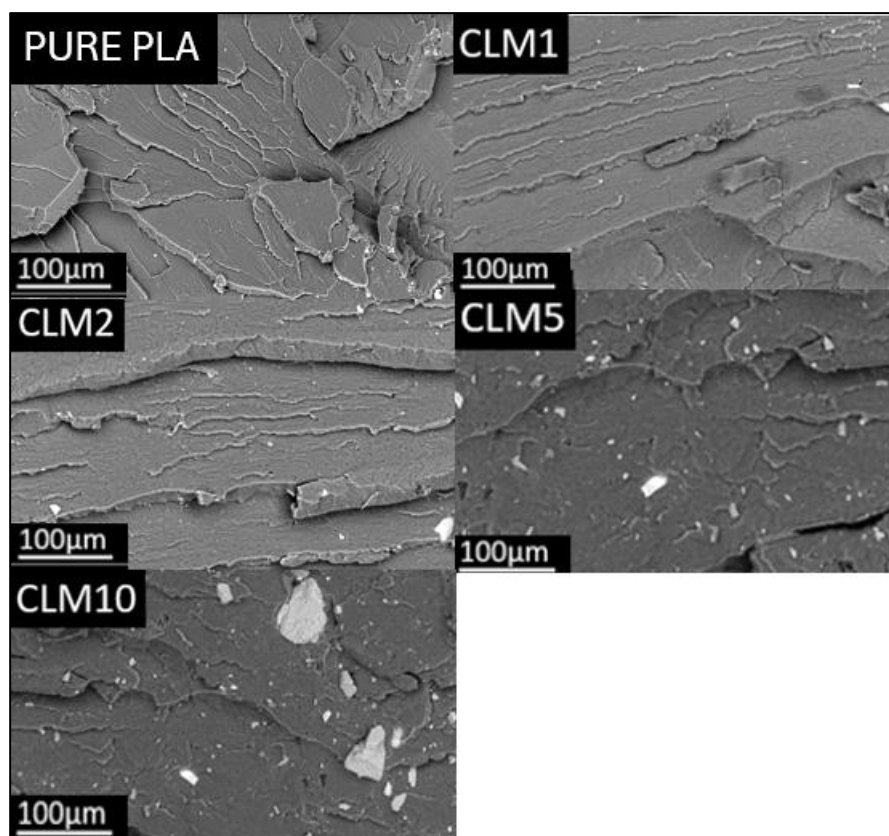
Figure 3.7: SEM images of CLM compounds.
