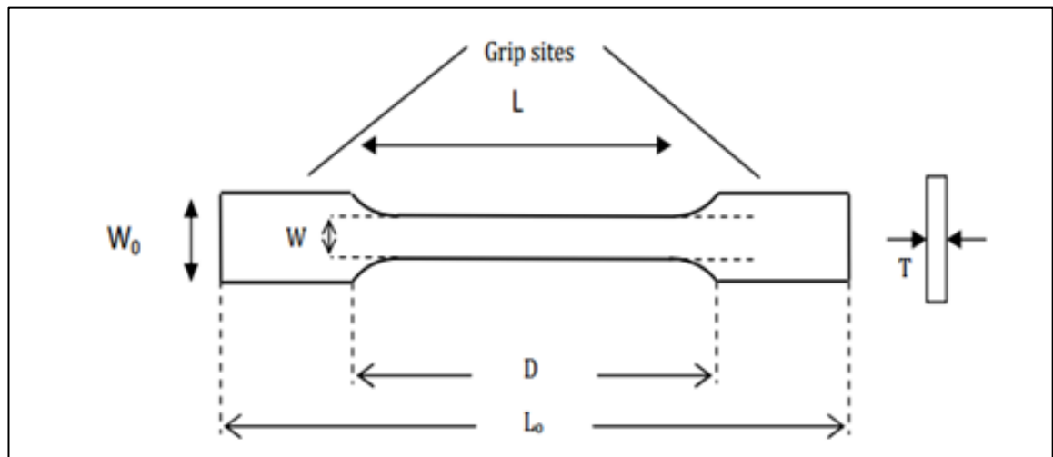
Figure 2.3: Schematic of tensile test specimen.
