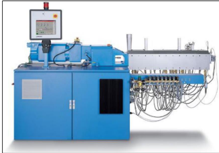
Figure 2.1: Twin-screw extruder.
