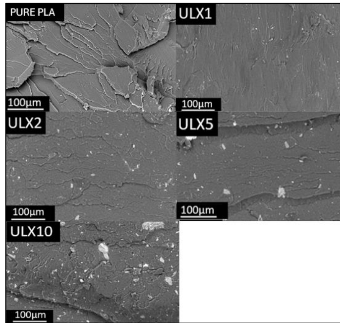
Figure 3.6: SEM images of ULX compounds.
