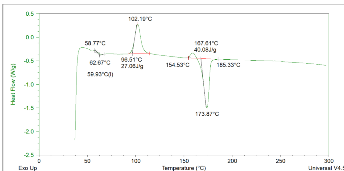
Figure 3.4: 1 st heating curve of pure PLA.
