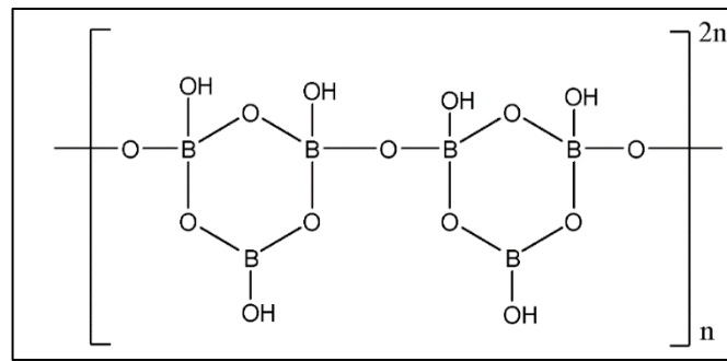
Figure 1.4: Chemical structure of colemanite.
