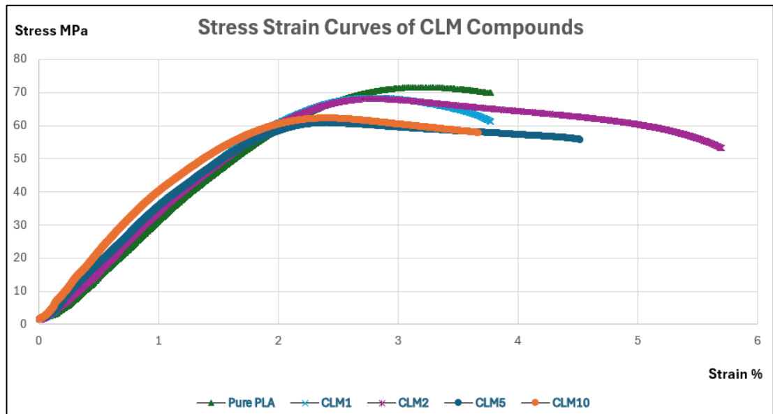
Figure 3.2: Stress Strain Curves of CLM Compounds.
