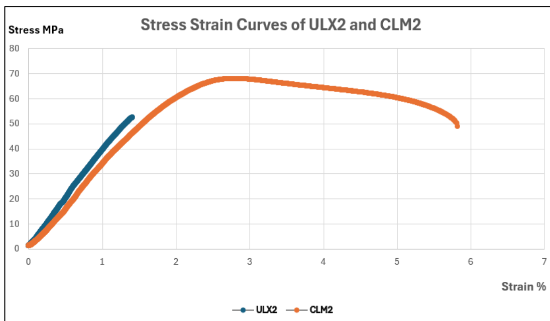
Figure 3.3: Stress Strain Curves of ULX2 and CLM2 Compounds.
