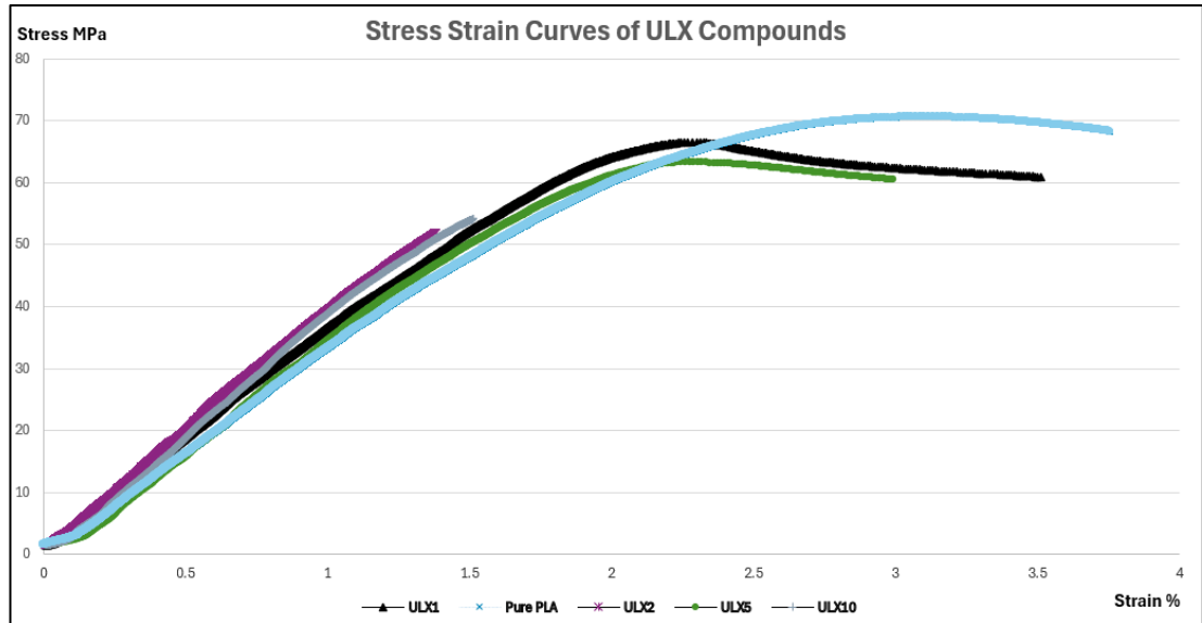
Figure 3.1: Stress Strain Curves of ULX Compounds.
