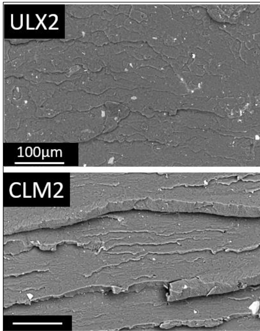
Figure 3.8: SEM Images of ULX2 and CLM2.
