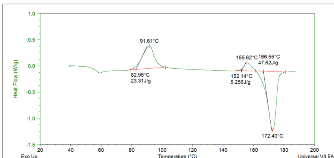
Figure 3.5: 1 st heating curve of ULX2.
