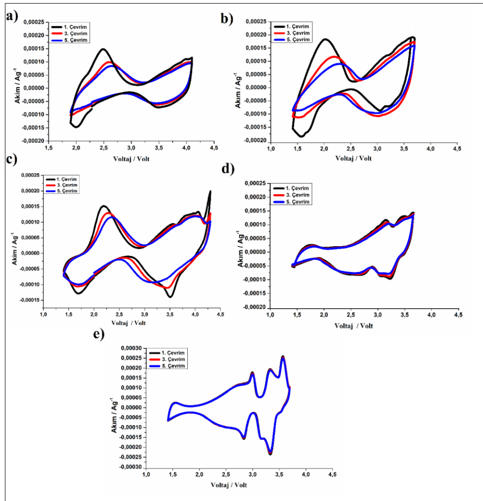
Şekil 4.23: 0.1 \text{ mVs}^{-1} tarama hızında a) \text{Na}_{0.7}\text{Mn}_{0.45}\text{Fe}_{0.45}\text{Co}_{0.1}\text{O}_2 b) \text{Na}_{0.7}\text{Mn}_{0.4}\text{Fe}_{0.4}\text{Co}_{0.2}\text{O}_2 c) \text{Na}_{0.7}\text{Mn}_{0.35}\text{Fe}_{0.35}\text{Co}_{0.3}\text{O}_2 d) \text{Na}_{0.7}\text{Mn}_{0.3}\text{Fe}_{0.3}\text{Co}_{0.4}\text{O}_2 e) \text{Na}_{0.7}\text{Mn}_{0.25}\text{Fe}_{0.25}\text{Co}_{0.5}\text{O}_2 numunelerine ait CV eğrileri.
