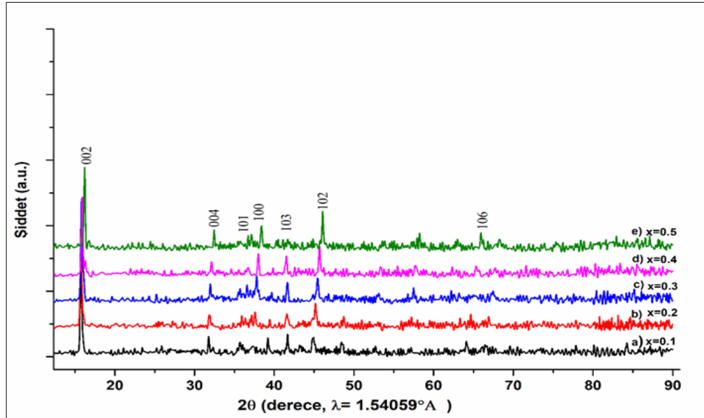
Şekil 4.12: Katı hal yöntemi ile sentezlenen a) \text{Na}_{0.7}\text{Mn}_{0.45}\text{Fe}_{0.45}\text{Co}_{0.1}\text{O}_2 b) \text{Na}_{0.7}\text{Mn}_{0.4}\text{Fe}_{0.4}\text{Co}_{0.2}\text{O}_2 c) \text{Na}_{0.7}\text{Mn}_{0.35}\text{Fe}_{0.35}\text{Co}_{0.3}\text{O}_2 d) \text{Na}_{0.7}\text{Mn}_{0.3}\text{Fe}_{0.3}\text{Co}_{0.4}\text{O}_2 e) \text{Na}_{0.7}\text{Mn}_{0.25}\text{Fe}_{0.25}\text{Co}_{0.5}\text{O}_2 maddelerinin XRD toz desenleri.
