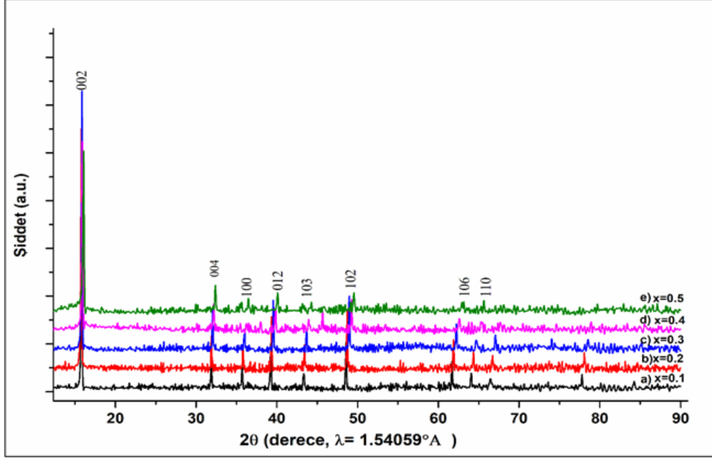
Şekil 4.11: Sol jel yöntemi ile sentezlenen a) \text{Na}_{0.7}\text{Mn}_{0.45}\text{Fe}_{0.45}\text{Co}_{0.1}\text{O}_2 b) \text{Na}_{0.7}\text{Mn}_{0.4}\text{Fe}_{0.4}\text{Co}_{0.2}\text{O}_2 c) \text{Na}_{0.7}\text{Mn}_{0.35}\text{Fe}_{0.35}\text{Co}_{0.3}\text{O}_2 d) \text{Na}_{0.7}\text{Mn}_{0.3}\text{Fe}_{0.3}\text{Co}_{0.4}\text{O}_2 e) \text{Na}_{0.7}\text{Mn}_{0.25}\text{Fe}_{0.25}\text{Co}_{0.5}\text{O}_2 maddelerinin XRD toz desenleri.
