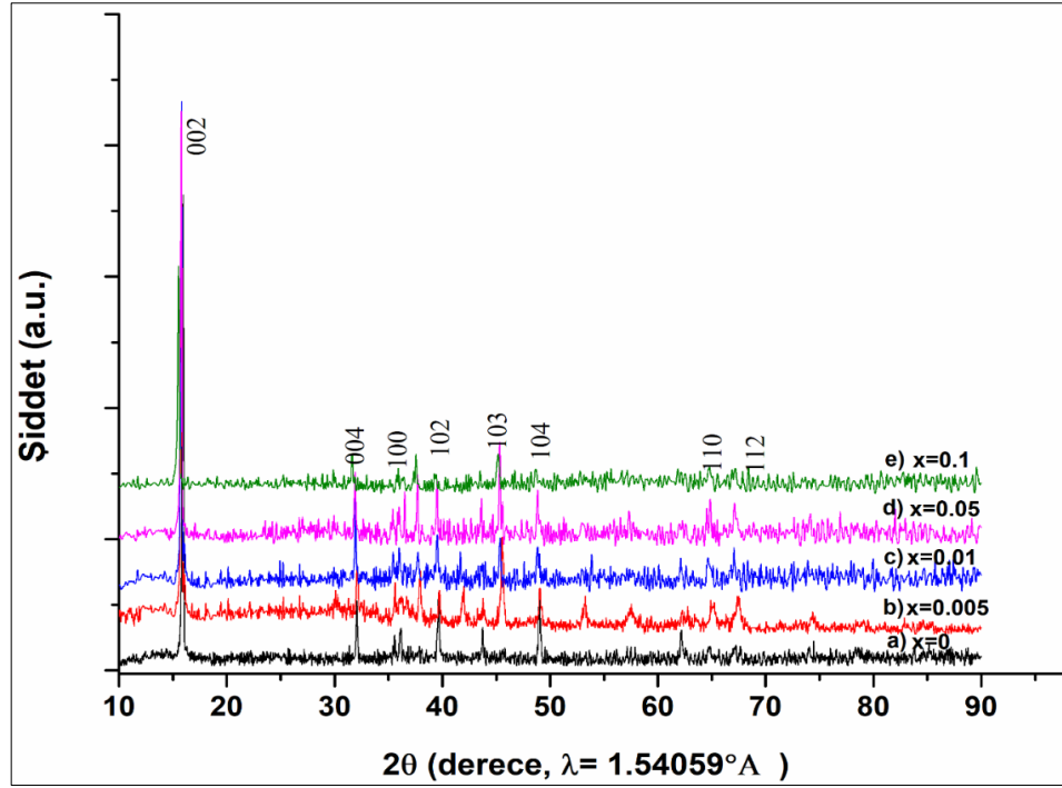
Şekil 4.51: Sol jel yöntemi ile sentezlenen a) \text{Na}_{0.6}\text{Mn}_{0.35}\text{Fe}_{0.35}\text{Co}_{0.3}\text{O}_2 b) \text{K}_{0.005}\text{Na}_{0.595}\text{Mn}_{0.35}\text{Fe}_{0.35}\text{Co}_{0.3}\text{O}_2 c) \text{K}_{0.01}\text{Na}_{0.59}\text{Mn}_{0.35}\text{Fe}_{0.35}\text{Co}_{0.3}\text{O}_2 d) \text{K}_{0.05}\text{Na}_{0.55}\text{Mn}_{0.35}\text{Fe}_{0.35}\text{Co}_{0.3}\text{O}_2 e) \text{K}_{0.1}\text{Na}_{0.5}\text{Mn}_{0.35}\text{Fe}_{0.35}\text{Co}_{0.3}\text{O}_2 maddelerinin XRD toz desenleri.
