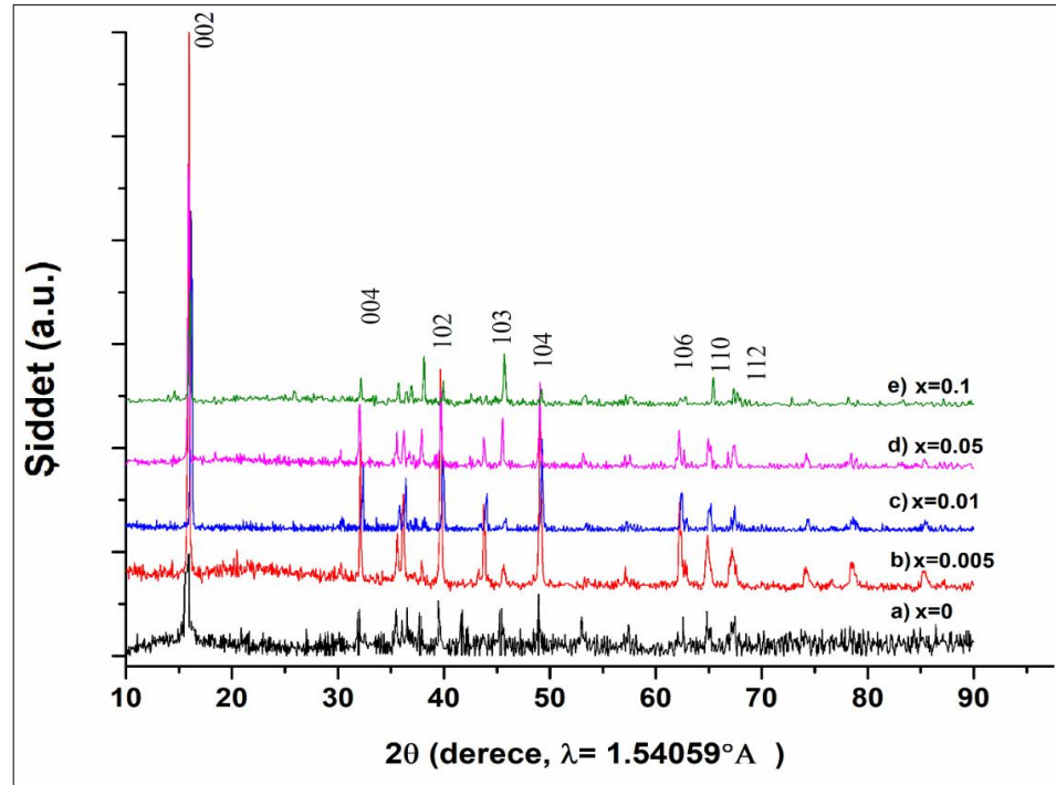
Şekil 4.52: Katı hal yöntemi ile sentezlenen a) \text{Na}_{0.6}\text{Mn}_{0.35}\text{Fe}_{0.35}\text{Co}_{0.3}\text{O}_2 b) \text{K}_{0.005}\text{Na}_{0.595}\text{Mn}_{0.35}\text{Fe}_{0.35}\text{Co}_{0.3}\text{O}_2 c) \text{K}_{0.01}\text{Na}_{0.59}\text{Mn}_{0.35}\text{Fe}_{0.35}\text{Co}_{0.3}\text{O}_2 d) \text{K}_{0.05}\text{Na}_{0.55}\text{Mn}_{0.35}\text{Fe}_{0.35}\text{Co}_{0.3}\text{O}_2 e) \text{K}_{0.1}\text{Na}_{0.5}\text{Mn}_{0.35}\text{Fe}_{0.35}\text{Co}_{0.3}\text{O}_2 maddelerinin XRD toz desenleri.
