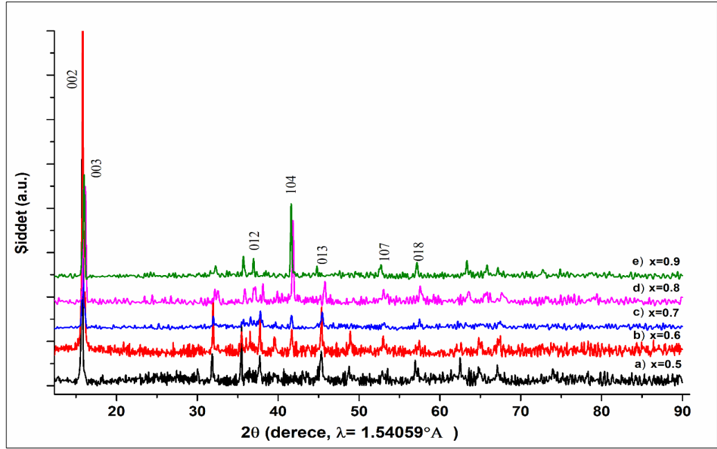
Şekil 4.30: Katı hal yöntemi ile sentezlenen a) \text{Na}_{0.5}\text{Mn}_{0.35}\text{Fe}_{0.35}\text{Co}_{0.3}\text{O}_2 b) \text{Na}_{0.6}\text{Mn}_{0.35}\text{Fe}_{0.35}\text{Co}_{0.3}\text{O}_2 c) \text{Na}_{0.7}\text{Mn}_{0.35}\text{Fe}_{0.35}\text{Co}_{0.3}\text{O}_2 d) \text{Na}_{0.8}\text{Mn}_{0.35}\text{Fe}_{0.35}\text{Co}_{0.3}\text{O}_2 e) \text{Na}_{0.9}\text{Mn}_{0.35}\text{Fe}_{0.35}\text{Co}_{0.3}\text{O}_2 maddelerinin XRD toz desenleri.
