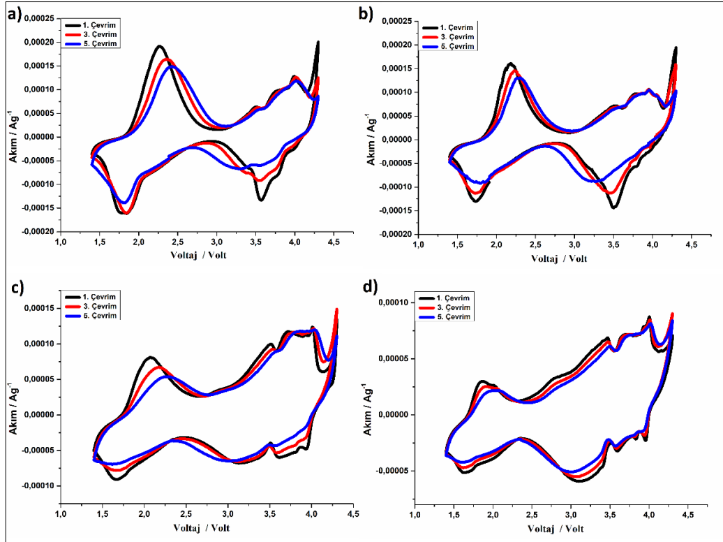
Şekil 4.39: 0.1 mVs -1 tarama hızında a) \text{Na}_{0.5}\text{Mn}_{0.35}\text{Fe}_{0.35}\text{Co}_{0.3}\text{O}_2 b) \text{Na}_{0.6}\text{Mn}_{0.35}\text{Fe}_{0.35}\text{Co}_{0.3}\text{O}_2 c) \text{Na}_{0.8}\text{Mn}_{0.35}\text{Fe}_{0.35}\text{Co}_{0.3}\text{O}_2 d) \text{Na}_{0.9}\text{Mn}_{0.35}\text{Fe}_{0.35}\text{Co}_{0.3}\text{O}_2 numunelerine ait CV eğrileri.
