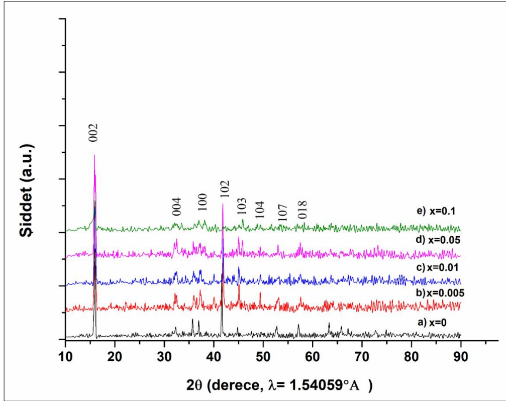
Şekil 4.54: Katı hal yöntemi ile sentezlenen a) \text{Na}_{0.9}\text{Mn}_{0.35}\text{Fe}_{0.35}\text{Co}_{0.3}\text{O}_2 b) \text{K}_{0.005}\text{Na}_{0.895}\text{Mn}_{0.35}\text{Fe}_{0.35}\text{Co}_{0.3}\text{O}_2 c) \text{K}_{0.01}\text{Na}_{0.89}\text{Mn}_{0.35}\text{Fe}_{0.35}\text{Co}_{0.3}\text{O}_2 d) \text{K}_{0.05}\text{Na}_{0.85}\text{Mn}_{0.35}\text{Fe}_{0.35}\text{Co}_{0.3}\text{O}_2 e) \text{K}_{0.1}\text{Na}_{0.8}\text{Mn}_{0.35}\text{Fe}_{0.35}\text{Co}_{0.3}\text{O}_2 maddelerinin XRD toz desenleri.
