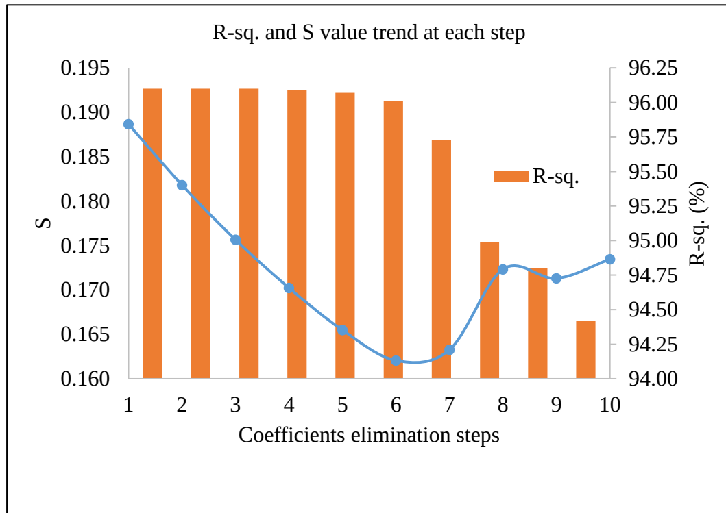
Figure 5.4: Elimination steps in cubic equation model with extra 4 cases.
