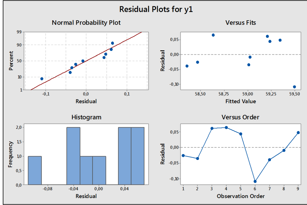
Figure 5.14: Residual plots for quadratic analysis for constant base angle 20^\circ .
