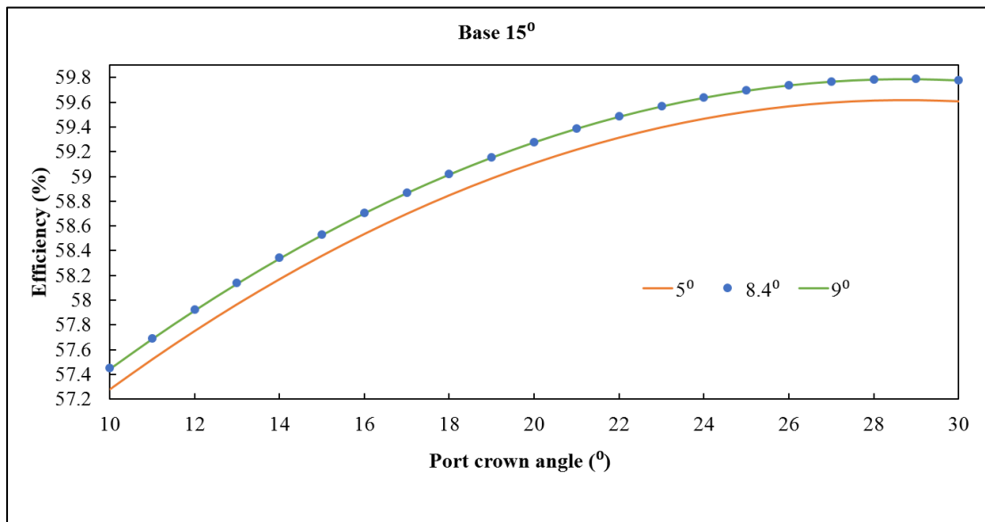
Figure 5.10: Effects of port crown angle and burner angle on the energy efficiency of the furnace for constant port base angle, x_3=15^\circ .
