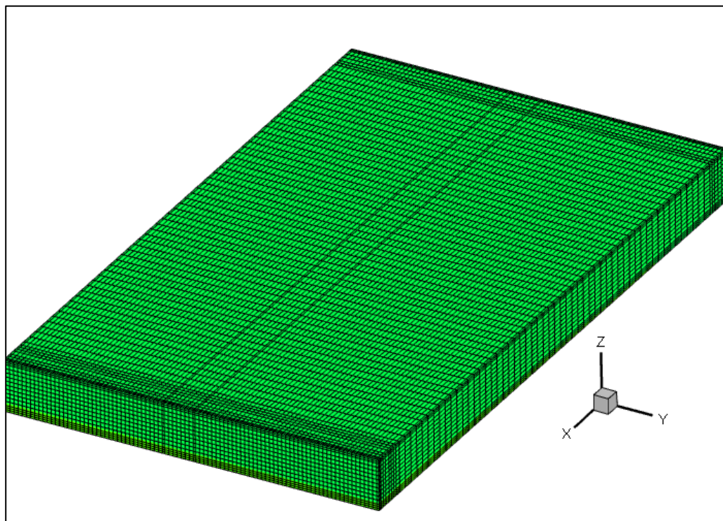
Figure 4.5: Grid structure of the glass bath solution domain.
