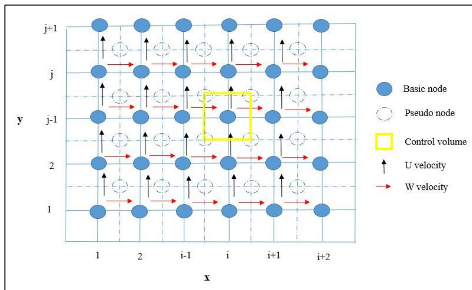
Figure C1.1: Grid representation of the solution domain.
