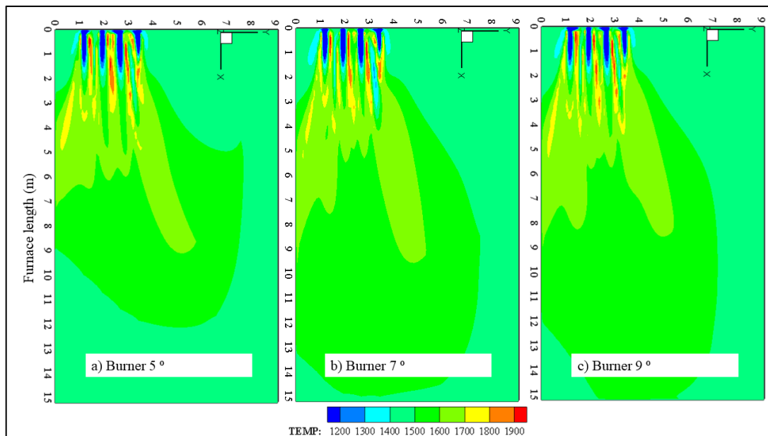
Figure 5.15: Top view of combustion space at burner axis for the angle of 5^\circ , 7^\circ , and 9^\circ .
