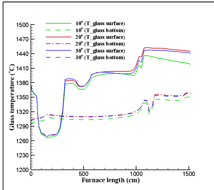
Figure 5.22: Surface and bottom temperatures of glass for the crown angle of 10^\circ , 20^\circ , and 30^\circ .
