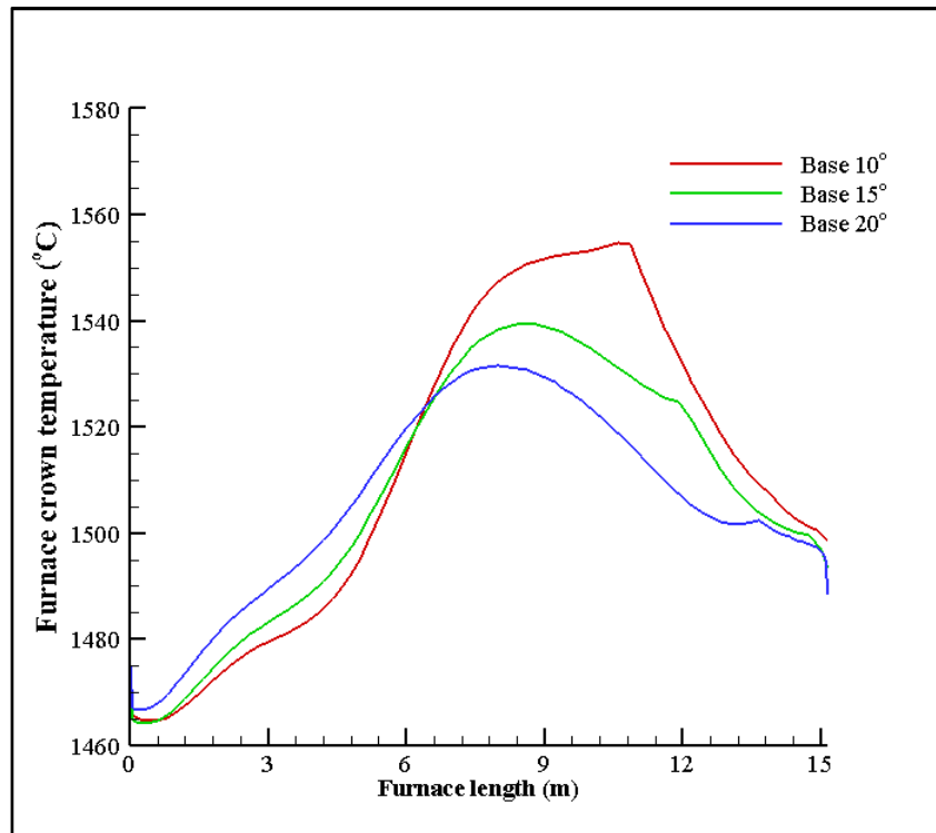
Figure 5.25: Combustion space temperatures at the roof of the furnace along the length for the port base angle of 10^\circ , 15^\circ , and 20^\circ .
