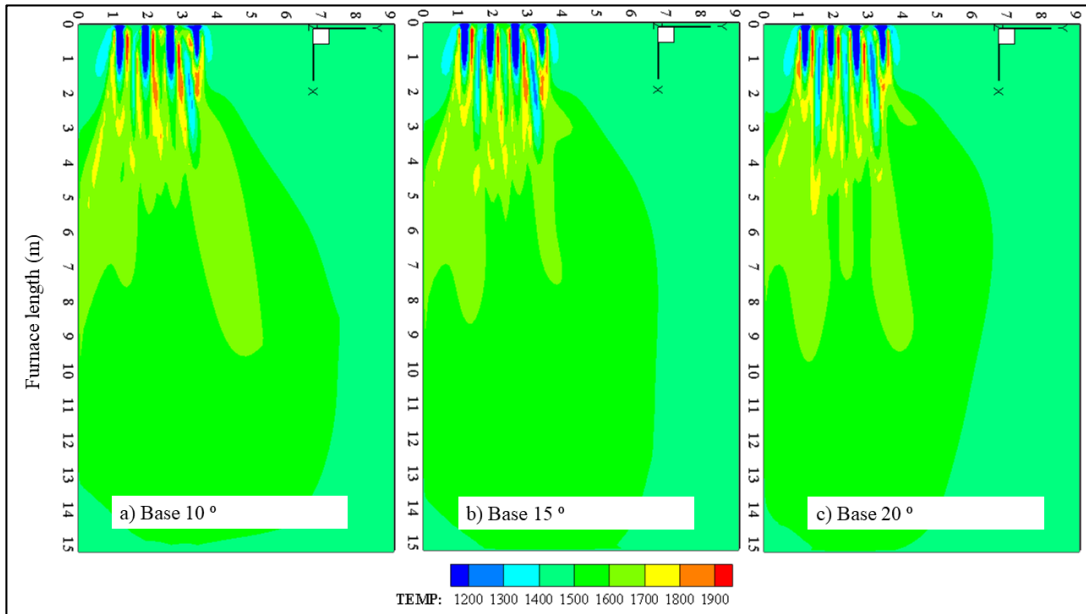
Figure 5.23: Top view of combustion space at burner axis for the port base angle of 10^\circ , 15^\circ , and 20^\circ .
