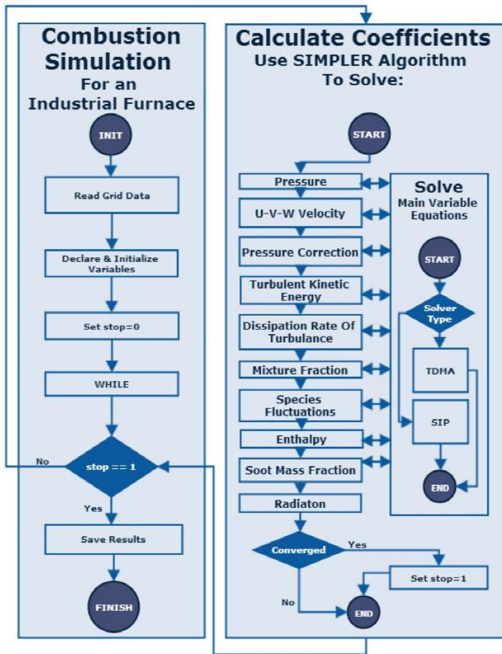
Figure 3.2: High-level structure of the Glass Furnace Simulation program.
