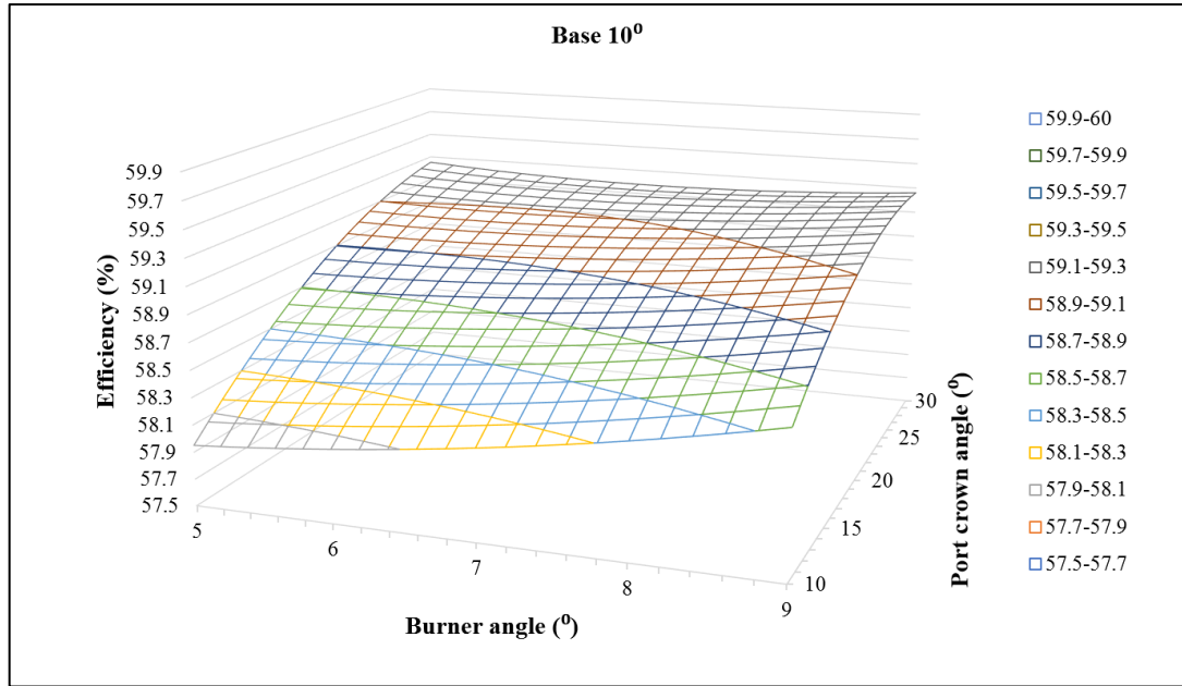
Figure 5.6: Energy efficiency diagram as a function of burner angle and port crown angle for constant port base angle, x_3=10^\circ .
