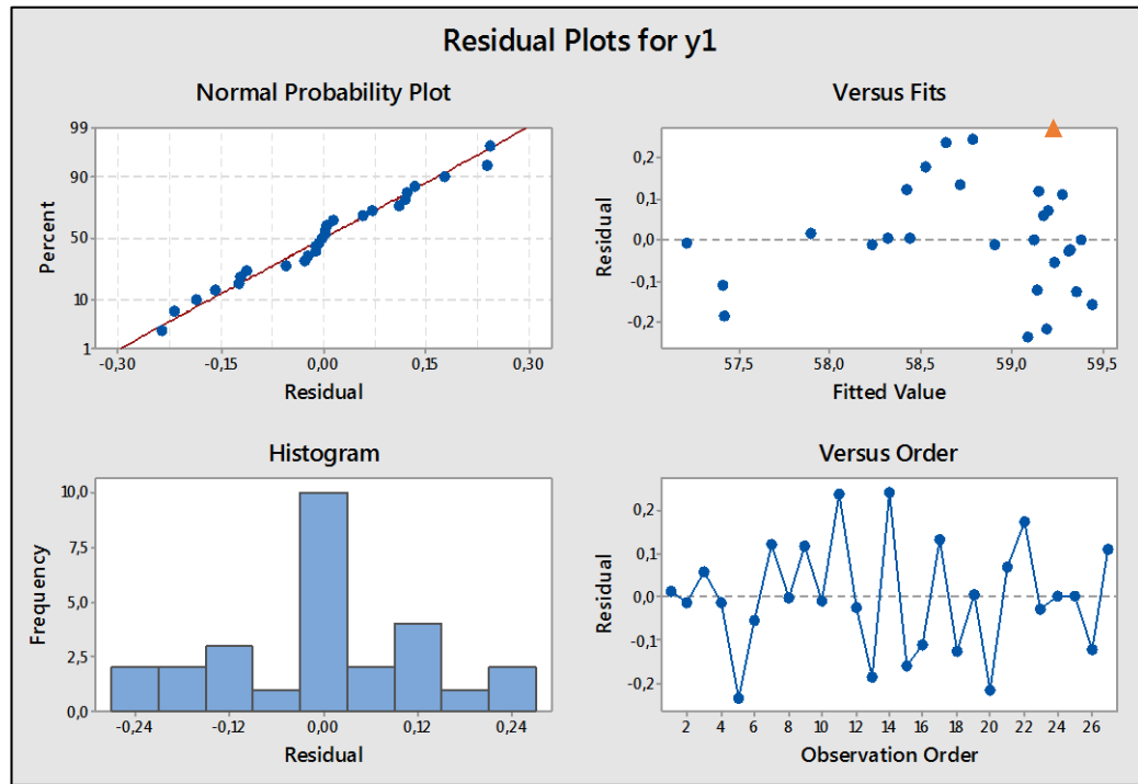
Figure 5.2: Residual plots for the cubic analysis of 27 cases with an improved model.
