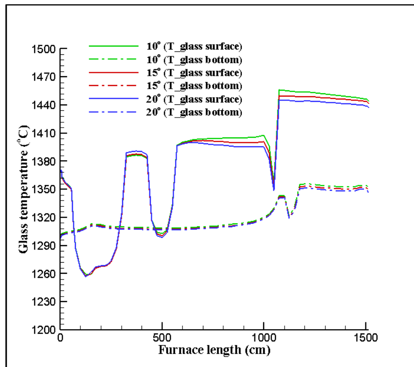
Figure 5.26: Surface and bottom temperatures of glass for the base angle of 10^\circ , 15^\circ , and 20^\circ .
