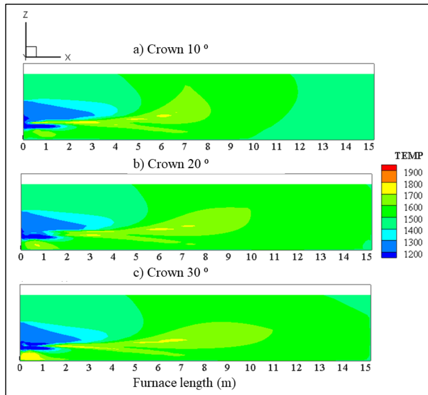
Figure 5.20: Side view of combustion space at burner axis for the port crown angle of 10°, 20°, and 30°.
