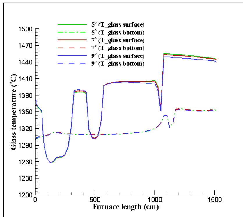
Figure 5.18: Surface and bottom temperatures of glass for the burner angle of 5°, 7°, and 9°.
