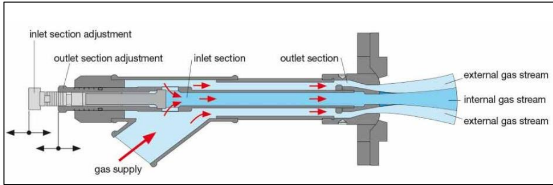
Figure 2.5: A typical pipe-in-pipe burner for glass furnace.
