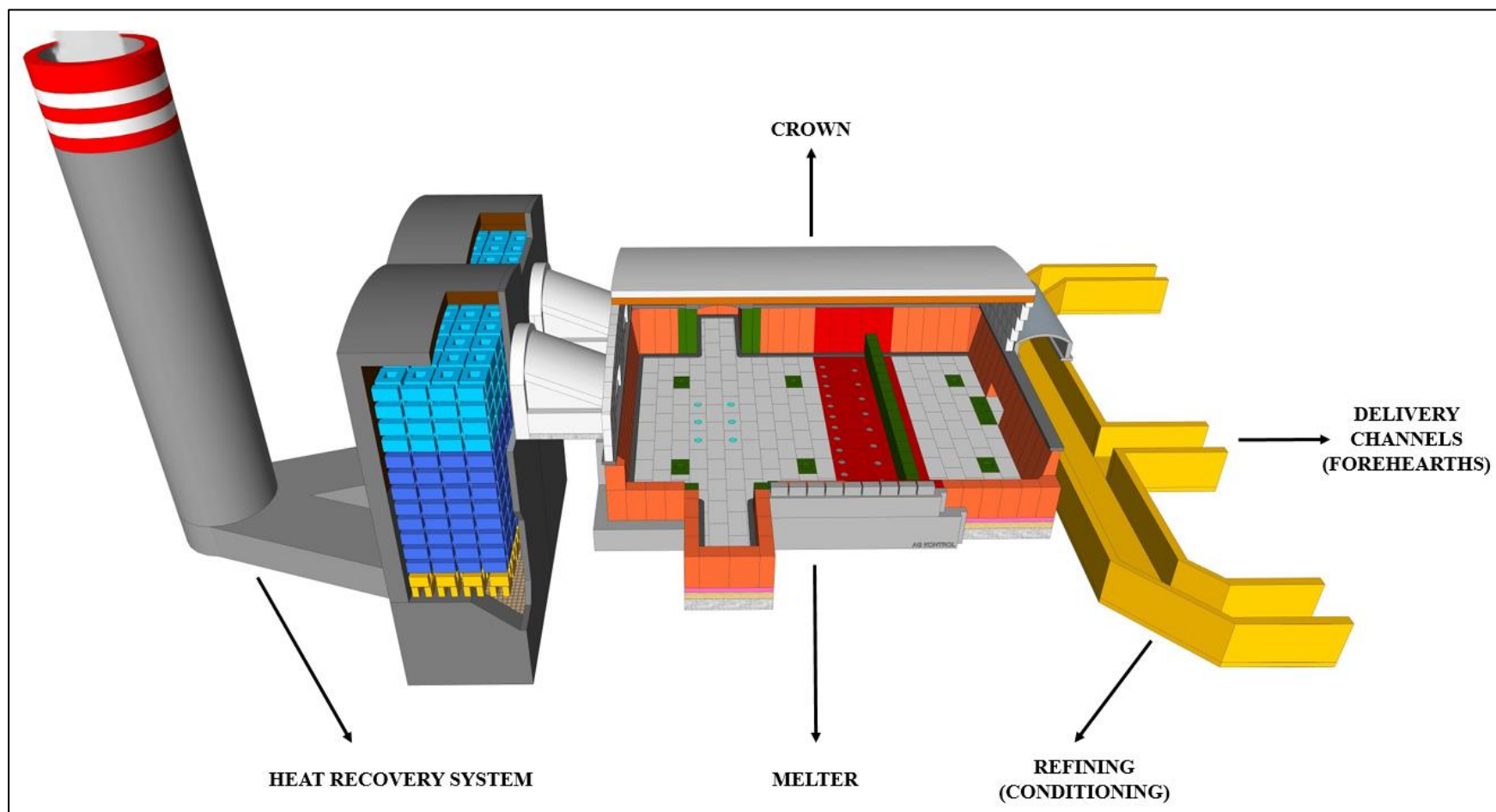
Figure 2.3: Schematic of a typical end-fired container glass furnace.
