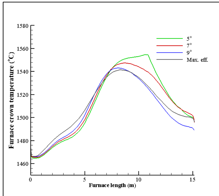
Figure 5.17: Combustion space temperatures at the roof of the furnace along the length for the burner angle of 5°, 7°, and 9°.
