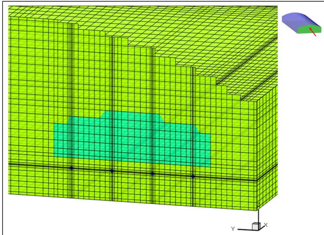
Figure 4.4: Finer grid structure around the burners and ports.
