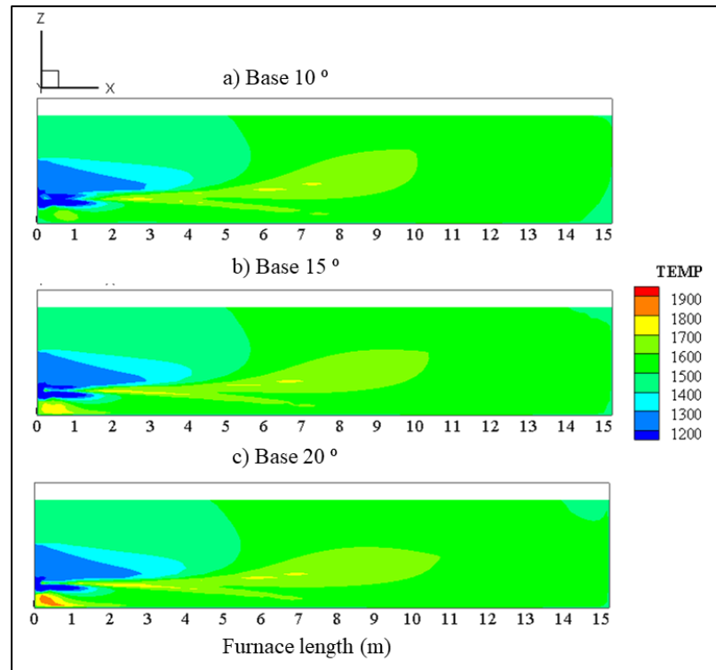
Figure 5.24: Side view of combustion space at burner axis for the port base angle of 10^\circ , 15^\circ , and 20^\circ .
