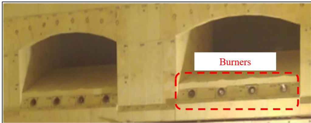
Figure 2.6: Inlet and outlet ports of a furnace.
