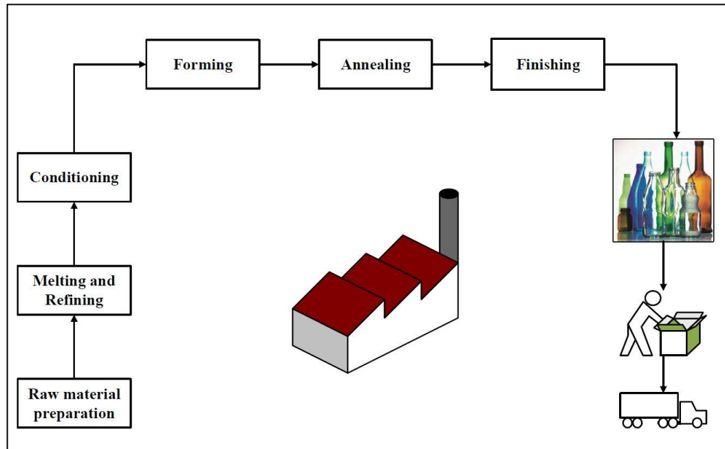
Figure 2.1: The flow diagram of a typical container glass production.
