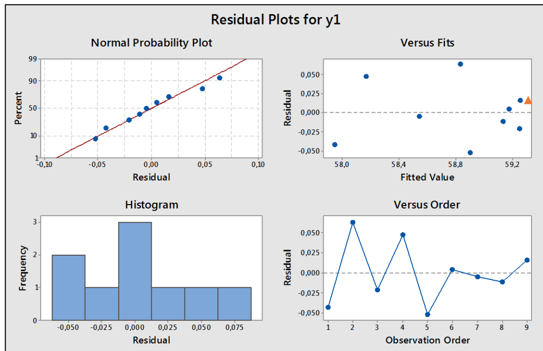
Figure 5.8: Residual plots for quadratic analysis for constant base angle 10^\circ .
