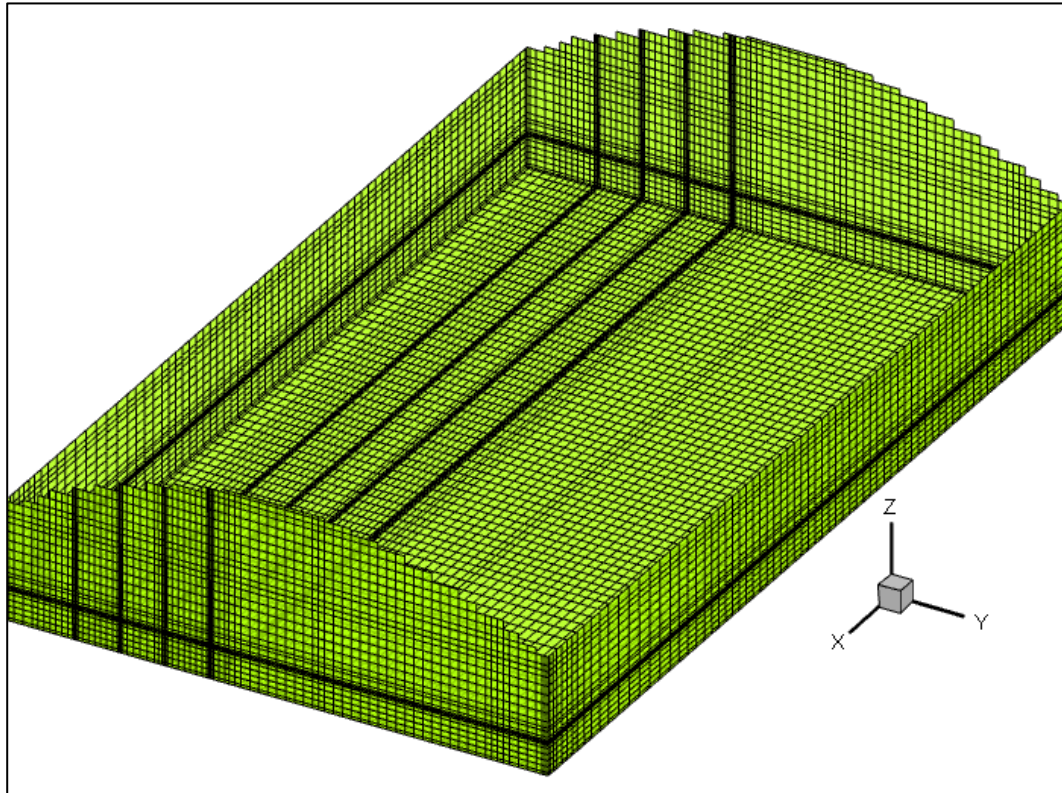
Figure 4.3: Grid structure of the combustion space solution domain.
