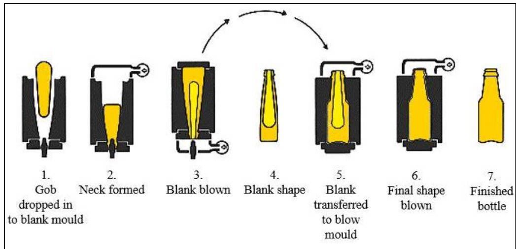
Figure 2.4: Schematic of the glass forming process.
