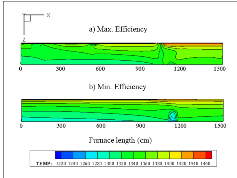
Figure 5.29: The temperatures along the depth of the glass for the minimum and the maximum energy efficient cases.
