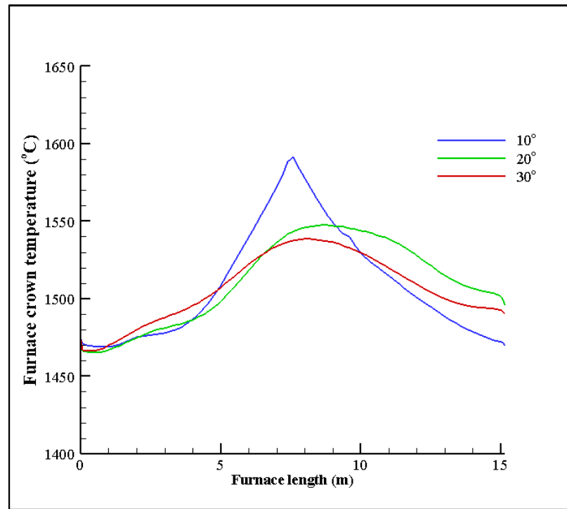
Figure 5.21: Combustion space temperatures at the roof of the furnace along the length for the crown angle of 10^\circ , 20^\circ , and 30^\circ .
