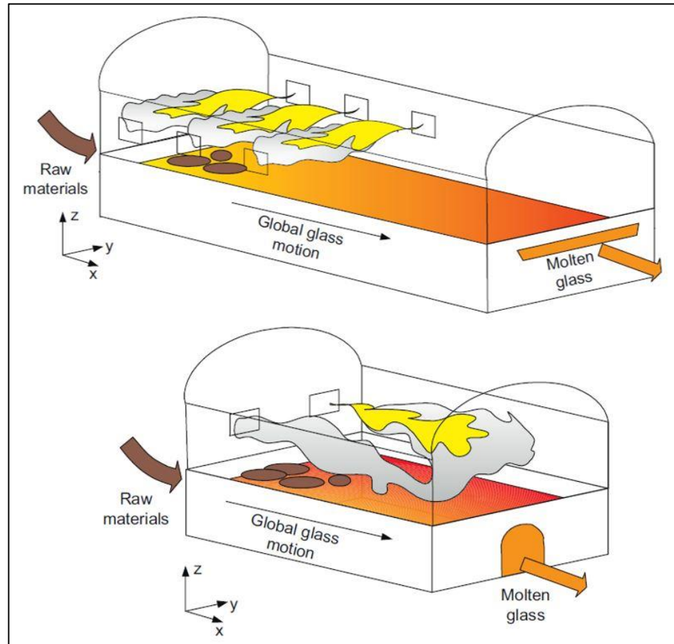
Figure 2.2: Two furnace types a) Cross-fired furnace b) End-fired furnace.
