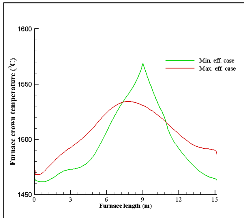
Figure 5.27: Combustion space temperatures at the roof of the furnace along the length for the minimum and maximum efficient cases 0 .
