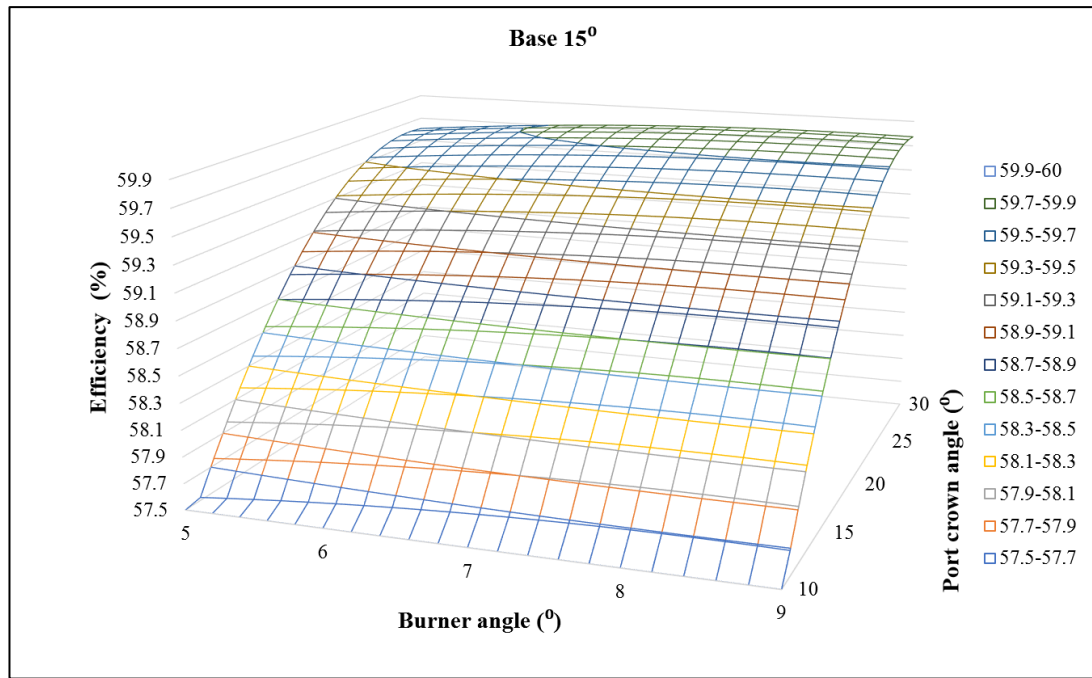
Figure 5.9: Energy efficiency diagram as a function of burner angle and port crown angle for constant port base angle, x_3=15^\circ .
