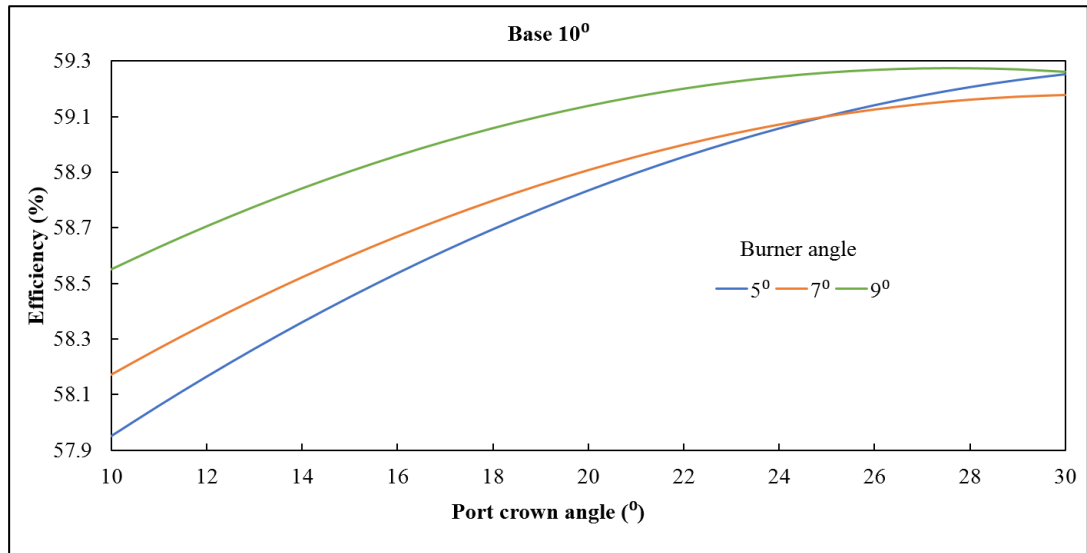
Figure 5.7: Effects of port crown angle and burner angle on the energy efficiency of the furnace for constant port base angle, x_3=10^\circ .
