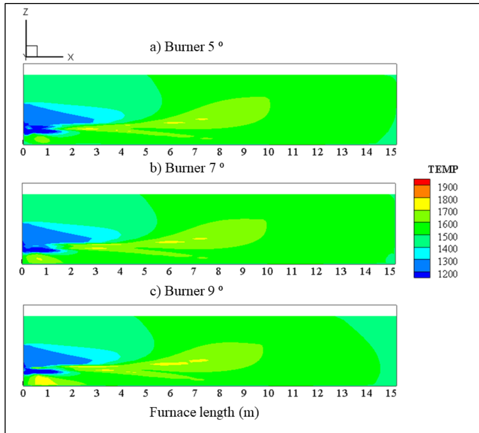
Figure 5.16: Side view of combustion space at burner axis for the burner angle of 5°, 7°, and 9°.
