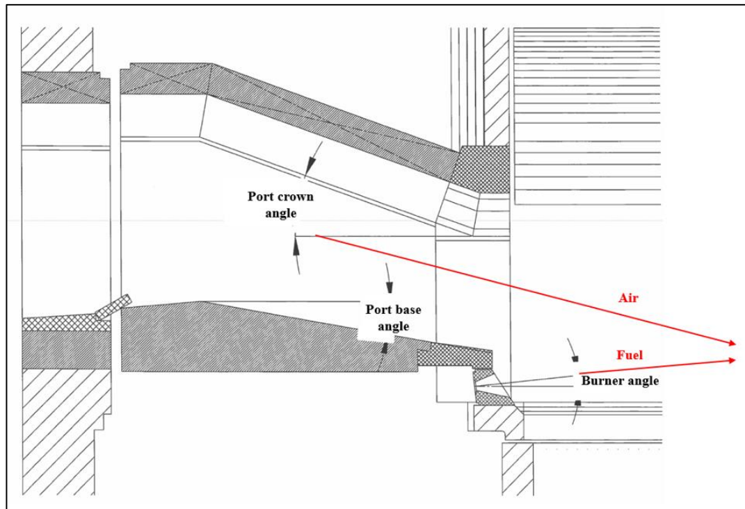
Figure 4.1: The geometrical configuration of port and burner.
