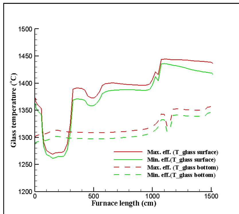
Figure 5.28: Surface and bottom temperatures of glass for the minimum and maximum efficient cases.
