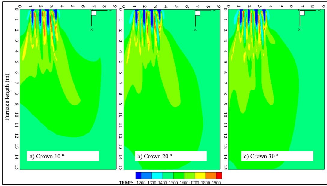
Figure 5.19: Top view of combustion space at burner axis for the port crown angle of 10^\circ , 20^\circ , and 30^\circ .
