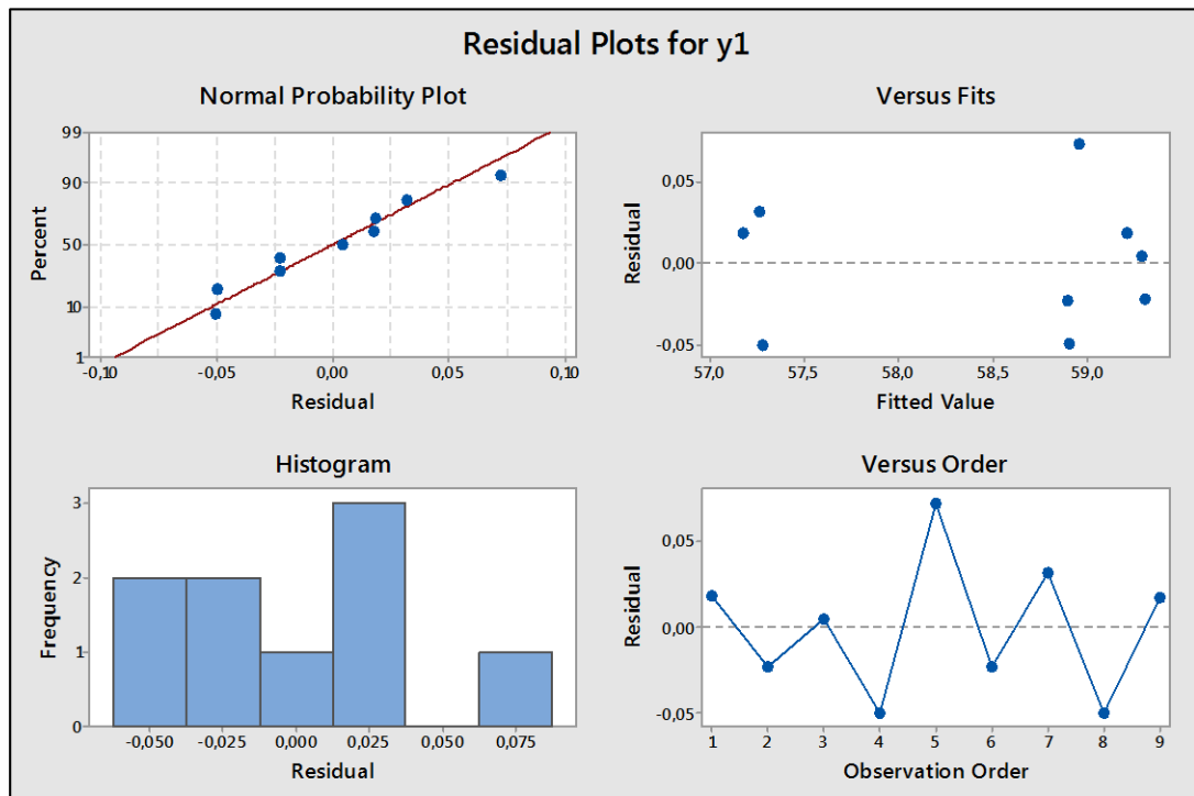
Figure 5.11: Residual plots for quadratic analysis for constant base angle 15^{\circ} .
