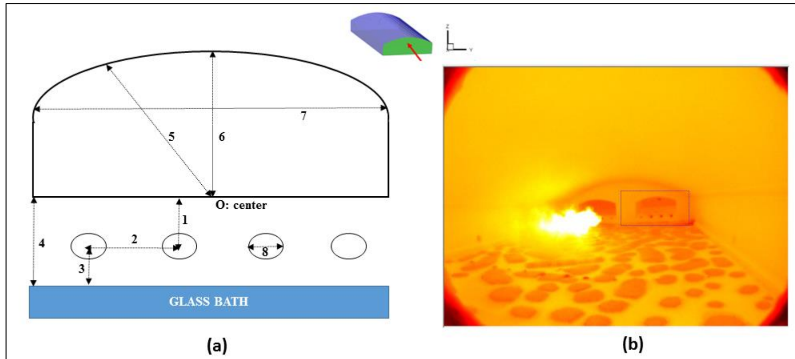
Figure 4.2: a) Representation of combustion space parameters related to ports and burners b) The combustion atmosphere of a real industrial furnace.
