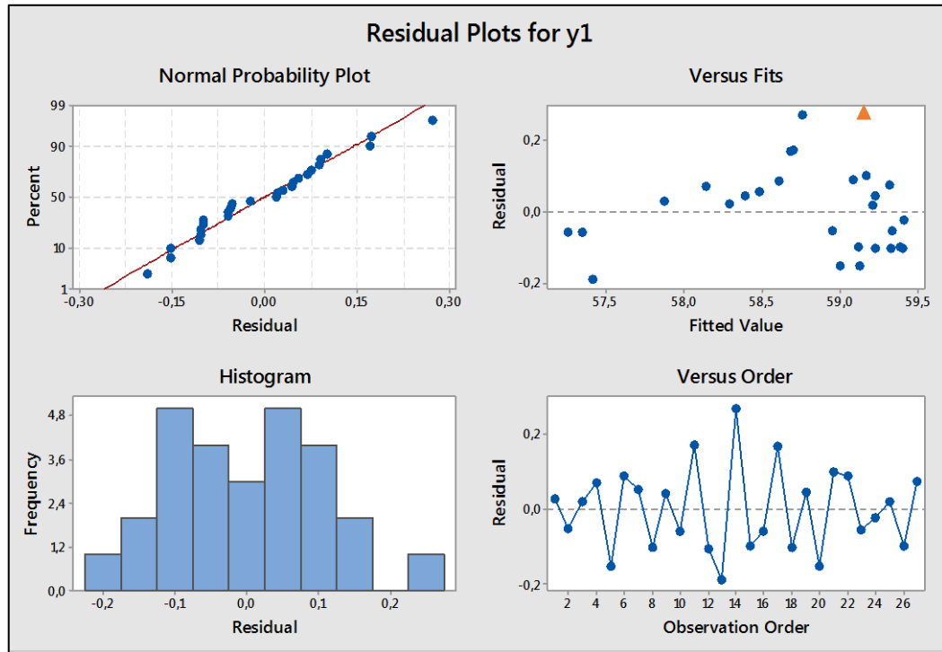
Figure 5.1: Residual plots for the cubic analysis of 27 cases.
