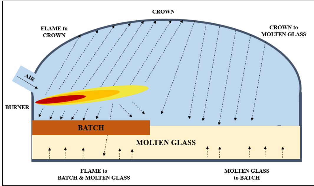
Figure 2.7: The representation of heat transfer mechanisms in glass furnaces.
