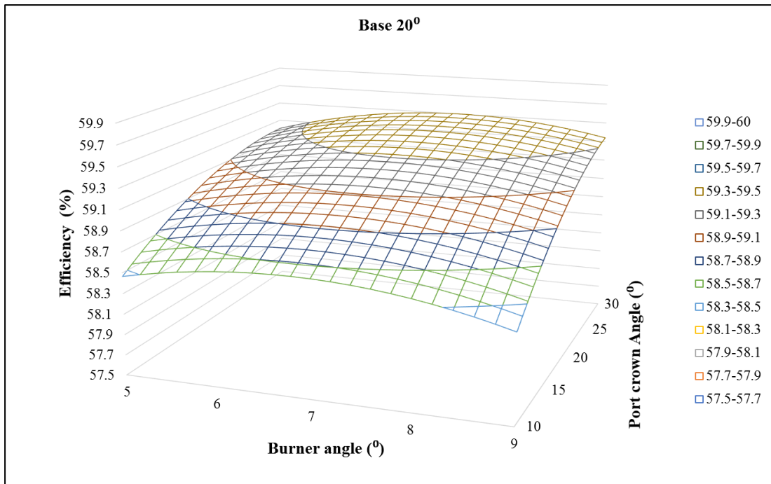
Figure 5.12: Energy efficiency diagram as a function of burner angle and port crown angle for constant port base angle, x_3=20^\circ .
