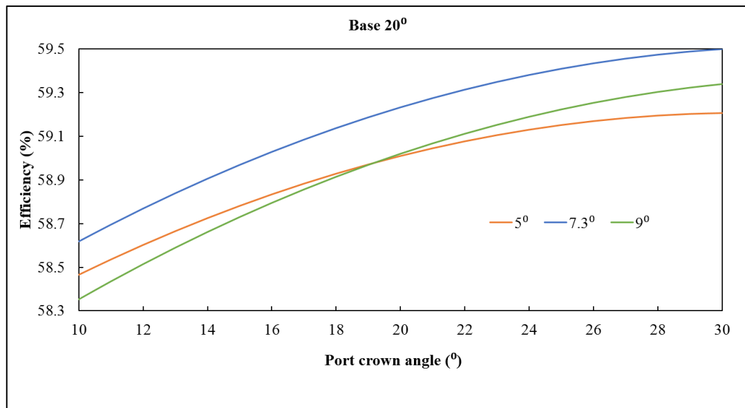
Figure 5.13: Effects of port crown angle and burner angle on the energy efficiency of the furnace for constant port base angle, x_3=20^\circ .
