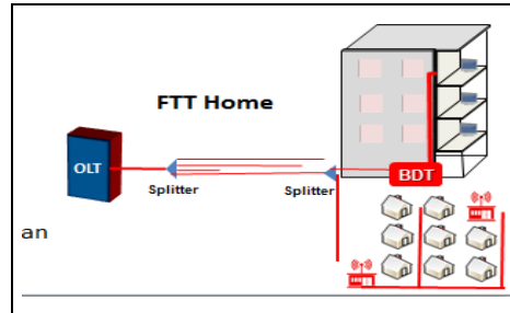
Şekil 4.3: Fiber-to-the-Home
