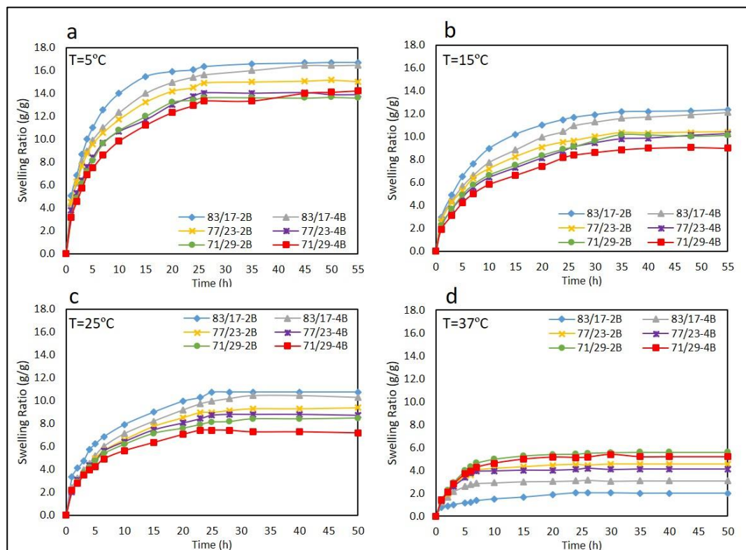
Figure A1.9: Swelling ratio of conventional hydrogels at 5°C (a), 15°C (b), 25°C (c) and 37°C (d) in pH = 5.0.
