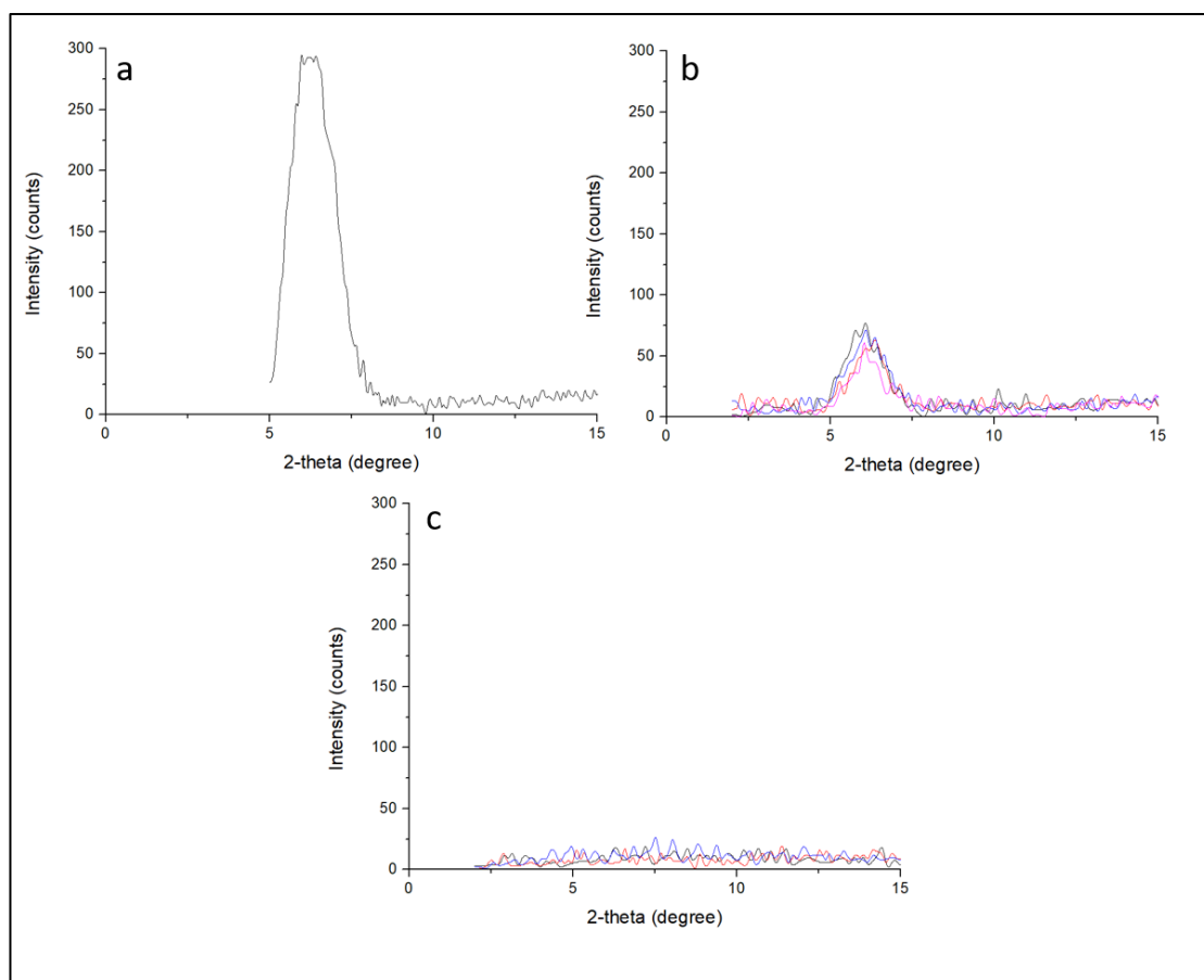
Figure 3.7: XRD profiles for (a) nanoclay, (b) nanocomposite hydrogels and (c) conventional hydrogels.
