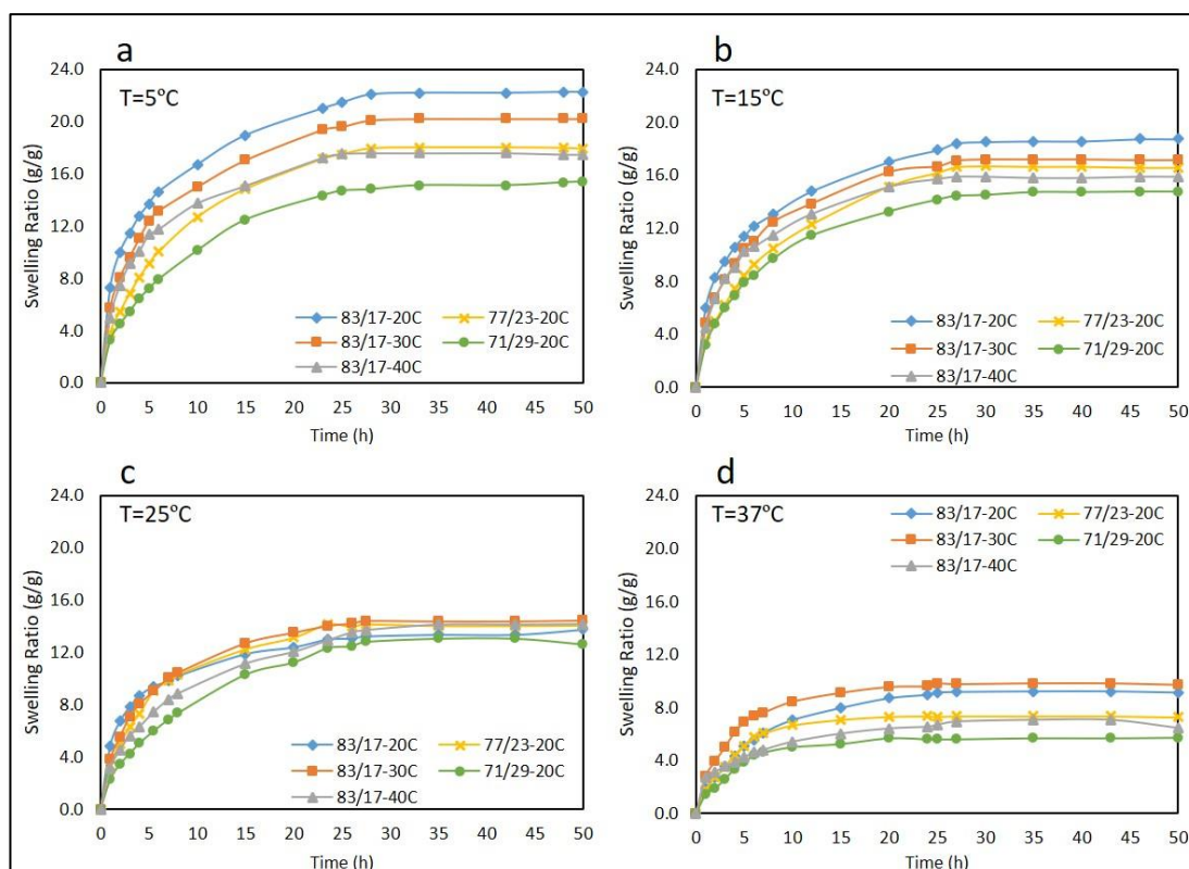
Figure A1.2: Swelling ratio of nanocomposite hydrogels at 5°C (a), 15°C (b), 25 °C (c) and 37°C (d) in pH = 3.0.
