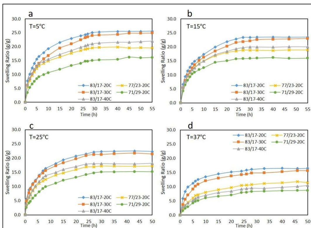
Figure A1.5: Swelling ratio of nanocomposite hydrogels at 5°C (a), 15°C (b), 25 °C (c) and 37°C (d) in pH = 8.0.
