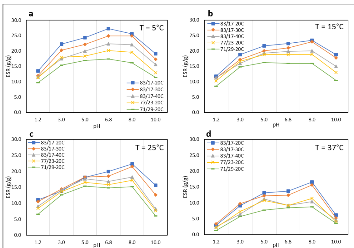
Figure 3.8: The ESR of nanocomposite hydrogels as a function of pH at (a) 5 °C, (b) 15 °C, (c) 25 °C and (d) 37°C.
