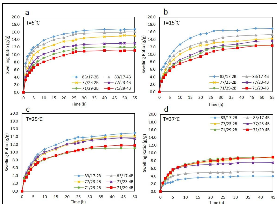
Figure A1.11: Swelling ratio of conventional hydrogels at 5°C (a), 15°C (b), 25°C (c) and 37°C (d) in pH = 8.0.
