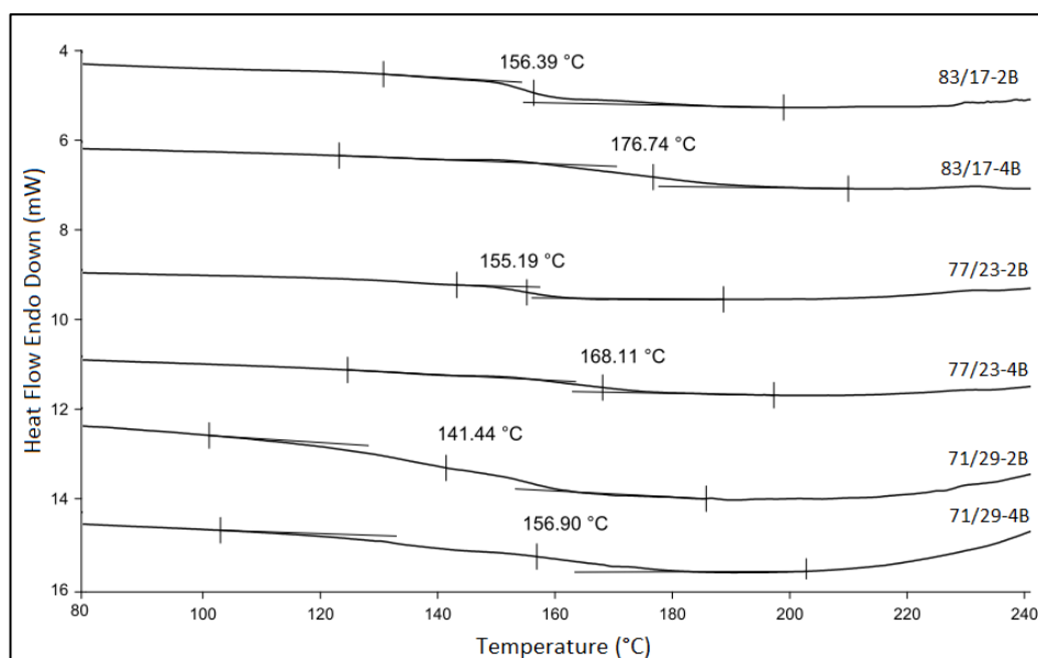
Figure 3.5: DSC thermograms of dried conventional hydrogels.
