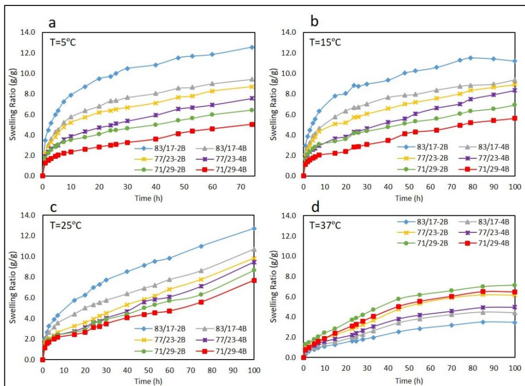
Figure A1.12: Swelling ratio of conventional hydrogels at 5°C (a), 15°C (b), 25 °C (c) and 37°C (d) in pH = 10.0.
