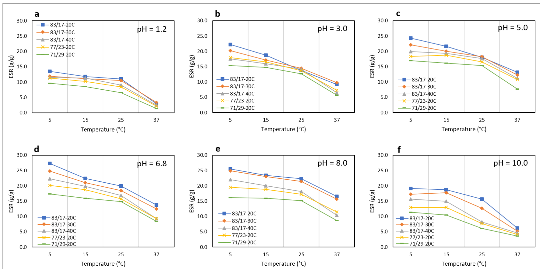
Figure 3.10: The ESR of nanocomposite hydrogels as a function of temperature in the pH of (a) 1.2, (b) 3.0, (c) 5.0, (d) 6.8, (e) 8.0 and (f) 10.0.
