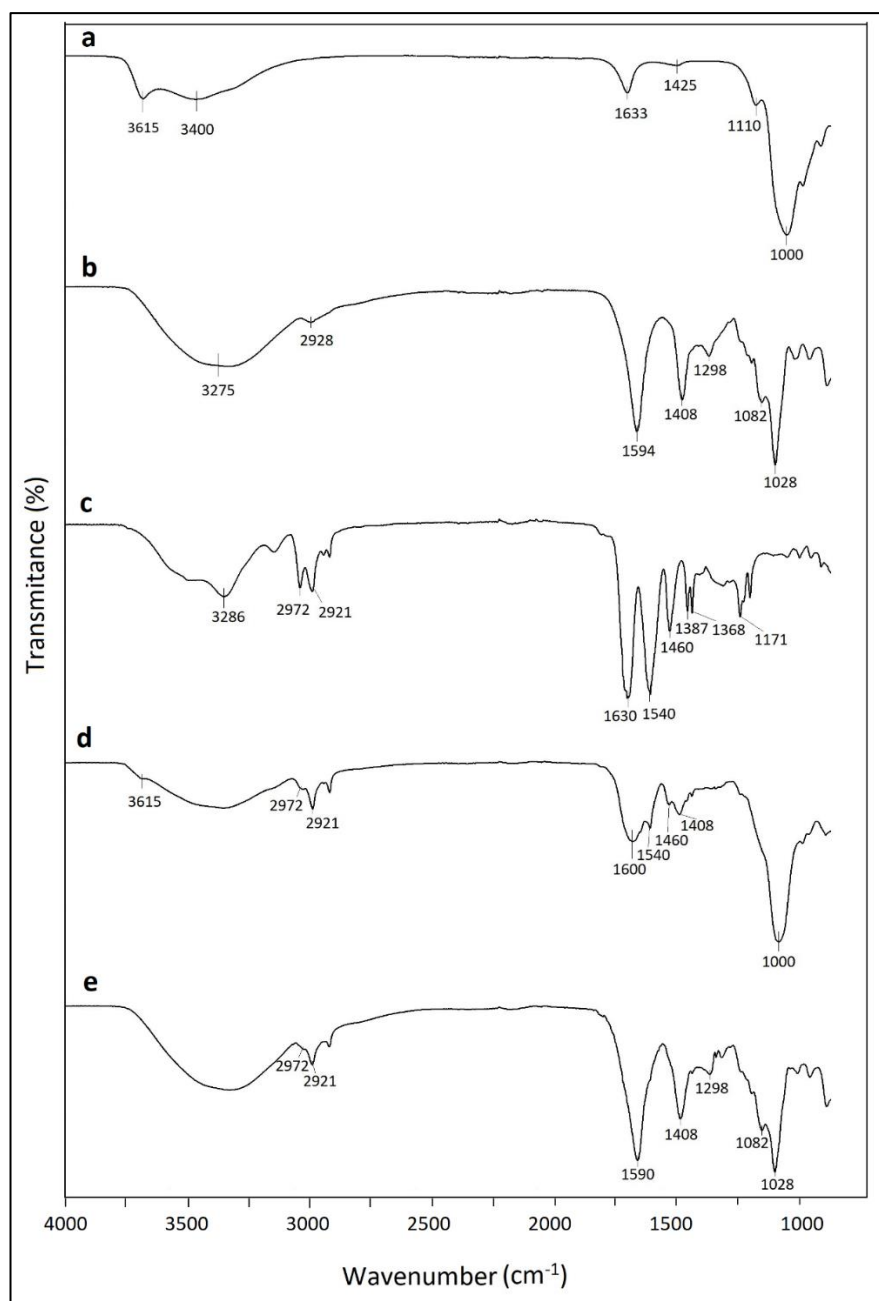
Figure 3.6: The FT-IR absorption spectra of (a) nanoclay, (b) NaAlg, (c) PNIPA and prepared (d) nanocomposite and (e) conventional hydrogels.
