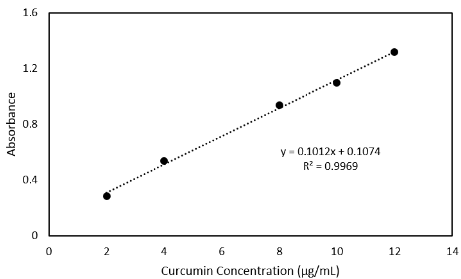
Figure B1.1: UV calibration curve of curcumin at 425 nm.
