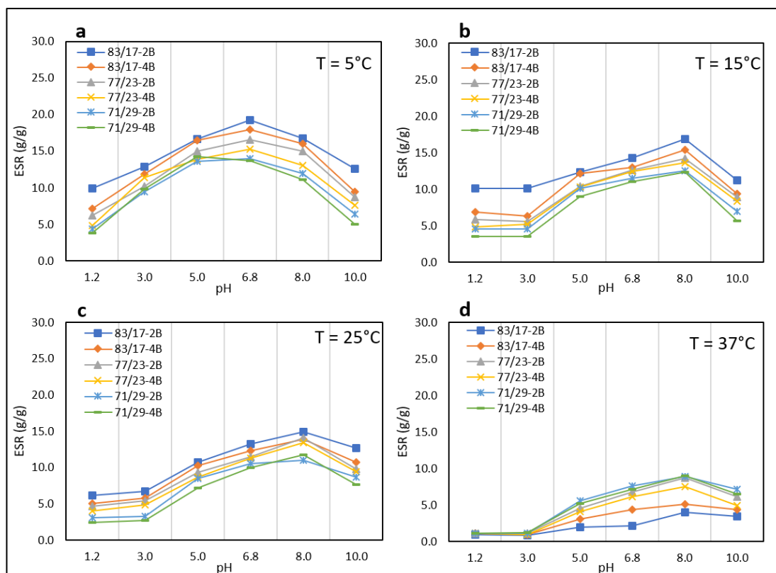
Figure 3.9: The ESR of conventional hydrogels as a function of pH at (a) 5 °C, (b) 15 °C, (c) 25 °C and (d) 37 °C.
