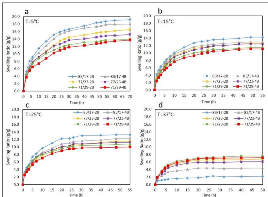
Figure A1.10: Swelling ratio of conventional hydrogels at 5°C (a), 15°C (b), 25°C (c) and 37°C (d) in pH = 6.8.
