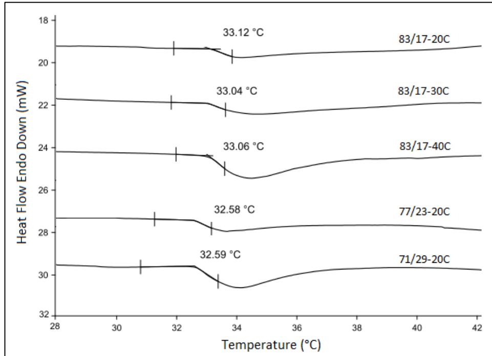
Figure 3.2: DSC thermograms of swollen nanocomposite hydrogels.
