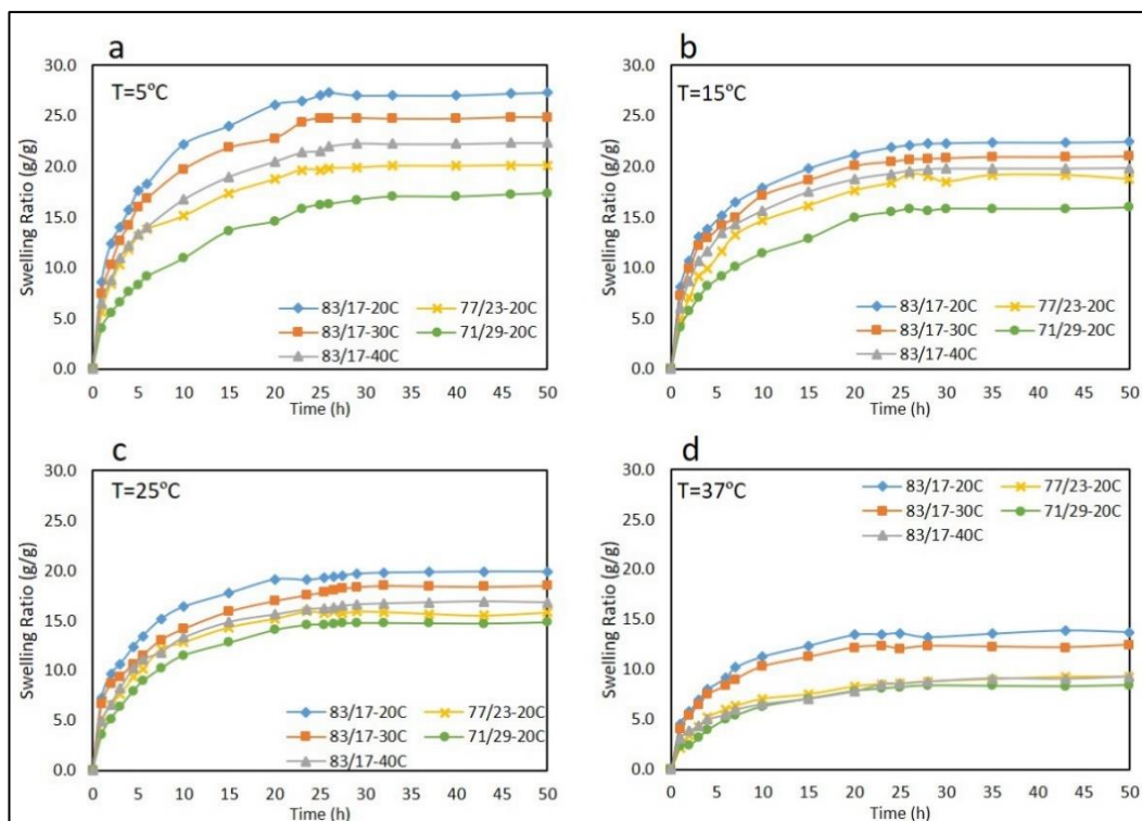
Figure A1.4: Swelling ratio of nanocomposite hydrogels at 5°C (a), 15°C (b), 25 °C (c) and 37°C (d) in pH = 6.8.
