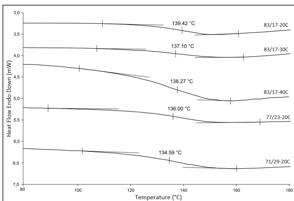
Figure 3.4: DSC thermograms of dried nanocomposite hydrogels.
