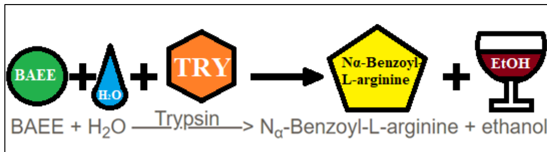
Figure 4.4: BAEE - Trypsin reaction scheme.
