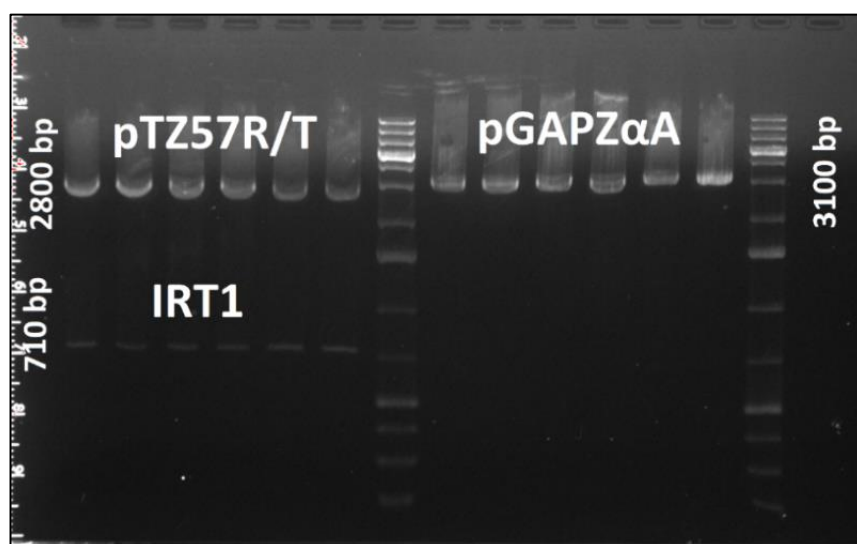
Figure 5.4: Agarose gel (1%) image of pGAPZ \alpha A and restricted pTZ57R/T that including IRT1.
