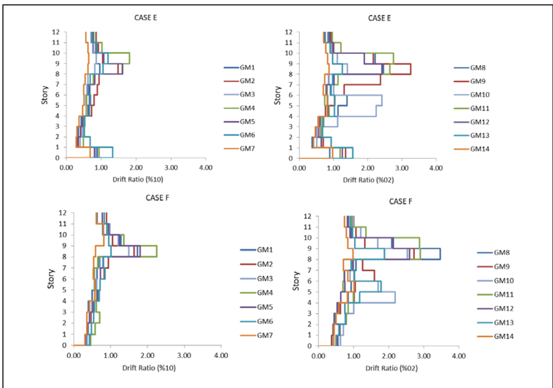
Figure 6.20: Drift ratios for 12- story frames corresponding to 2% and 10% probability of exceedance in 50 year.
