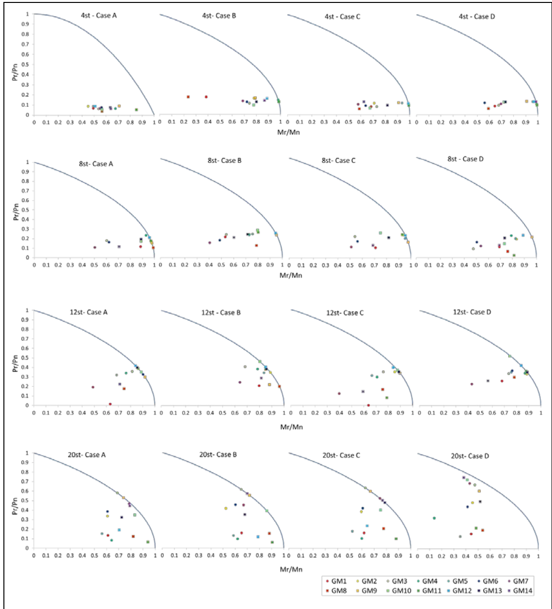
Figure 5.32: The maximum axial load and moment combination variations for each ground motions correspond to 2% and 10% probability of exceedance in 50 year.
