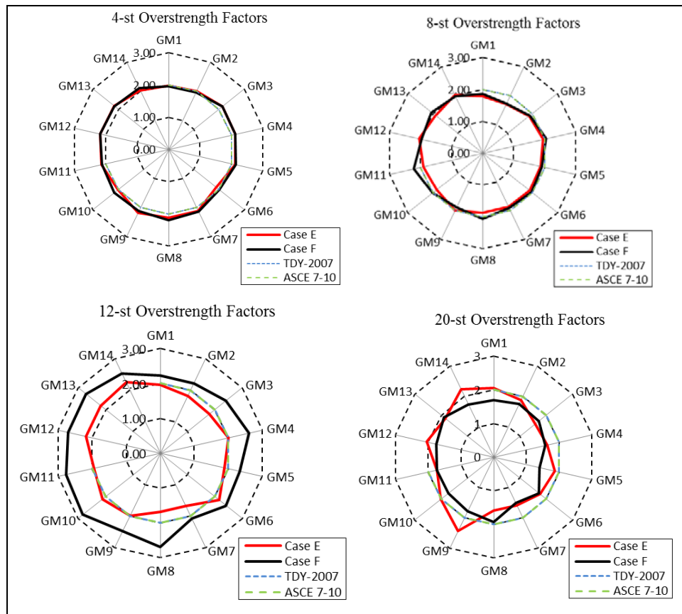
Figure 6.39: Overstrength factors for SCBF's under selected ground motions.
