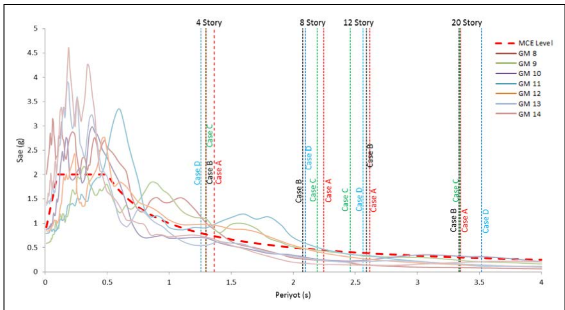
Figure 5.23: Response Spectra of the ground motions (GM8 to GM14) selected from PEER database for design earthquake level corresponding to 2% probability of exceedance in 50 year.
