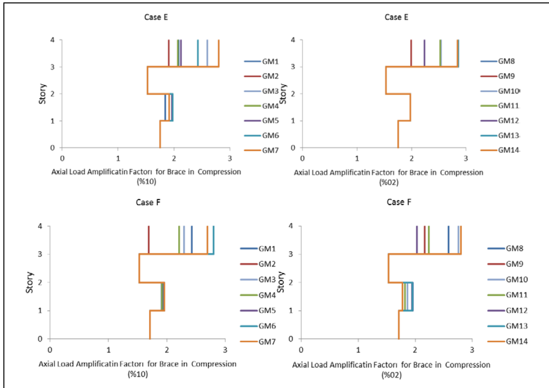
Figure 6.28: Maximum amplification factor for brace in compression in 4- story frames corresponding to 2% and 10% probability of exceedance in 50 year.
