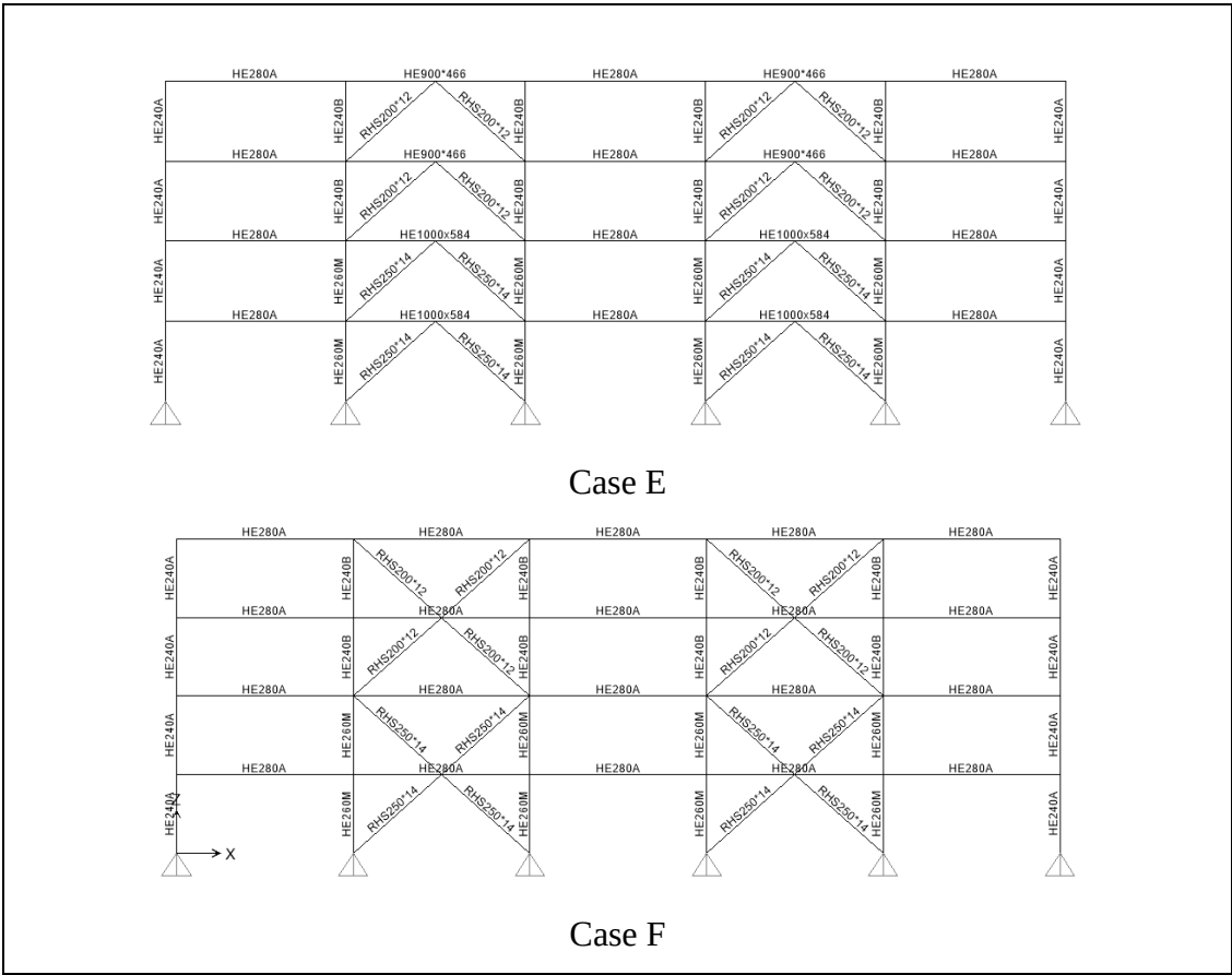
Figure C1.1: Elevations and member sizes for the 4- story SCBF.
