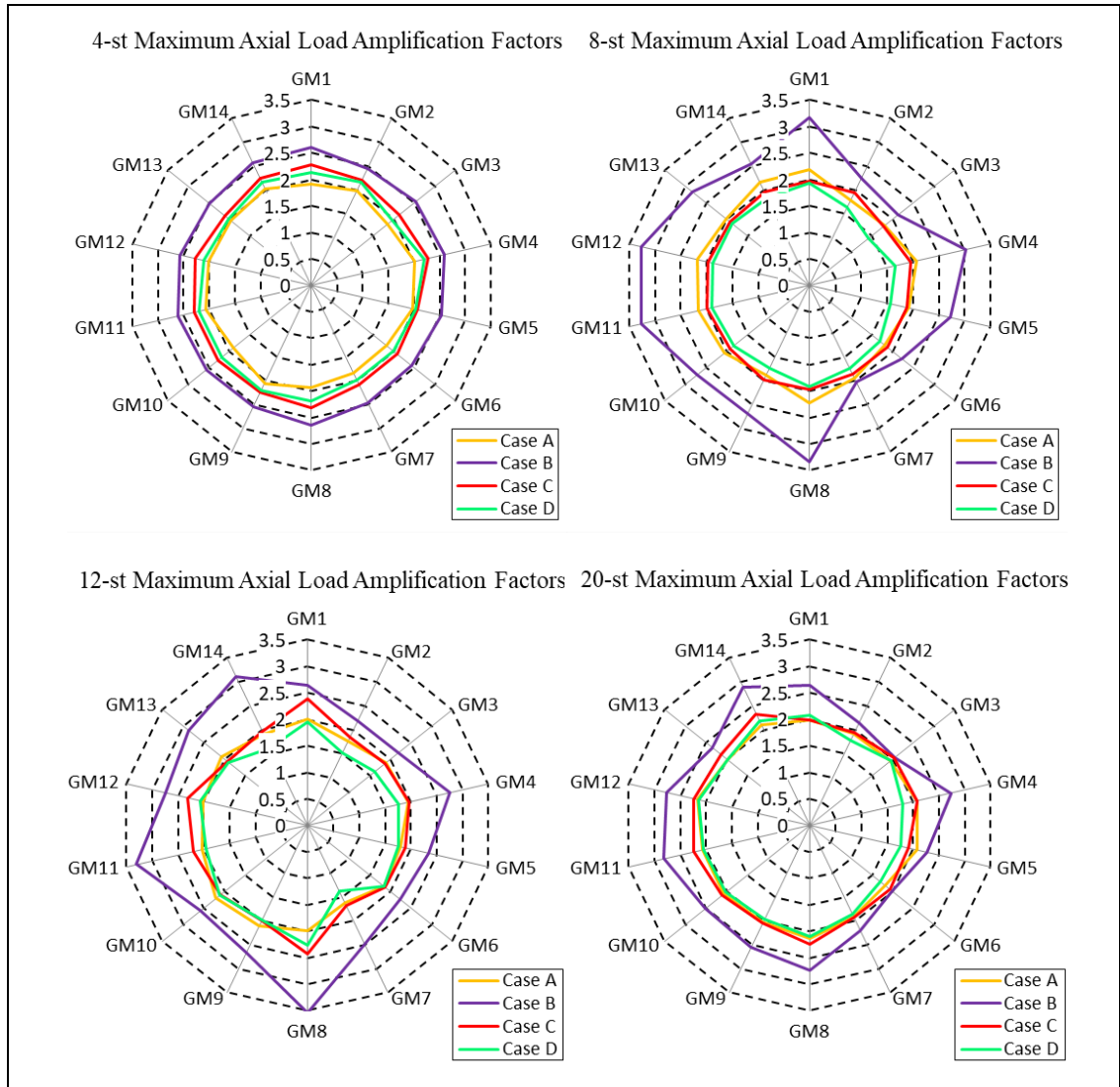
Figure 5.31: Maximum amplification factor in each story frames corresponding to 2% and 10% probability of exceedance in 50 year.
