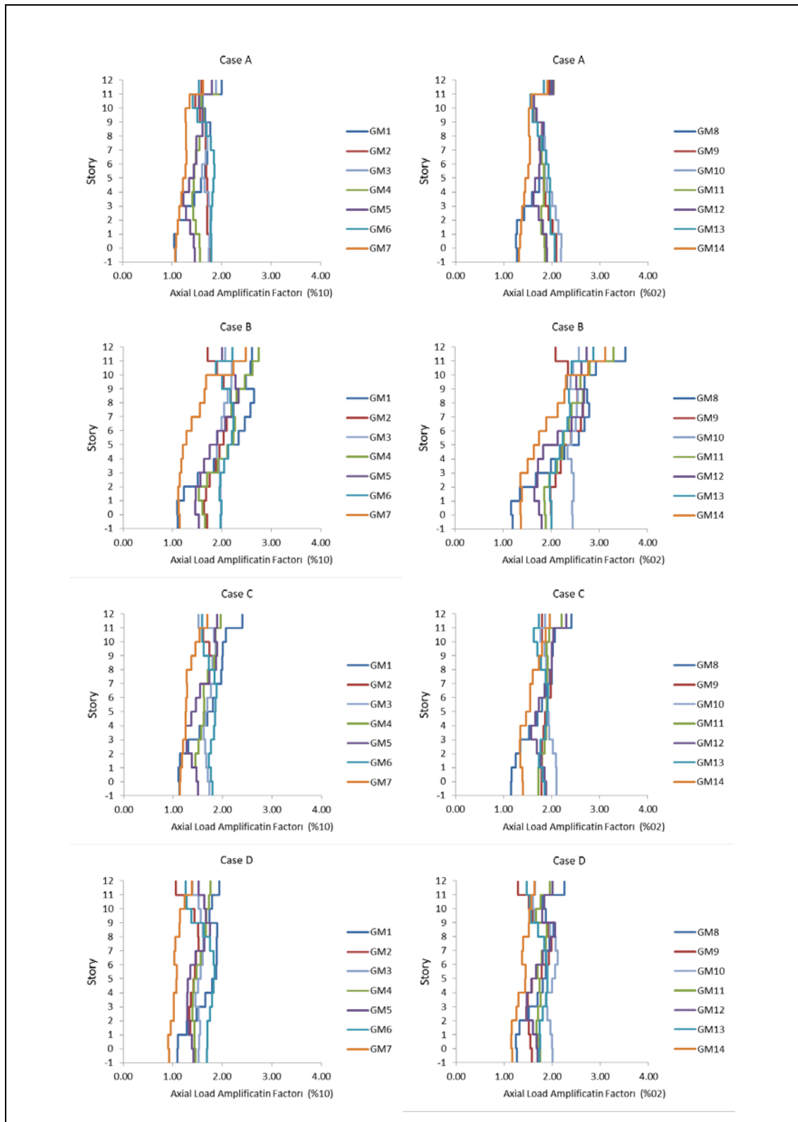
Figure 5.28: Maximum amplification factor for 12- story frames corresponding to 2% and 10% probability of exceedance in 50 year.
