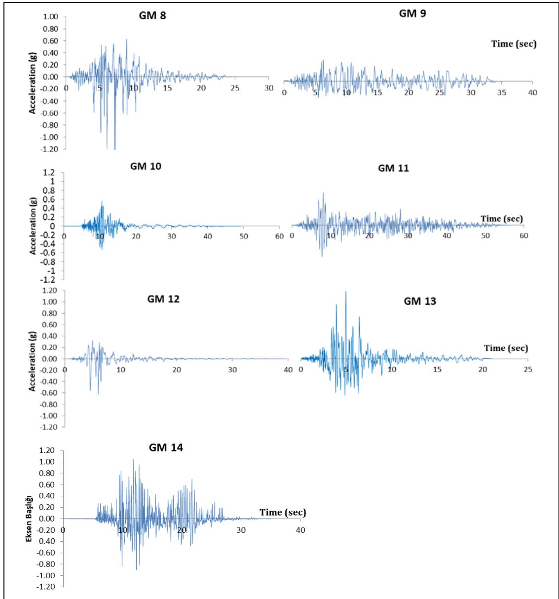
Figure 6.15: Acceleration time histories of the selected ground motions corresponding to 2% probability of exceedance in 50 year.
