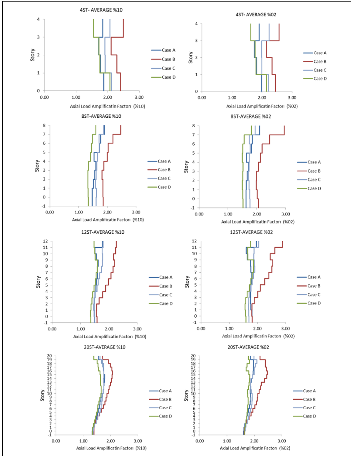
Figure 5.30: Maximum average amplification factor in each story frames corresponding to 2% and 10% probability of exceedance in 50 year.
