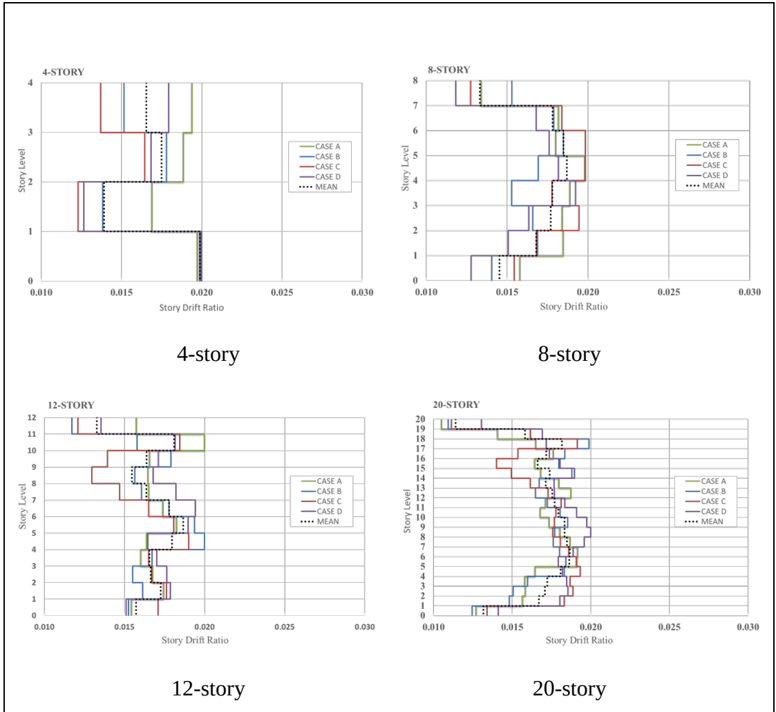
Figure 5.4: Story drift ratio of SMF.
