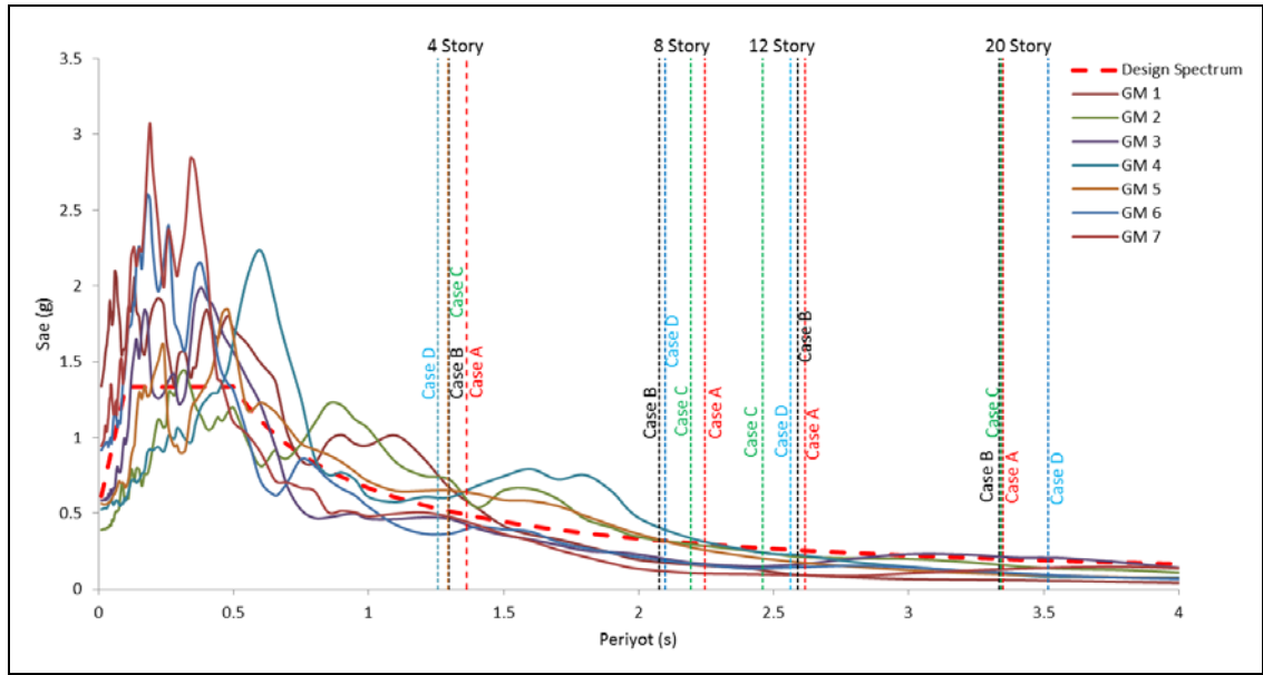
Figure 5.22: Response Spectra of the ground motions (GM1 to GM7) selected from PEER database for design earthquake level corresponding to 10% probability of exceedance in 50 year.
