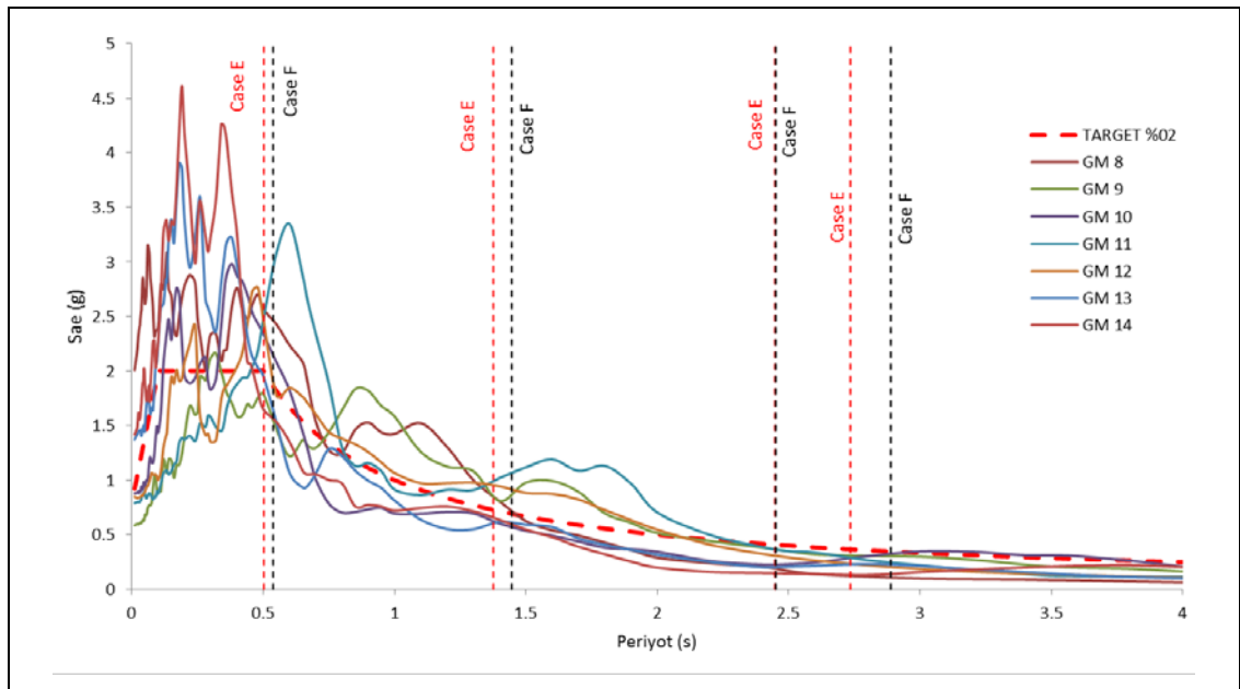
Figure 6.17: Response Spectra of the ground motions (GM8 to GM14) selected from PEER database for design earthquake level corresponding to 2% probability of exceedance in 50 year.
