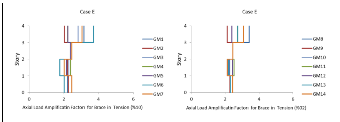
Figure 6.32: Maximum amplification factor for brace in tension in 4- story frames corresponding to 2% and 10% probability of exceedance in 50 year.
