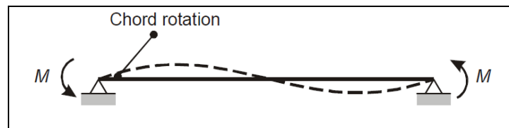
Figure 5.11: Chord rotation model.
