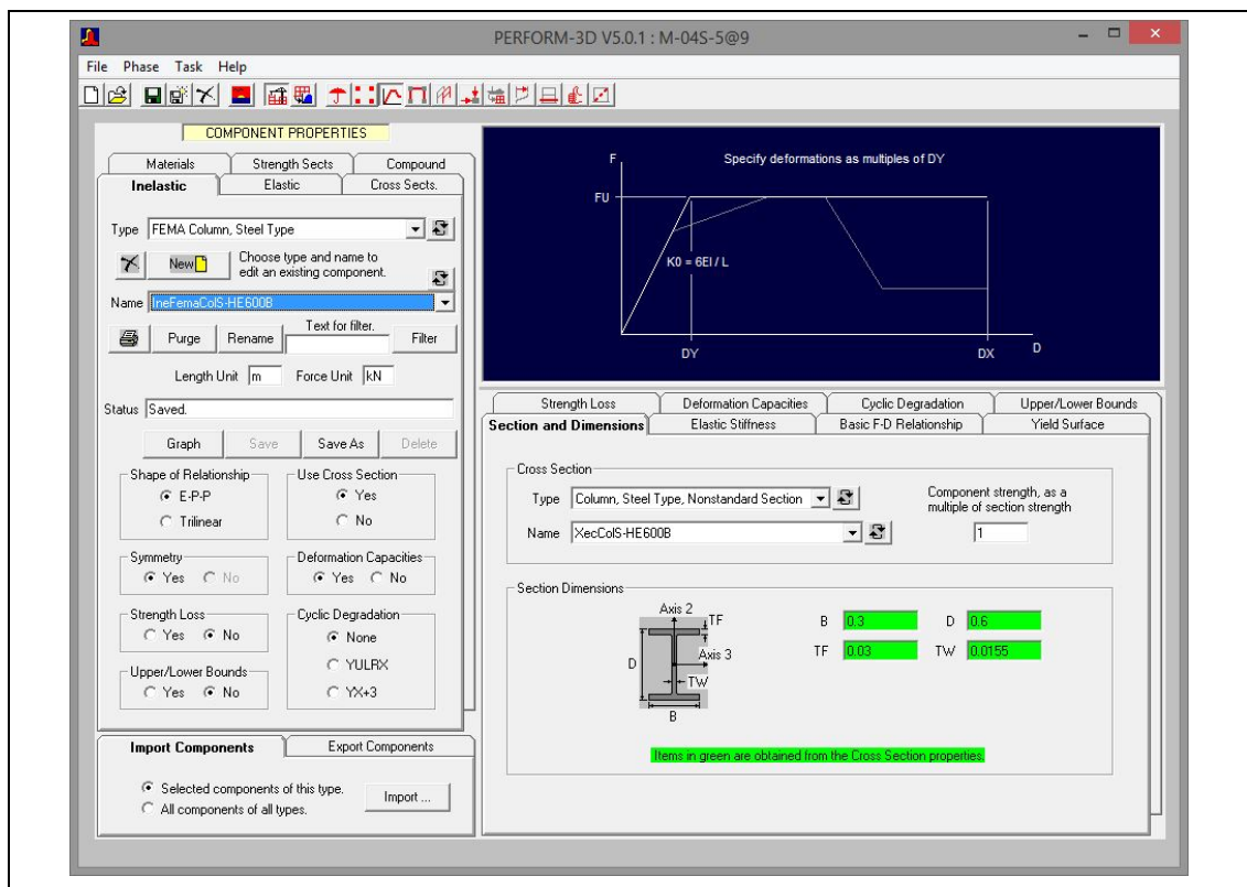
Figure 5.15: Fema Column, Steel Type menu for HE600B section.
