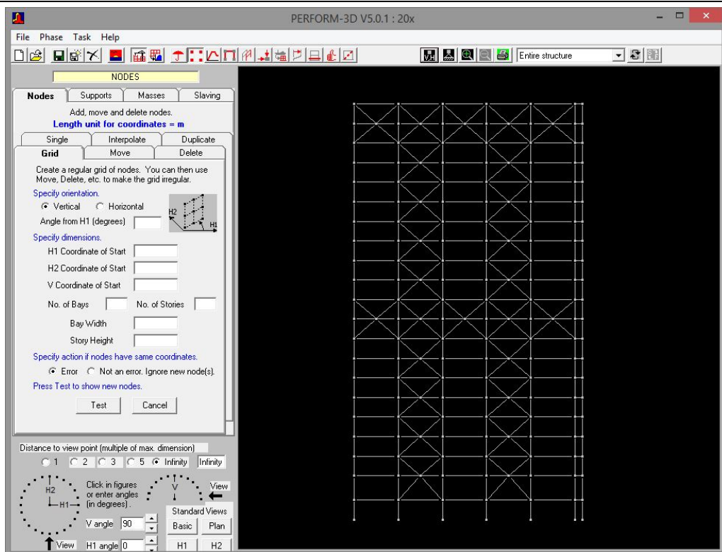
20 – Story Frame (two story X-Braced model)
