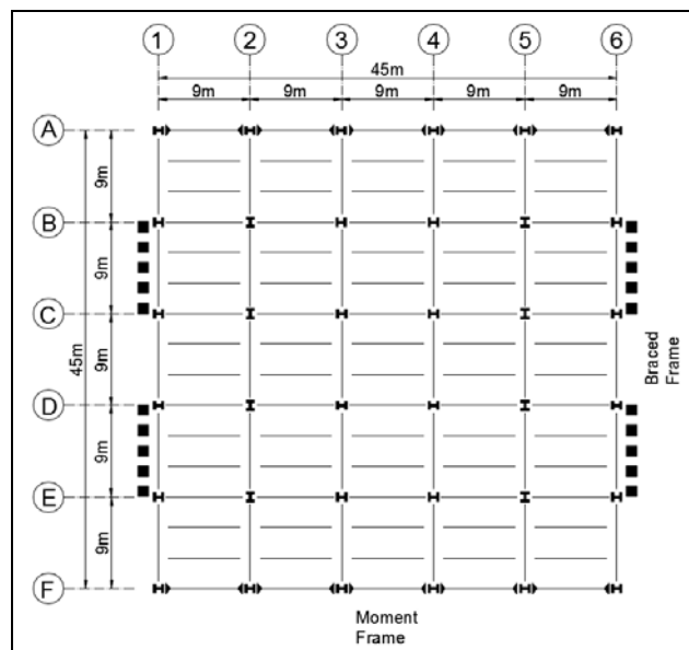
Figure 6.1: Plan of the 4-, 8-, 12- and 20- story SCBF buildings.
