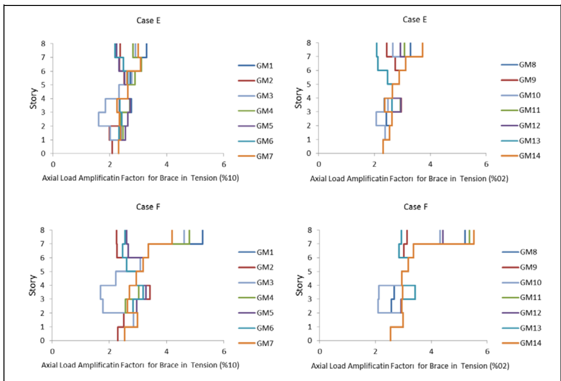
Figure 6.33: Maximum amplification factor for brace in tension in 8- story frames corresponding to 2% and 10% probability of exceedance in 50 year.
