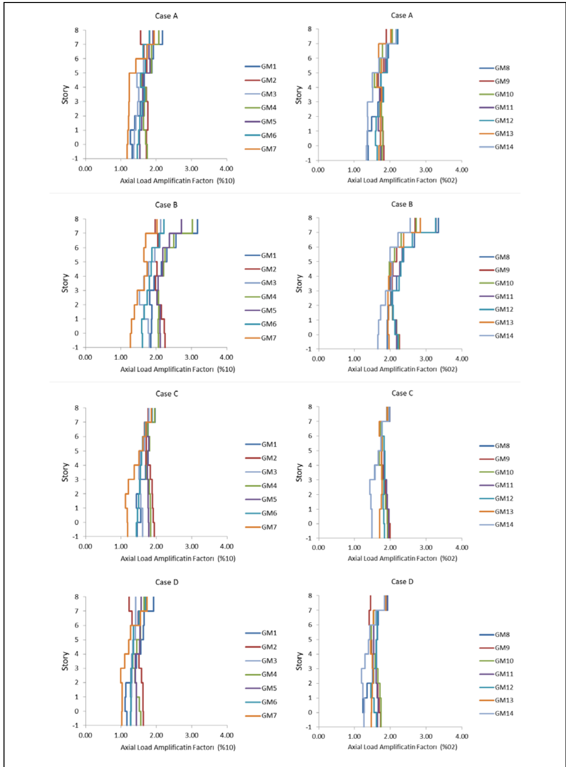
Figure 5.27: Maximum amplification factor for 8- story frames corresponding to 2% and 10% probability of exceedance in 50 year.
