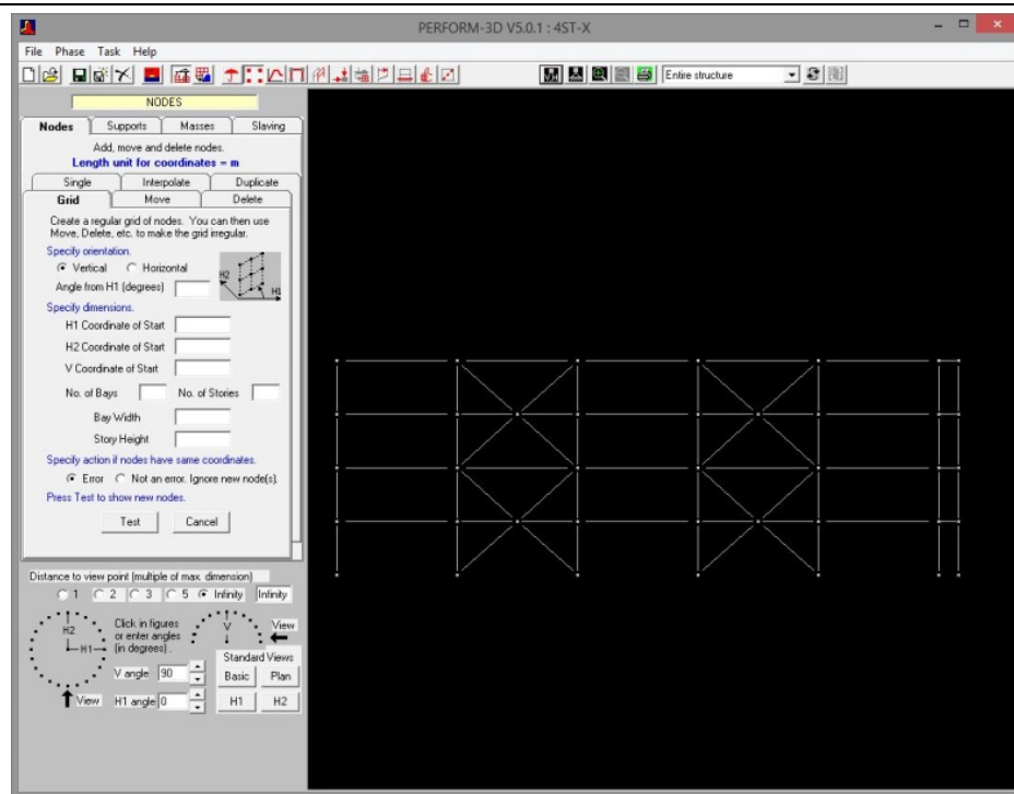
4 – Story Frame (two story X-Braced model)
