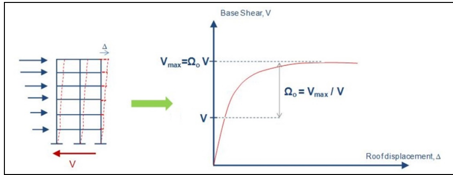
Figure 1.1: Schematic illustration of amplified seismic load, ( \Omega_0 )
