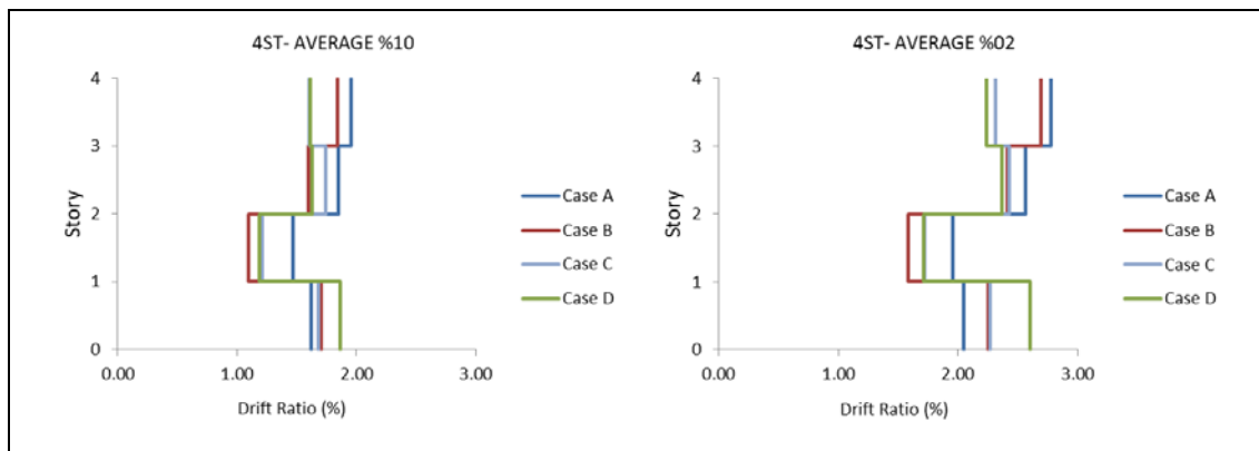
Figure 5.24: Average of maximum drift ratio in each story corresponding to 2% and 10% probability of exceedance in 50 year.
