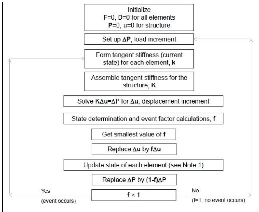
Figure 4.3: Detailed algorithm of load increments.
