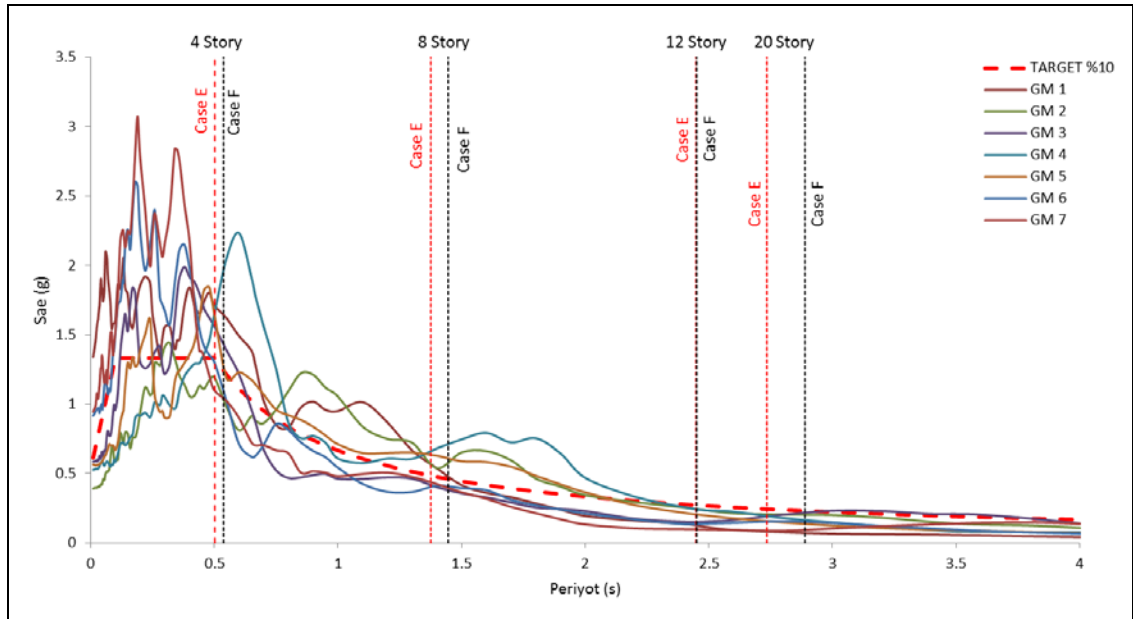
Figure 6.16: Response Spectra of the ground motions (GM1 to GM7) selected from PEER database for design earthquake level corresponding to 10% probability of exceedance in 50 year.
