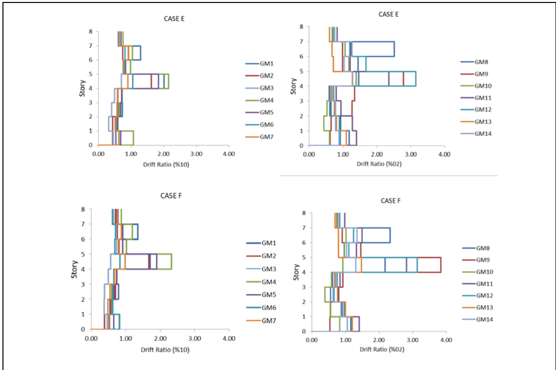
Figure 6.19: Drift ratios for 8- story frames corresponding to 2% and 10% probability of exceedance in 50 year.
