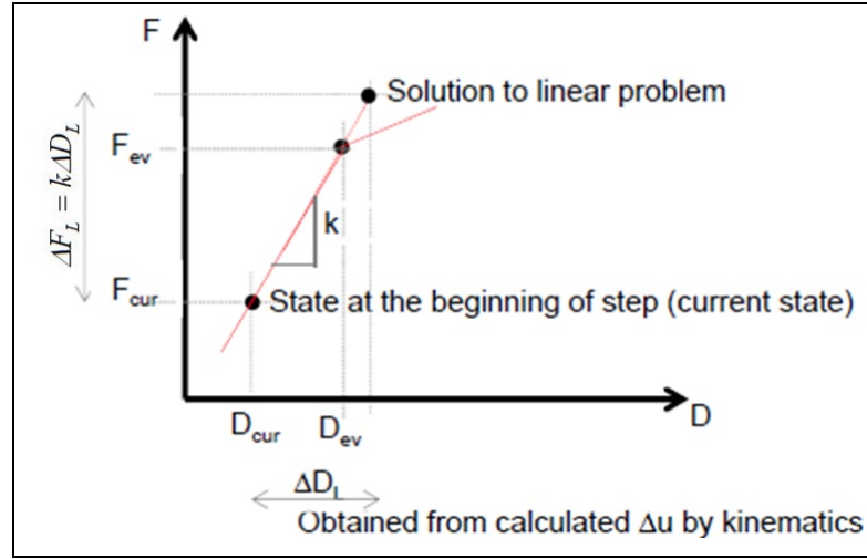
Figure 4.2: Typical element in a structural model.
