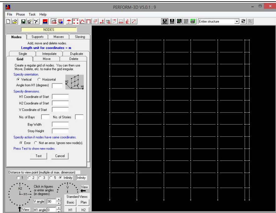
8 Story frame model
