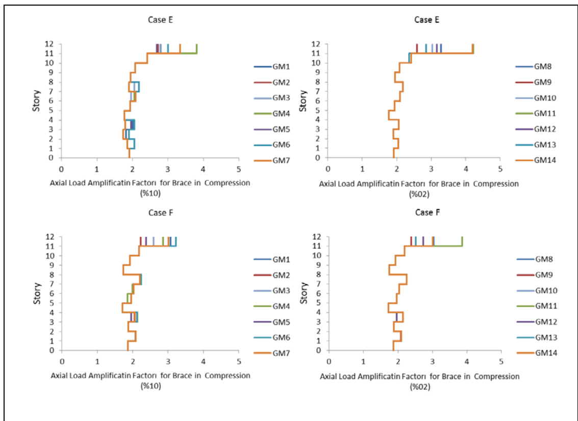
Figure 6.30: Maximum amplification factor for brace in compression in 12- story frames corresponding to 2% and 10% probability of exceedance in 50 year.
