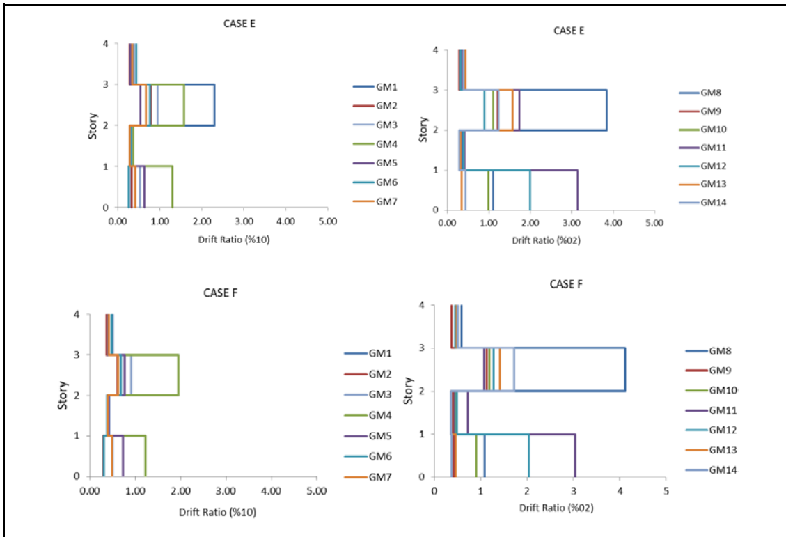
Figure 6.18: Drift ratios for 4- story frames corresponding to 2% and 10% probability of exceedance in 50 year.
