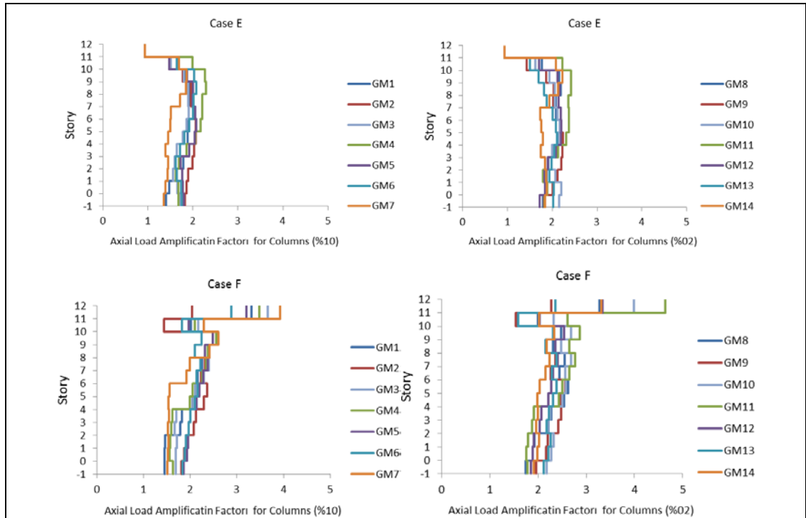
Figure 6.26: Maximum amplification factor for 12- story frames corresponding to 2% and 10% probability of exceedance in 50 year.
