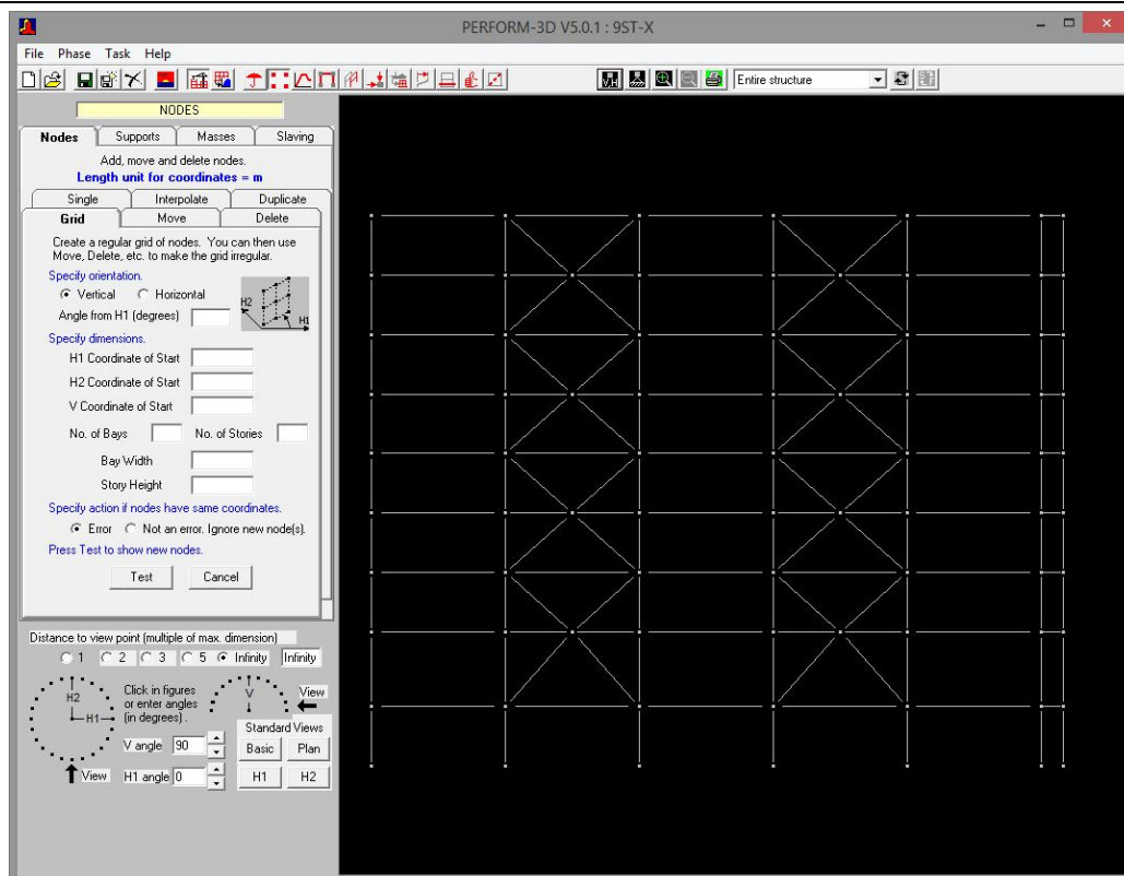
8 – Story Frame (two story X-Braced model)
