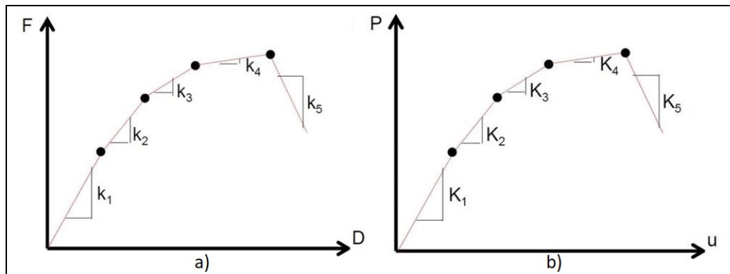
Figure 4.1: a) Multi linear element/component, b) structure model.
