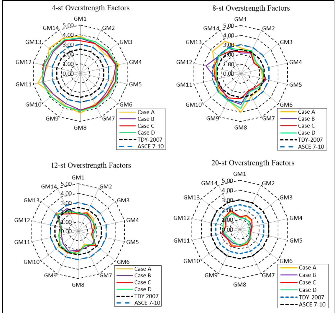
Figure 5.37: Overstrength factors under selected ground motions.
