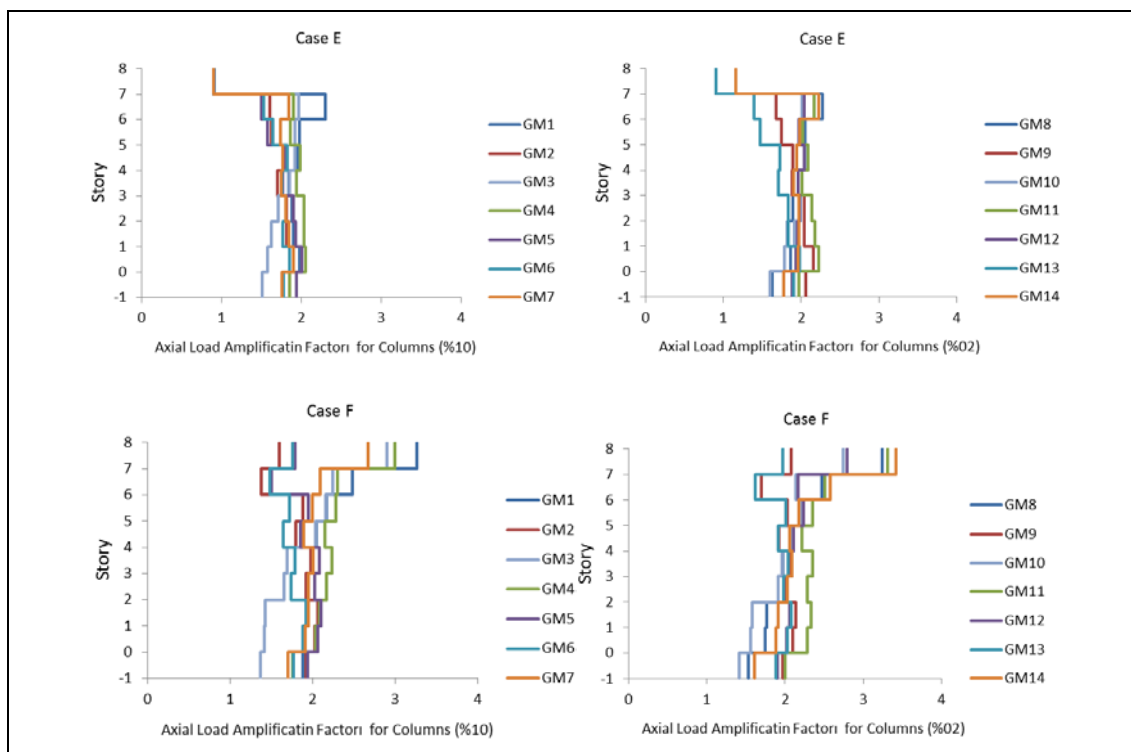
Figure 6.25: Maximum amplification factor for 8- story frames corresponding to 2% and 10% probability of exceedance in 50 year.
