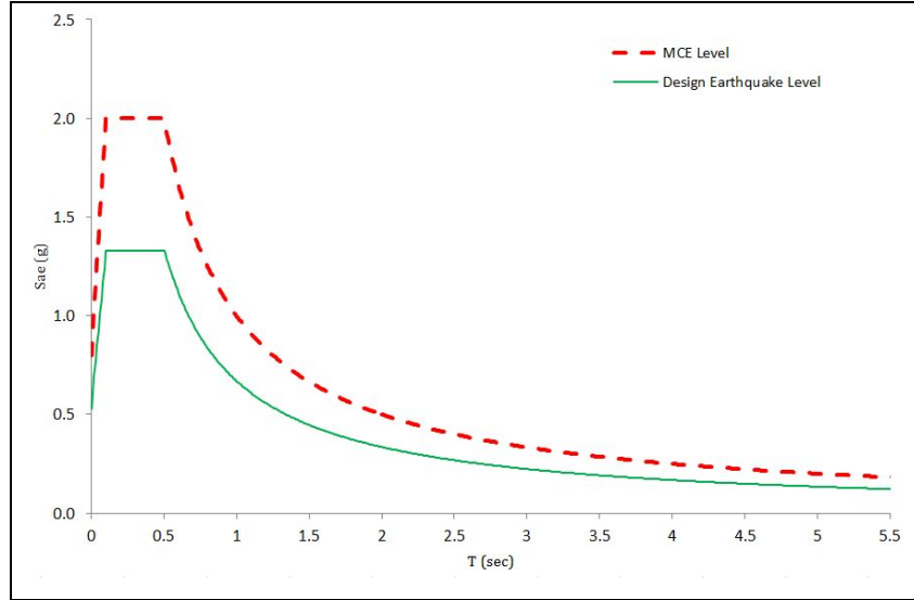
Figure 5.3: Response Spectra for DBE and MCE levels for SMF.
