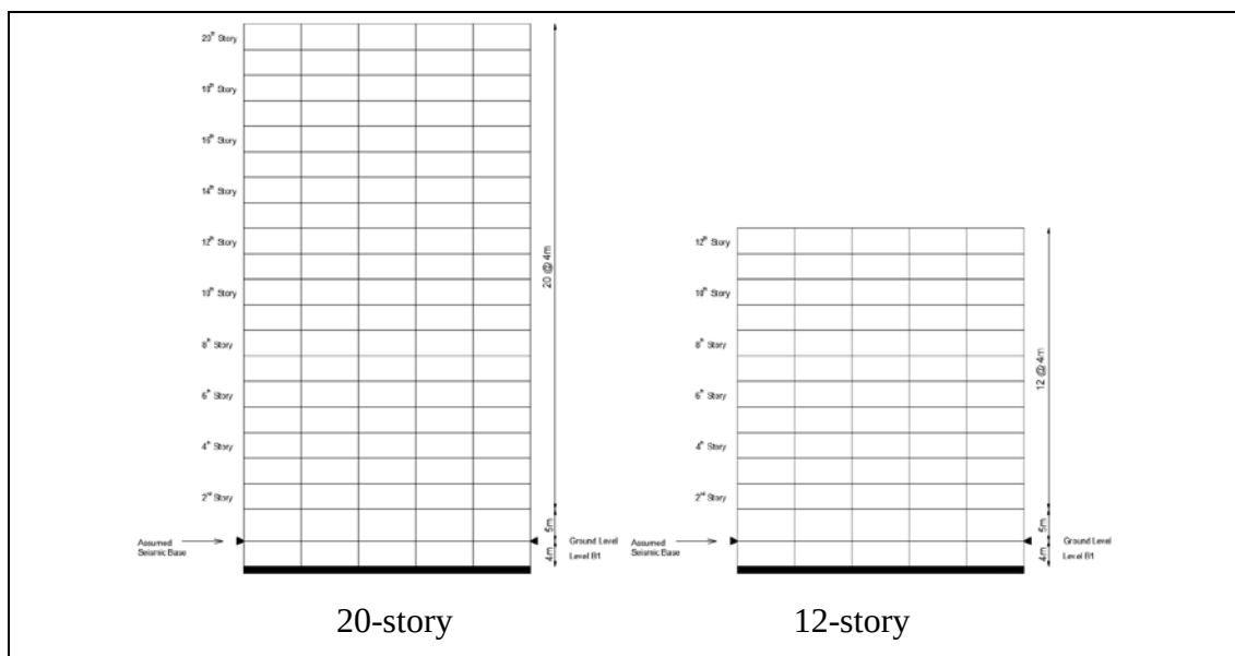
Figure 5.2: Elevations of the SMF buildings.
