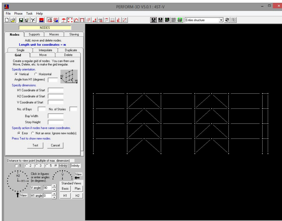
4 – Story Frame (two story Inverted-V Brace model)
