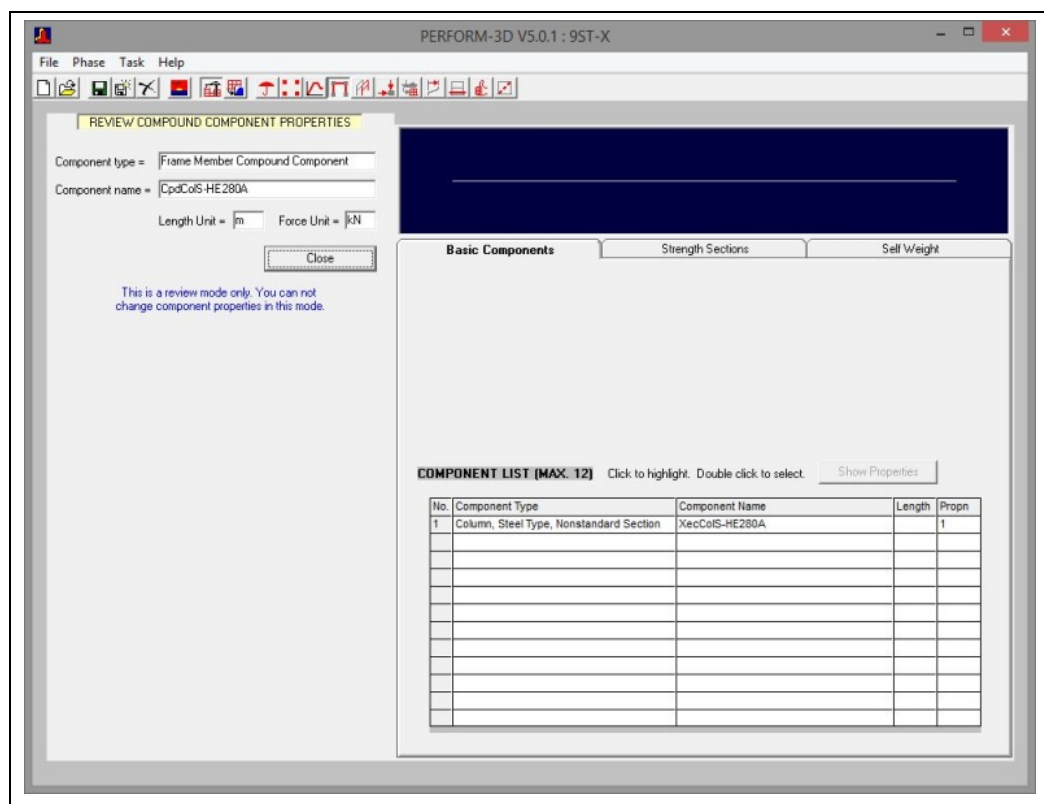
Figure 6.8: Compound menu for HE280A gravity column.
