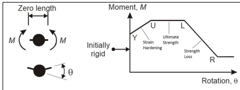
Figure 5.5: Plastic Hinge.
