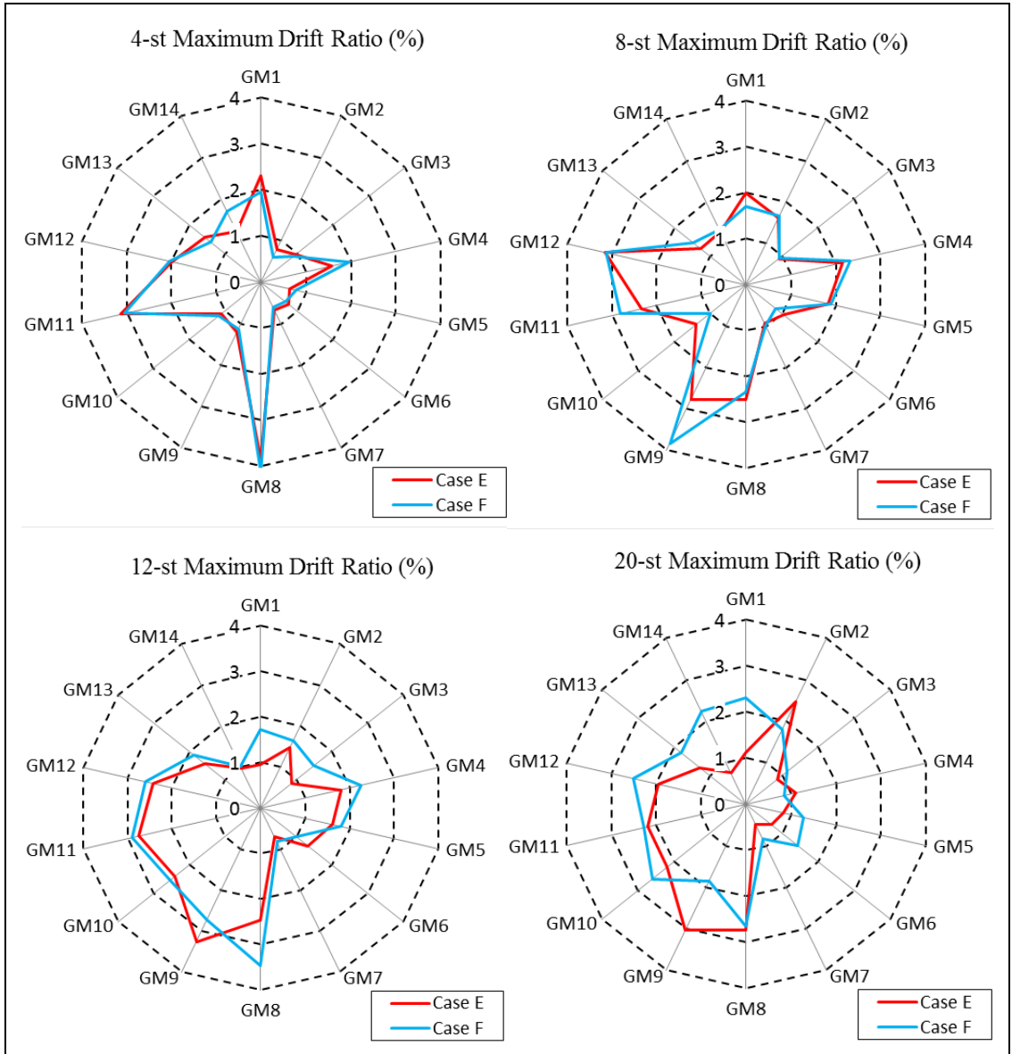
Figure 6.23: Drift Maximum drift ratio in each frame corresponding to 2% and 10% probability of exceedance in 50 year.
