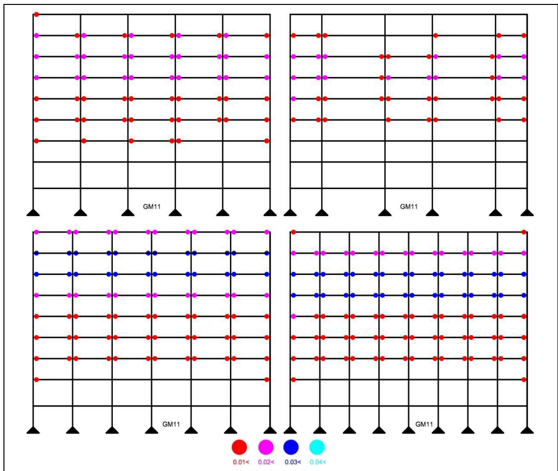
Figure 5.34: Highest plastic hinge rotations for 8 story frames.
