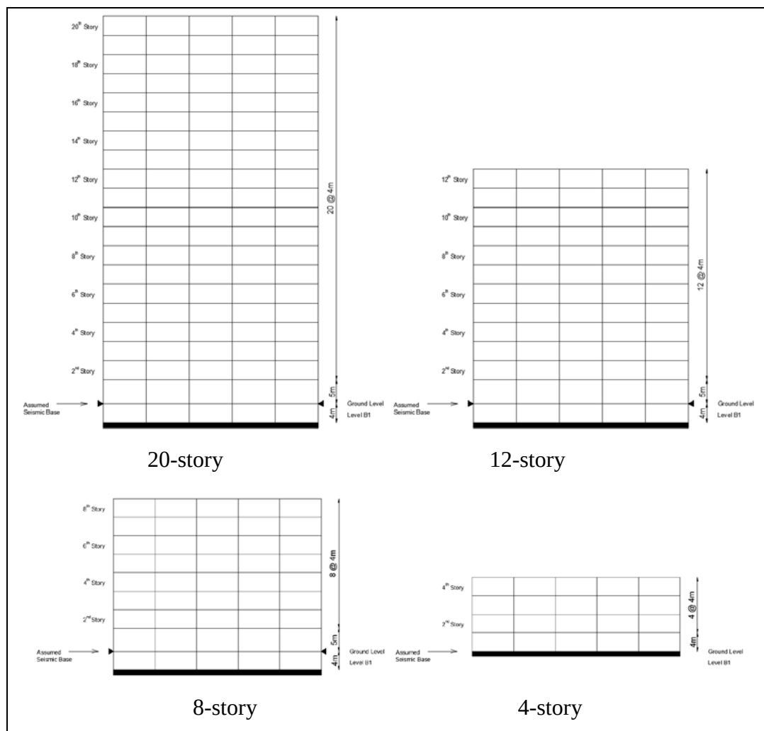
Figure 6.2: Elevations of the SCBF buildings.
