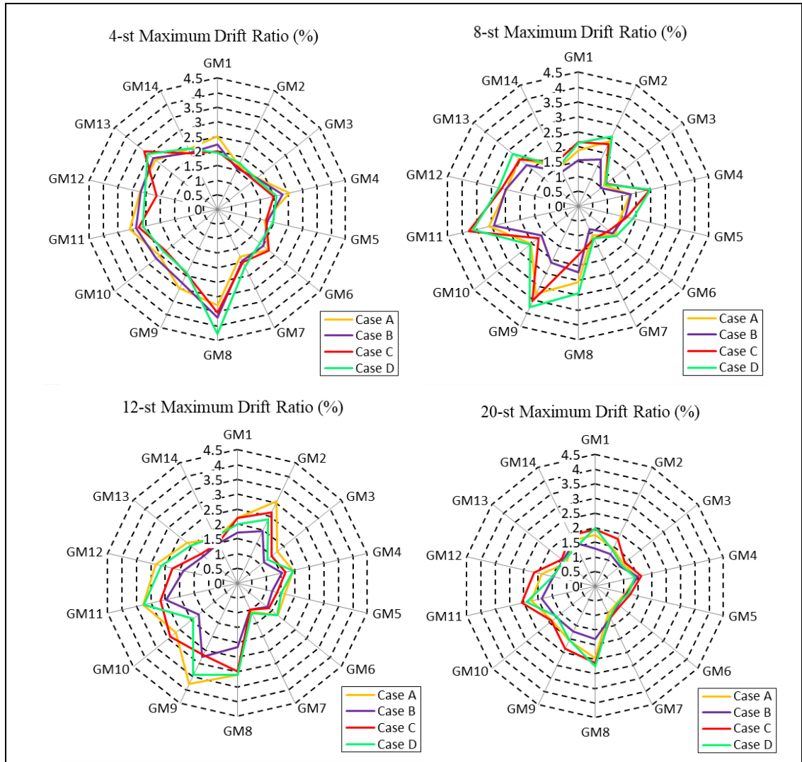
Figure 5.25: Drift Maximum drift ratio in each frame corresponding to 2% and 10% probability of exceedance in 50 year.
