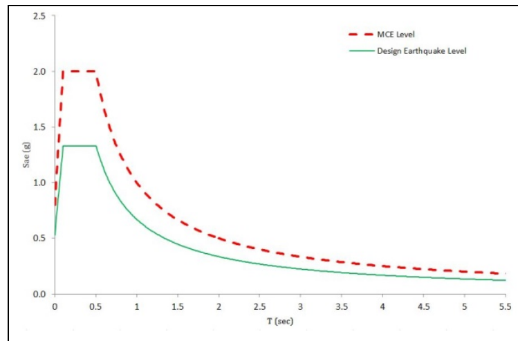
Figure 6.3: Response Spectra for DBE and MCE levels for SCBF.
