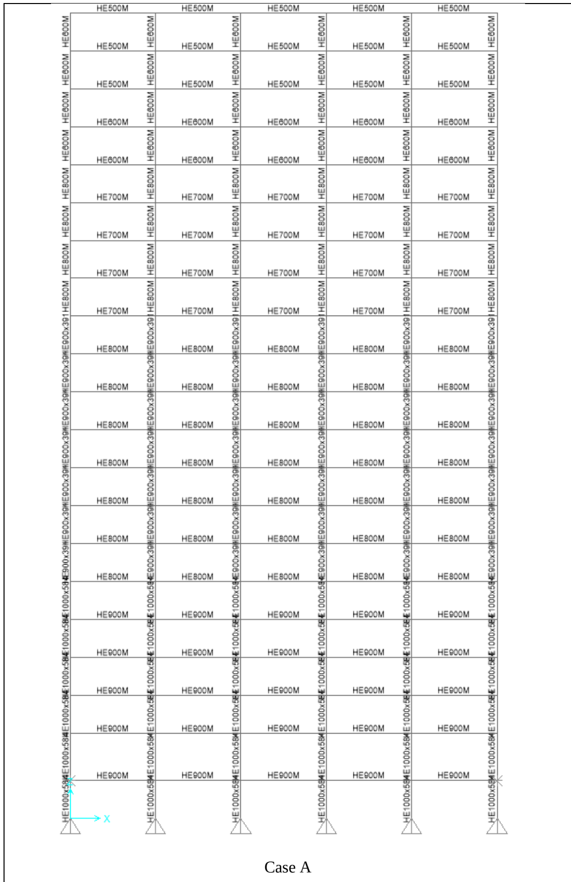
Figure B1.4: Elevations and member sizes for the 20- story SMF.
