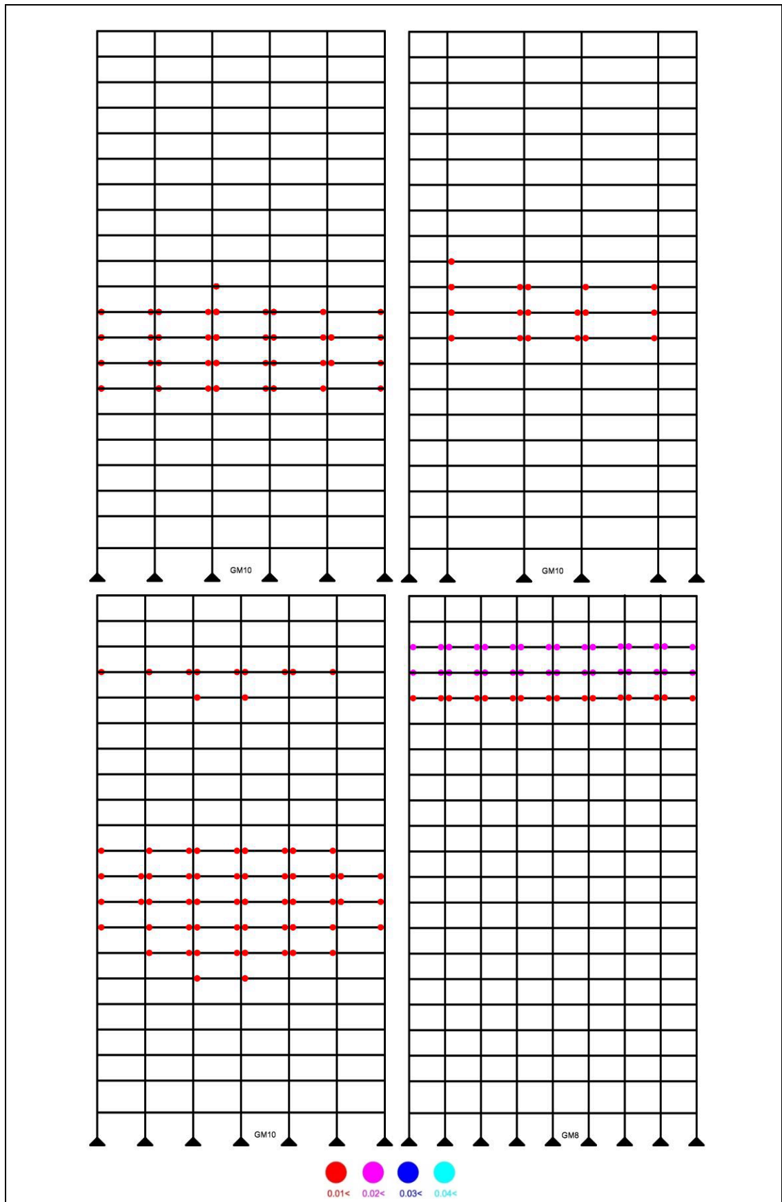
Figure 5.36: Highest plastic hinge rotations for 20 story frames.
