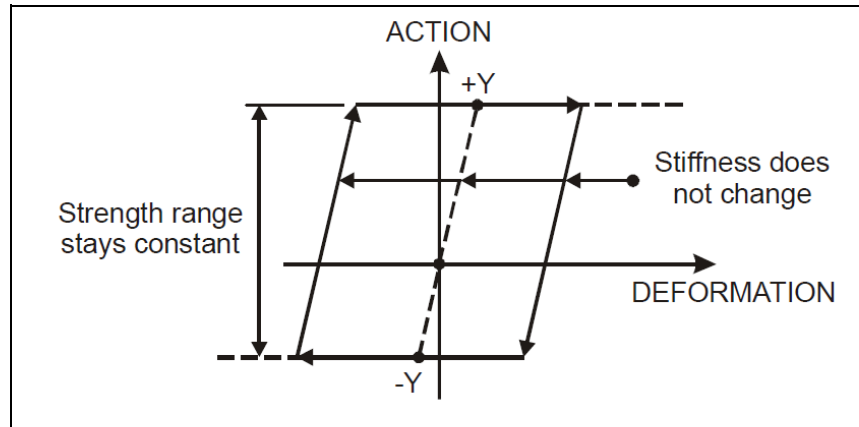
Figure 5.13: Non-Degrading Loop for E-P-P Behavior.
