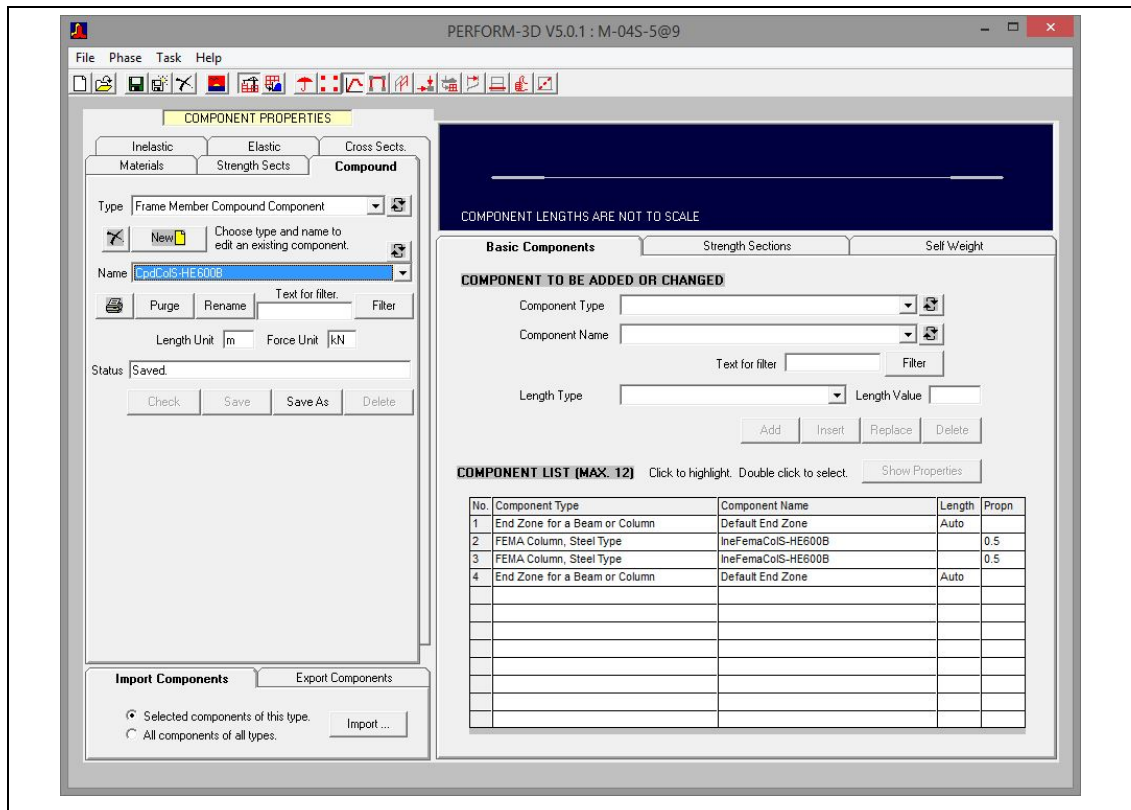
Figure 5.14: Column compound model for HE600B section.
