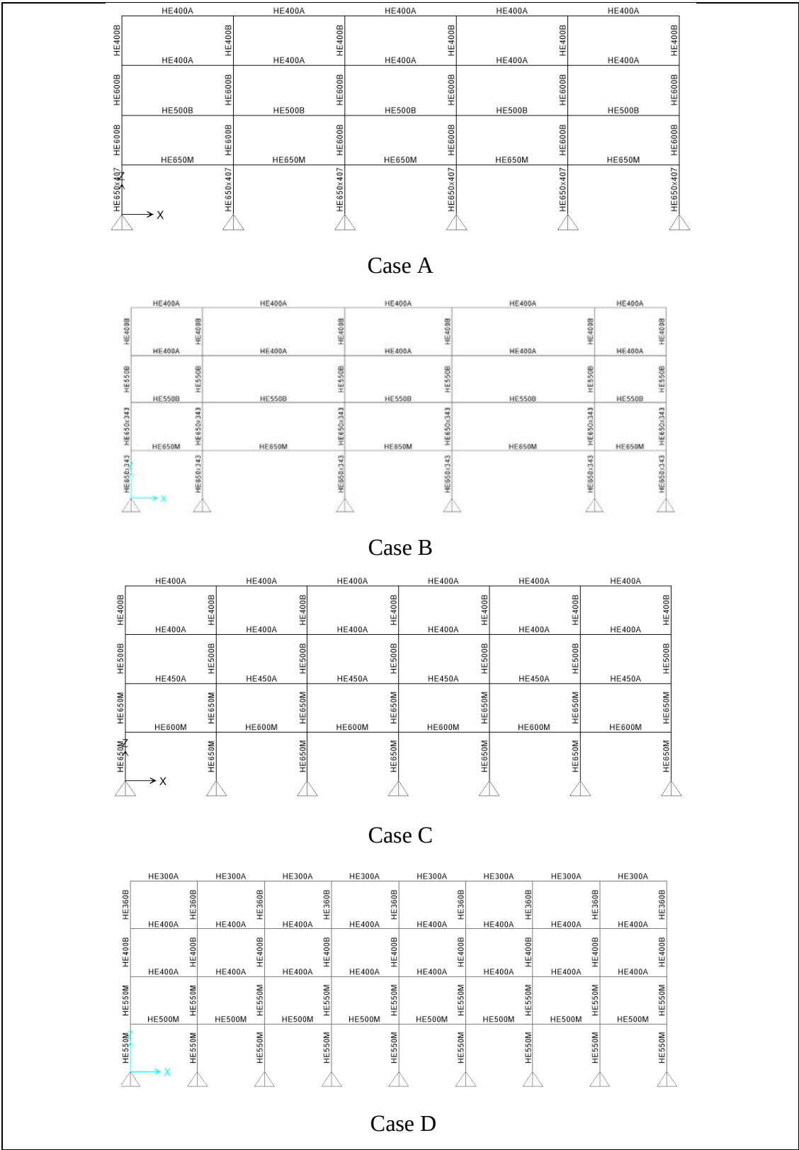
Figure B1.1: Elevations and member sizes for the 4- story SMF.
