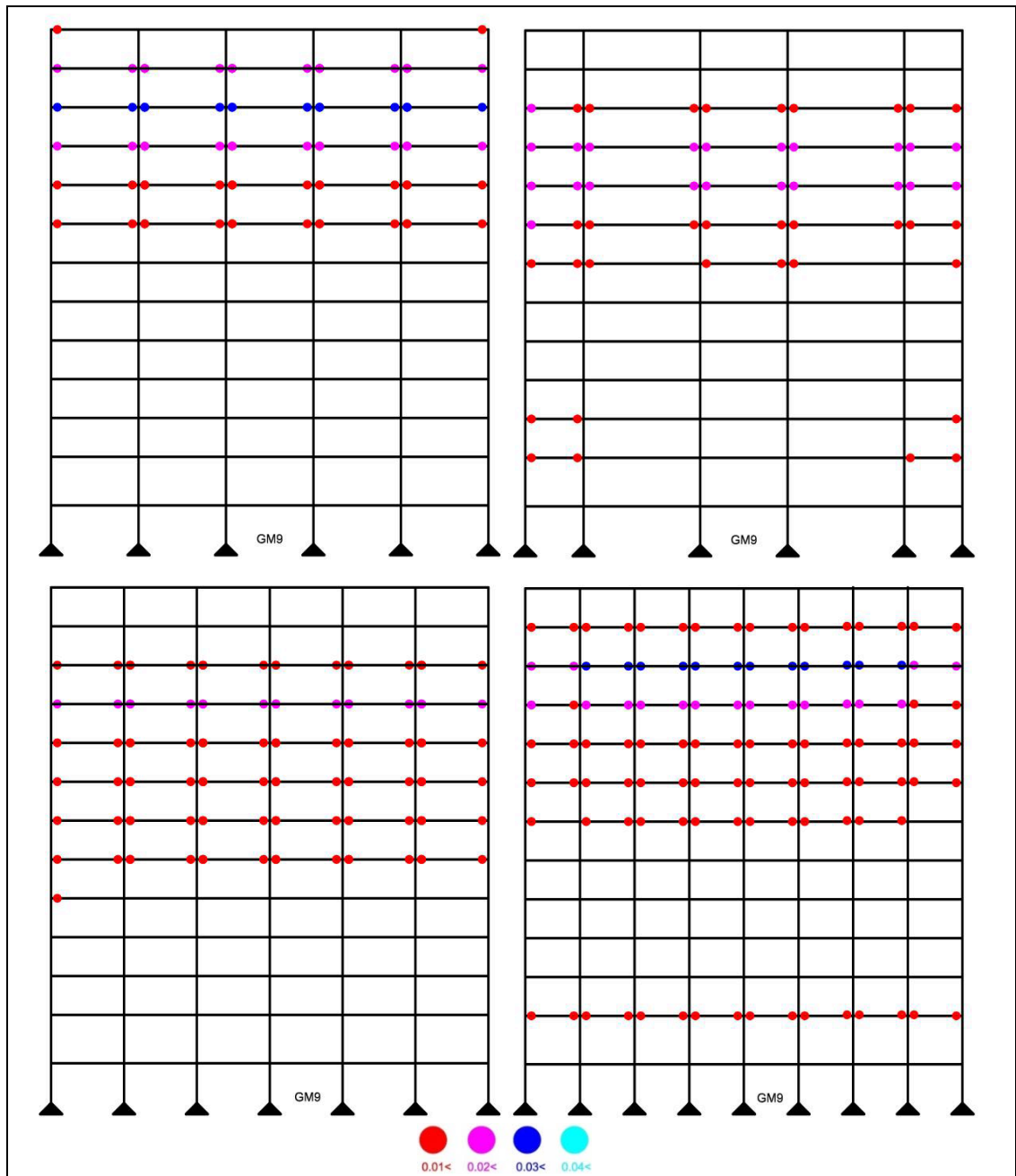
Figure 5.35: Highest plastic hinge rotations for 12 story frames.
