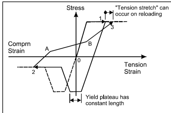
Figure 6.6: Buckling Hysteresis Loop.
