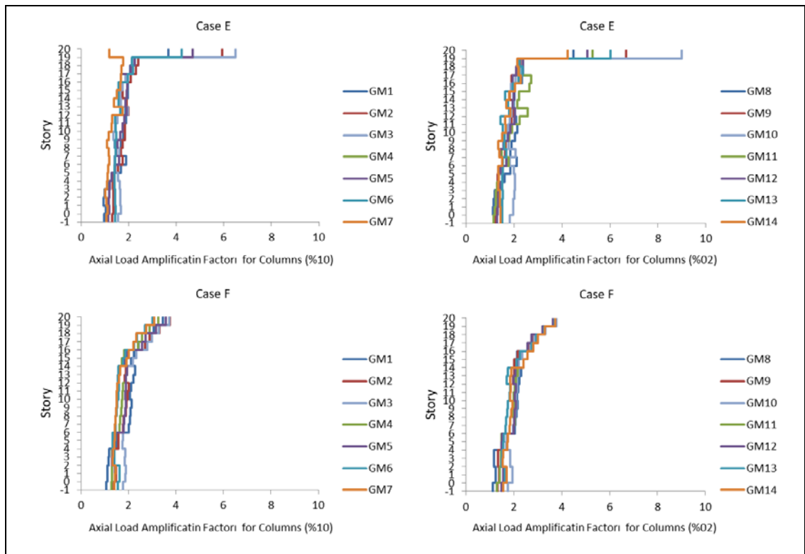
Figure 6.27: Maximum amplification factor for 20- story frames corresponding to 2% and 10% probability of exceedance in 50 year.
