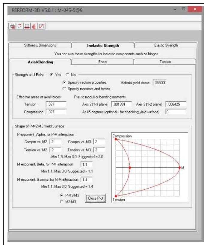
Figure 5.18: Yield surface arrangement in Perform 3D.
