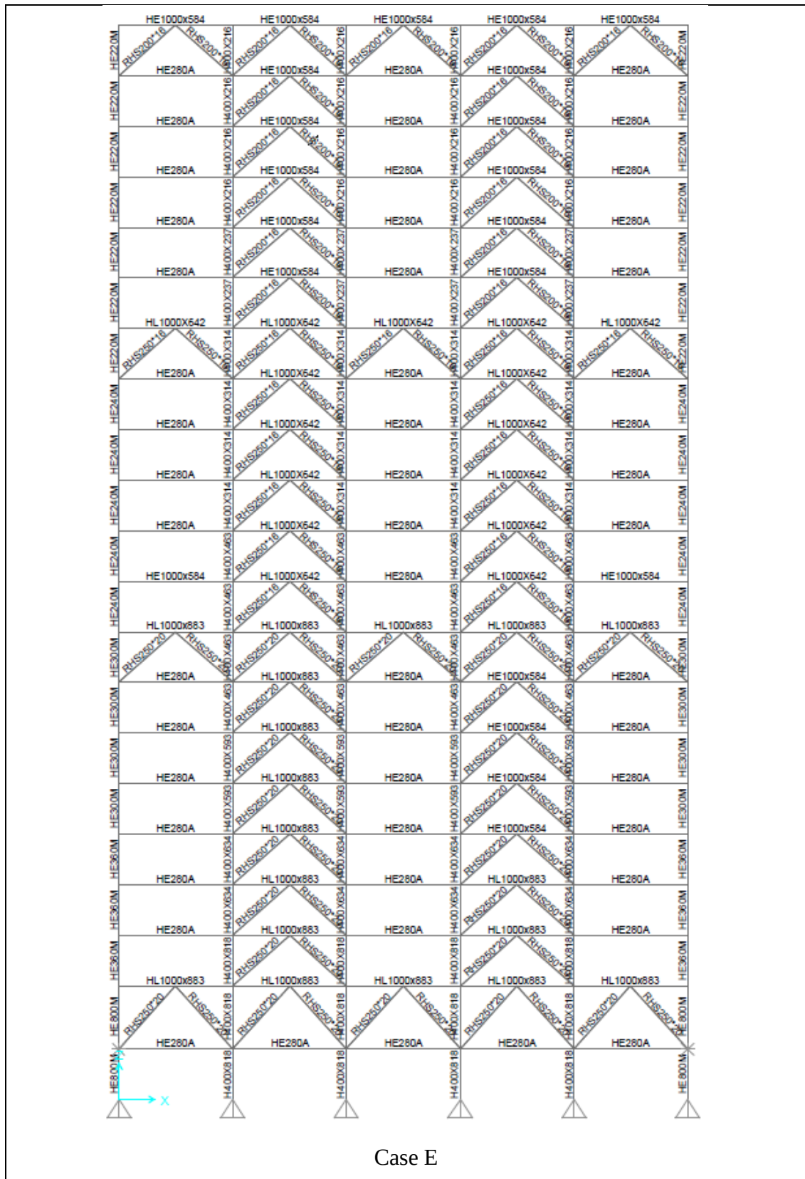
Figure C1.4: Elevations and member sizes for the 20- story SCBF.
