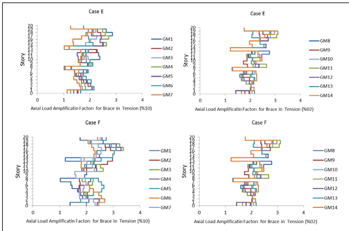
Figure 6.35: Maximum amplification factor for brace in tension in 20- story frames corresponding to 2% and 10% probability of exceedance in 50 year.
