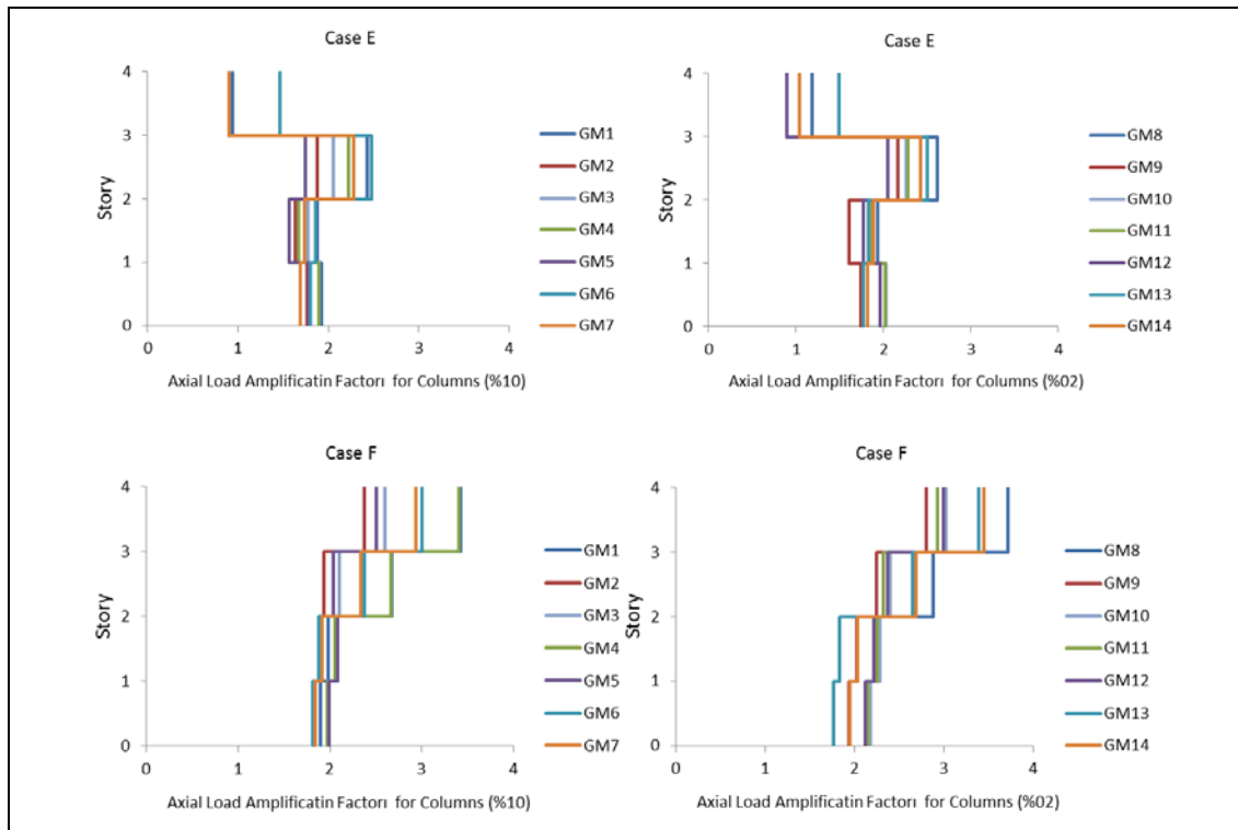
Figure 6.24: Maximum amplification factor for 4- story frames corresponding to 2% and 10% probability of exceedance in 50 year.
