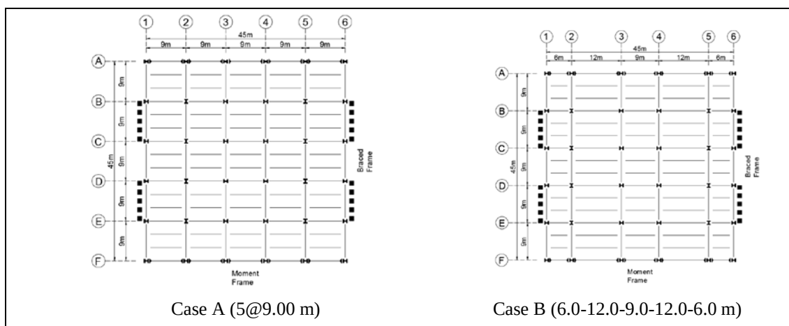
Figure 5.1: Plan of the 4-, 8-, 12- and 20- story SMF buildings.
