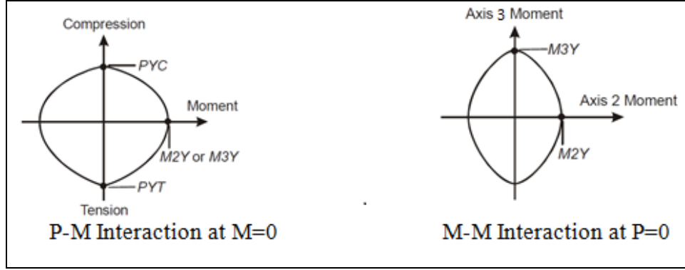
Figure 5.16: Yield Surface at M=0 and P=0.
