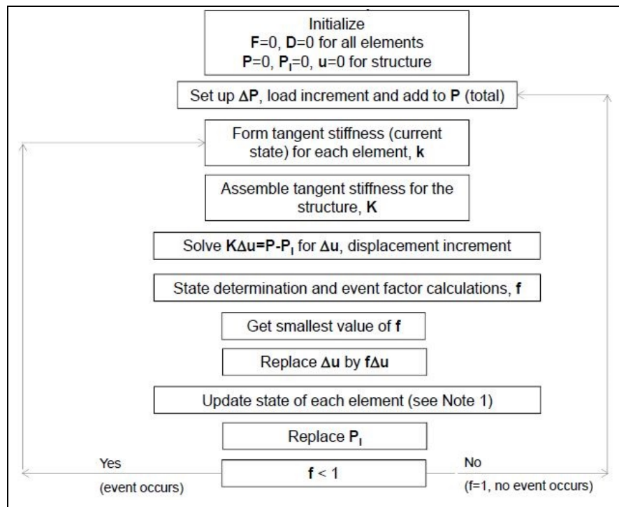
Figure 4.4: Detailed algorithm of total load.
