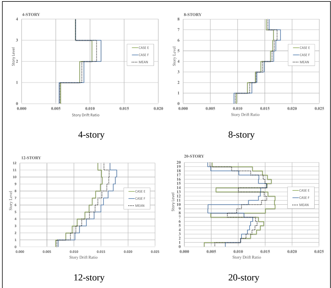
Figure 6.4: Story drift ratio of SCBF.
