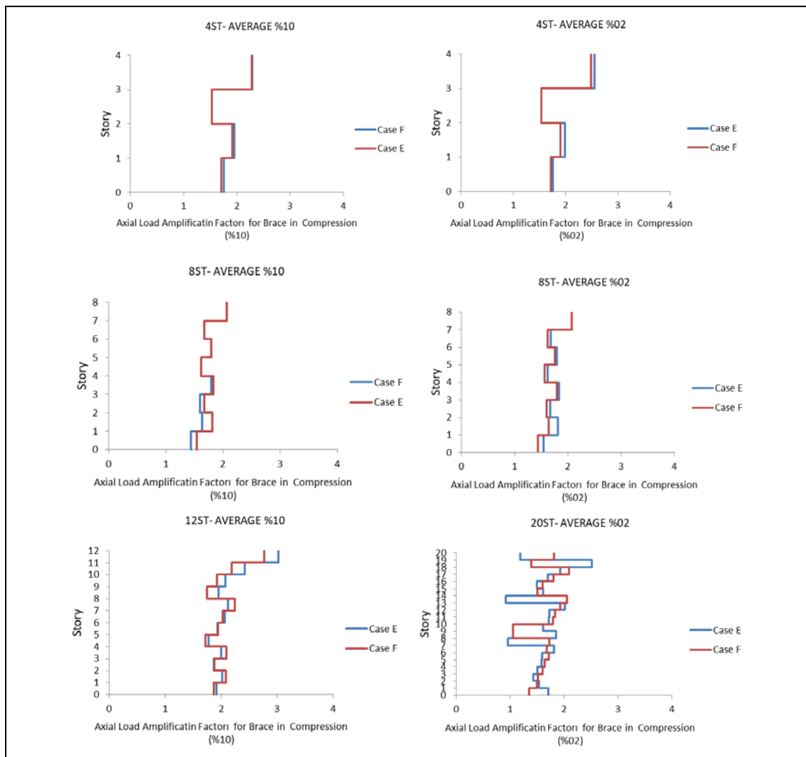
Figure 6.37: Maximum average axial compression amplification factor for brace corresponding to 2% and 10% probability of exceedance in 50 year.
