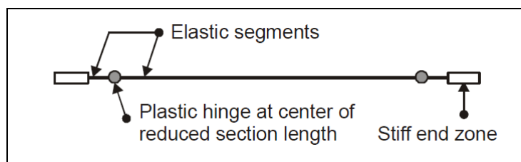
Figure 5.6: Model for Reduced Beam Section.
