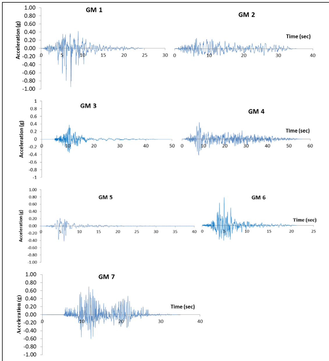
Figure 6.14: Acceleration time histories of the selected ground motions corresponding to 10% probability of exceedance in 50 year.
