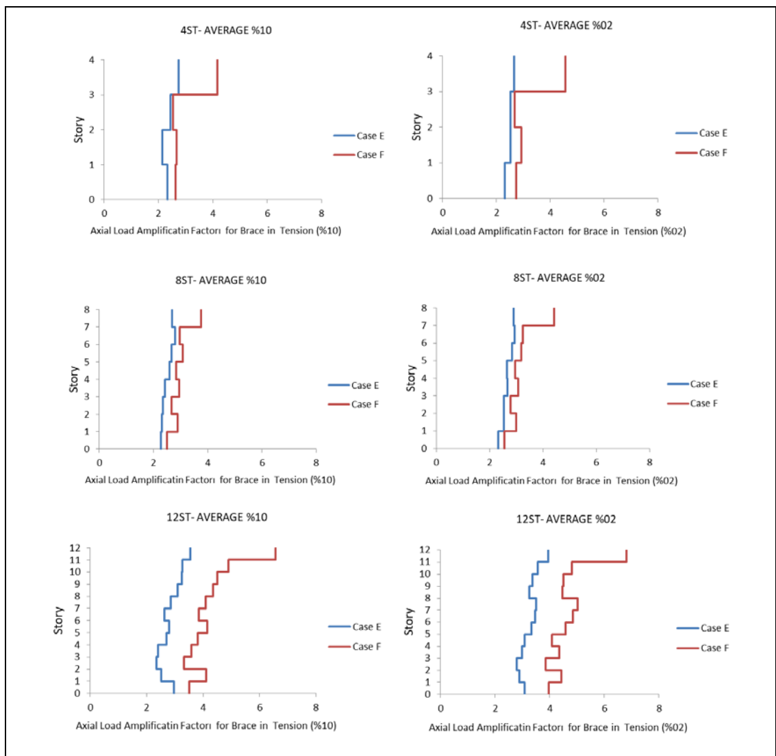
Figure 6.38: Maximum average axial tension amplification factor for brace corresponding to 2% and 10% probability of exceedance in 50 year.
