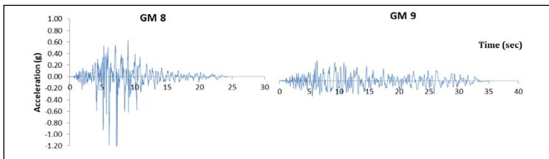
Figure 5.21: Acceleration time histories of the selected ground motions corresponding to 2% probability of exceedance in 50 year.
