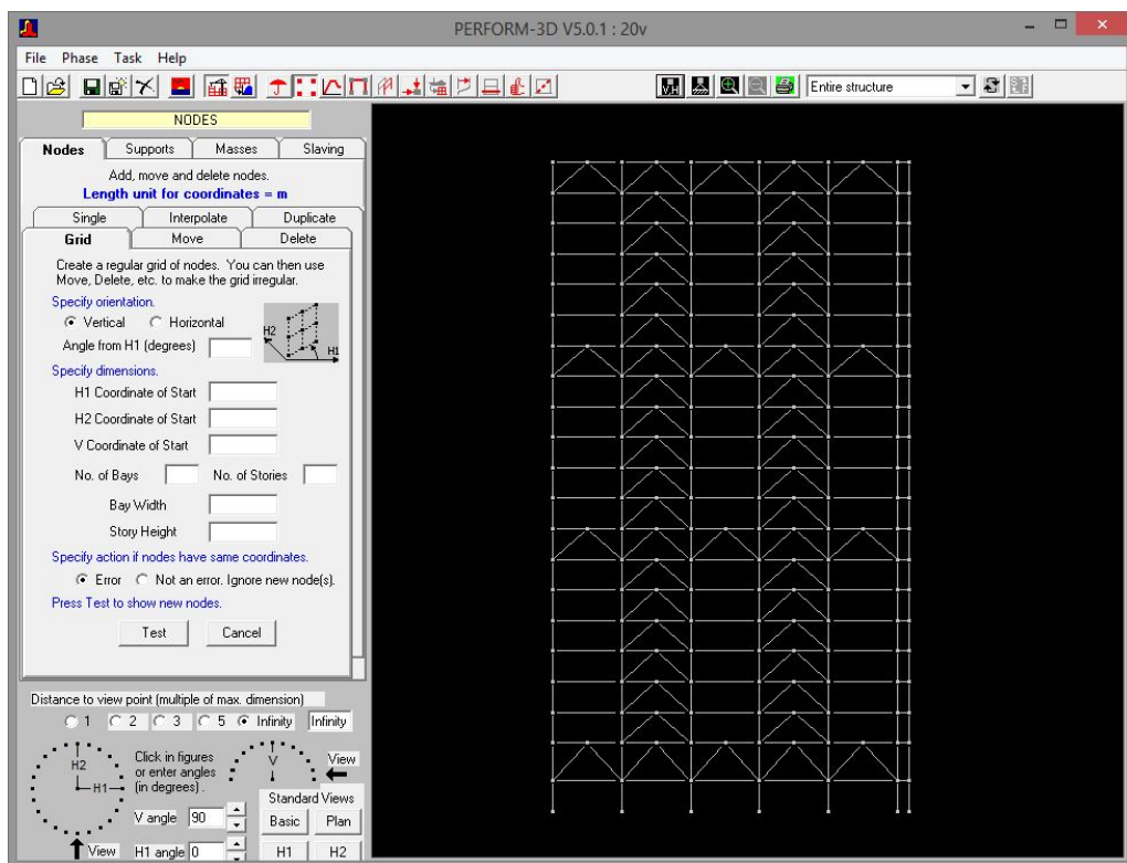
20 – Story Frame (two story Inverted-V Brace model)
