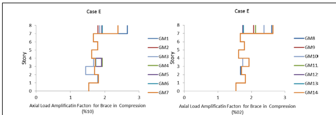
Figure 6.29: Maximum amplification factor for brace in compression in 8- story frames corresponding to 2% and 10% probability of exceedance in 50 year.
