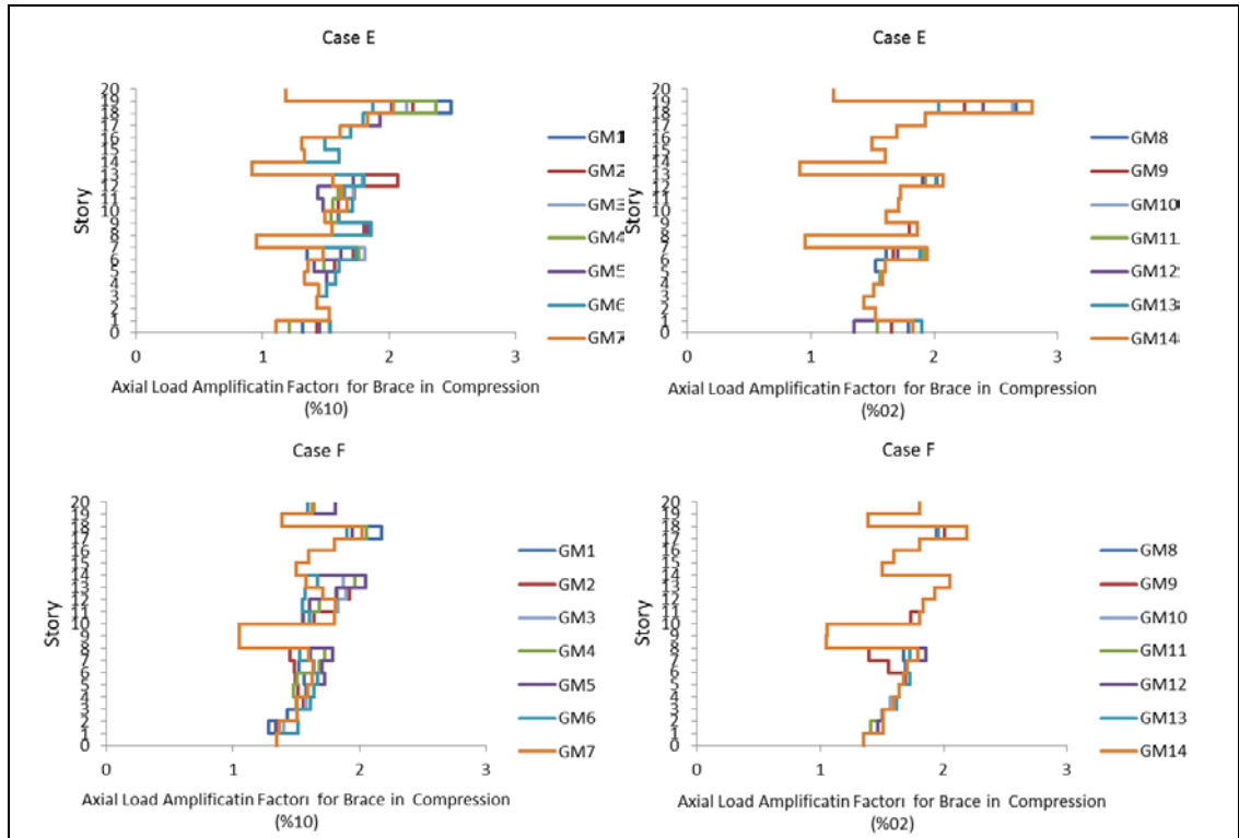
Figure 6.31: Maximum amplification factor for brace in compression in 20- story frames corresponding to 2% and 10% probability of exceedance in 50 year.
