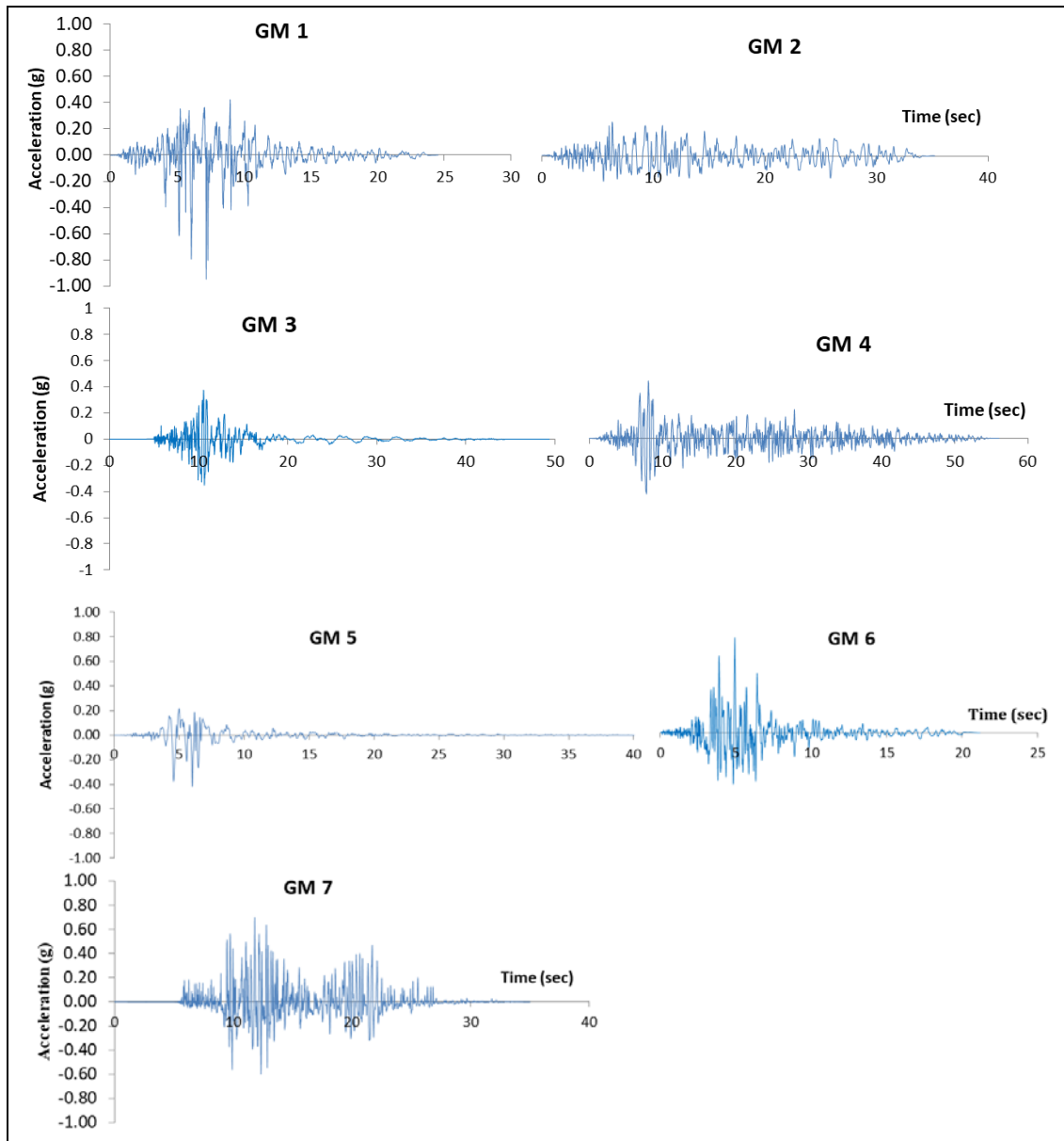
Figure 5.20: Acceleration time histories of the selected ground motions corresponding to 10% probability of exceedance in 50 year.
