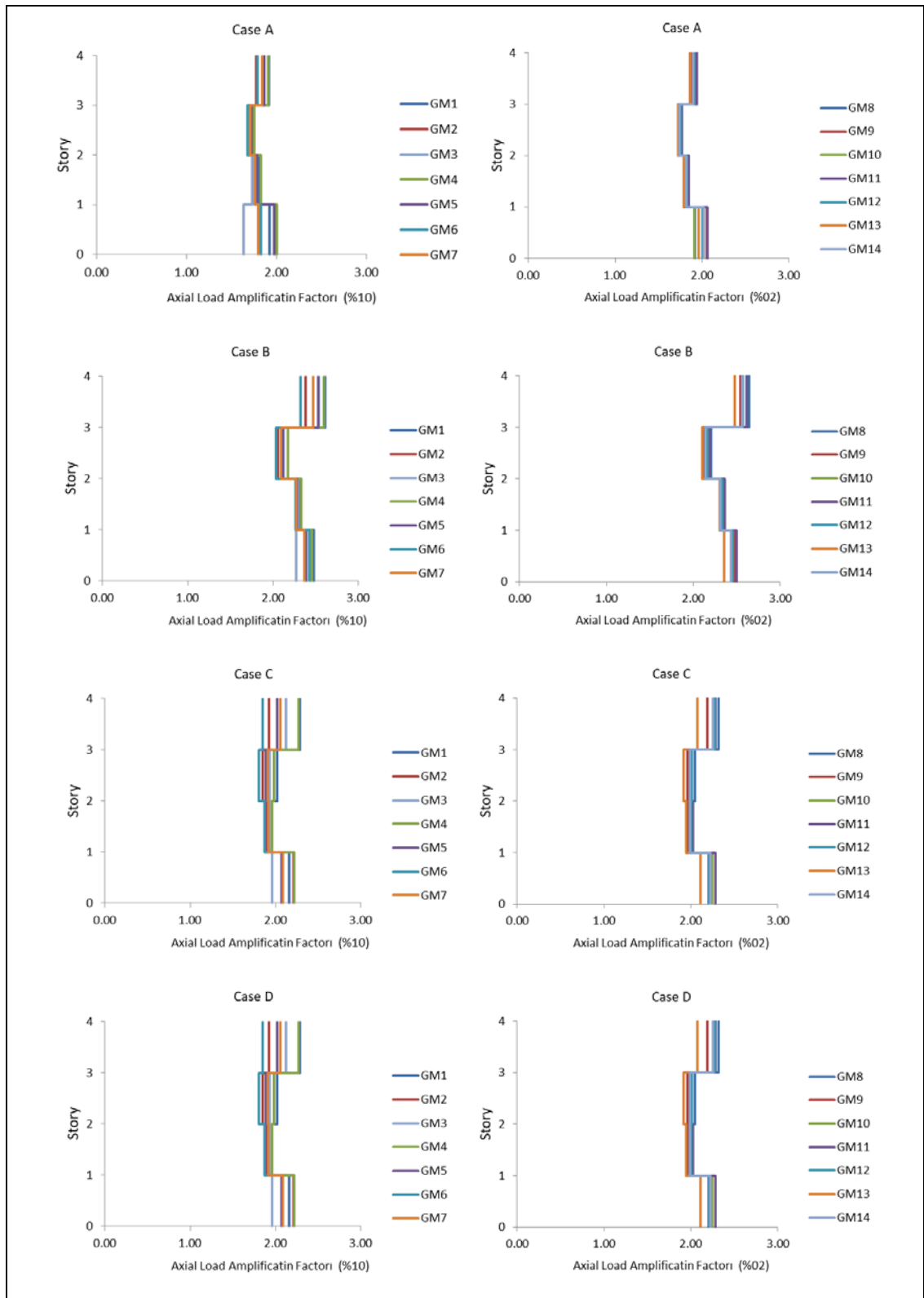
Figure 5.26: Maximum amplification factor for 4- story frames corresponding to 2% and 10% probability of exceedance in 50 year.
