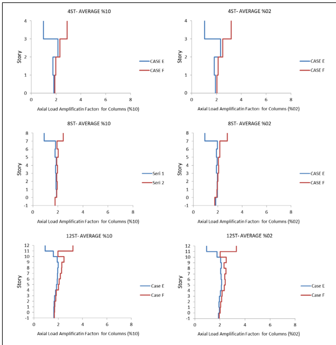
Figure 6.36: Maximum average axial compression amplification factor for column corresponding to 2% and 10% probability of exceedance in 50 year.
