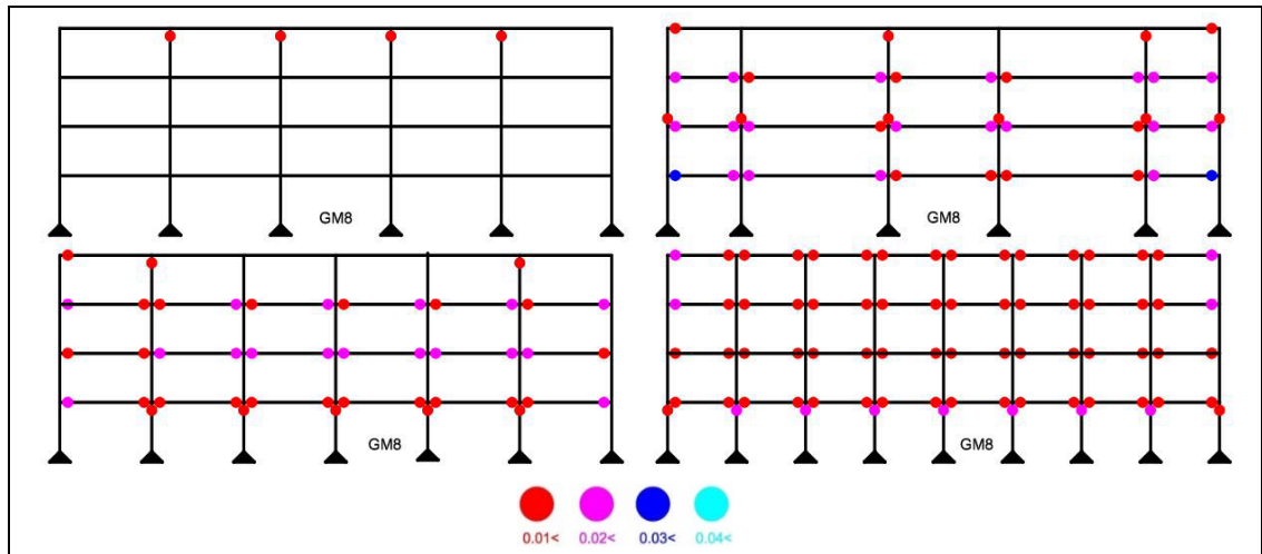
Figure 5.33: Highest plastic hinge rotations for 4 story frames.
