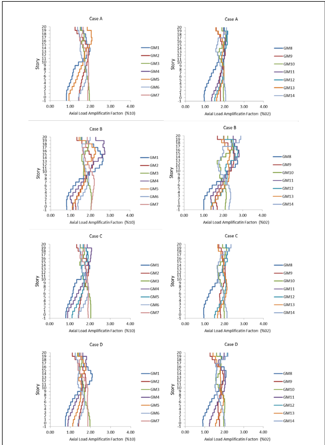
Figure 5.29: Maximum amplification factor for 20- story frames corresponding to 2% and 10% probability of exceedance in 50 year.
