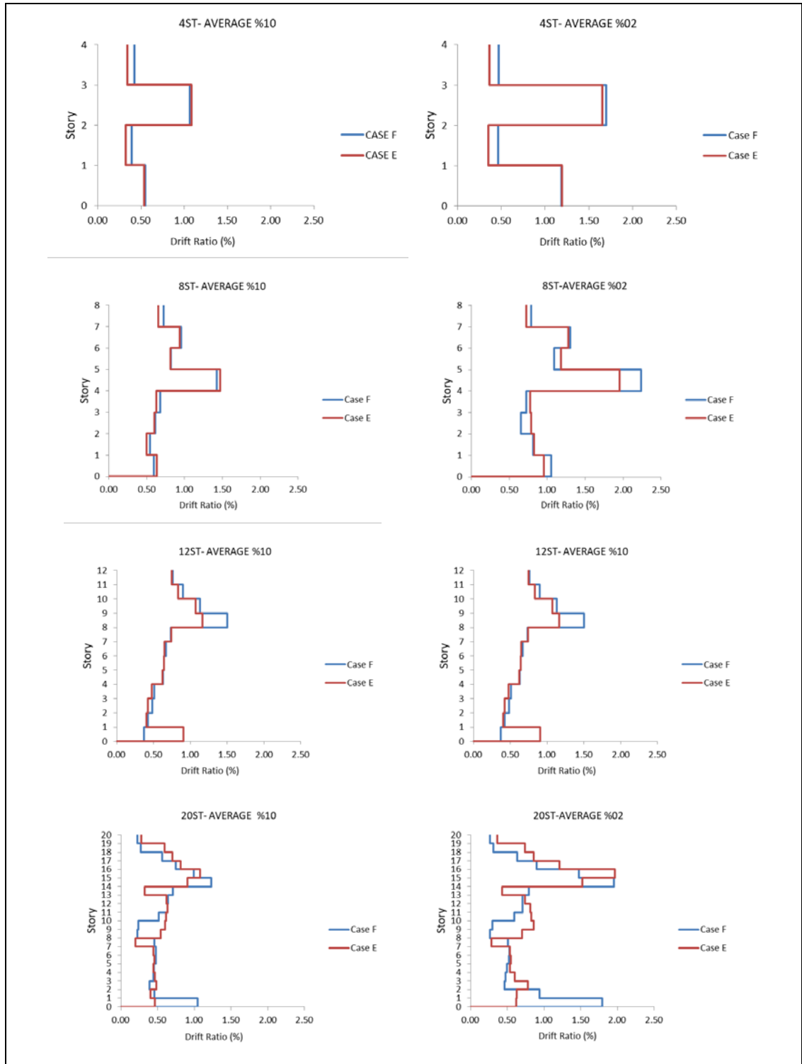
Figure 6.22: Average maximum drift ratio in frames corresponding to 2% and 10% probability of exceedance in 50 year.
