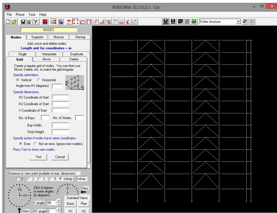
12 – Story Frame (two story Inverted-V Brace model)
