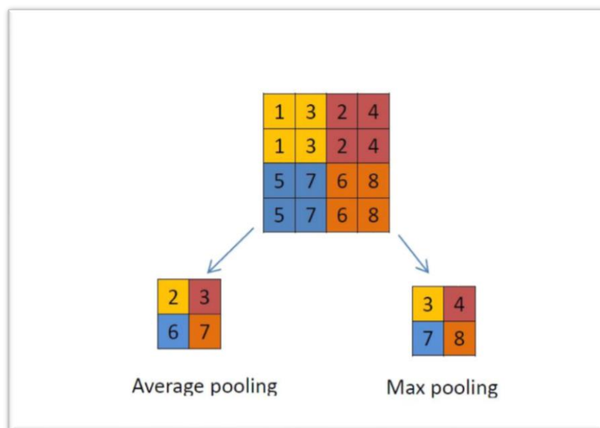
Figure 3.4: (on the left) Average pooling: The yellow box: (1 + 3 + 1 + 3) / 4 = 2 . (on the right) Max pooling: example of the blue box: \max(5, 7, 5, 7) = 7 .
