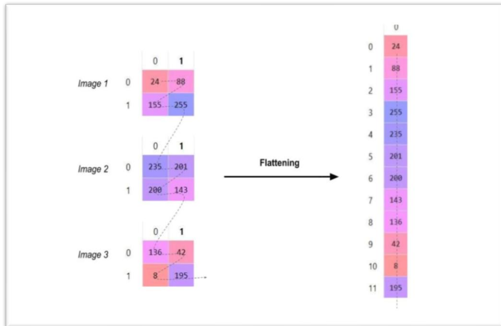
Figure 3.5: Final flattening of the final images of the filters + simplifications.
