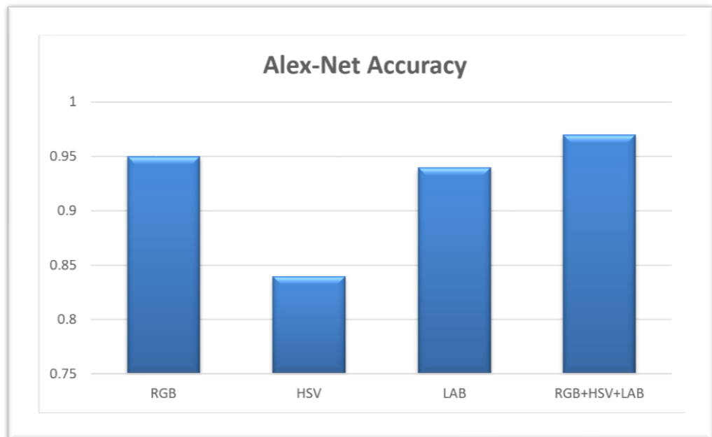
Figure 5.4: Validation Accuracy of Alex-Net on different color spaces.
