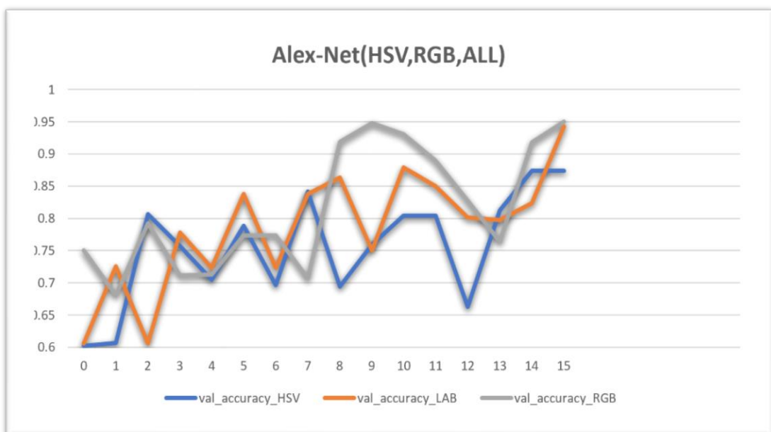
Figure 5.3: Validation Accuracy of Alex-Net on different color spaces.
