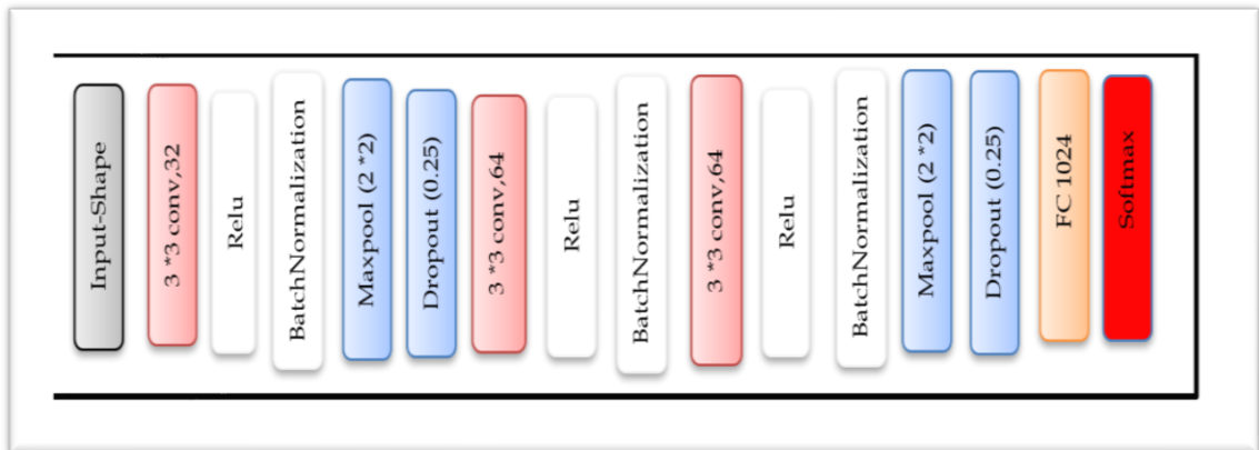
Figure 3.8: Custom Cnn Architecture.
