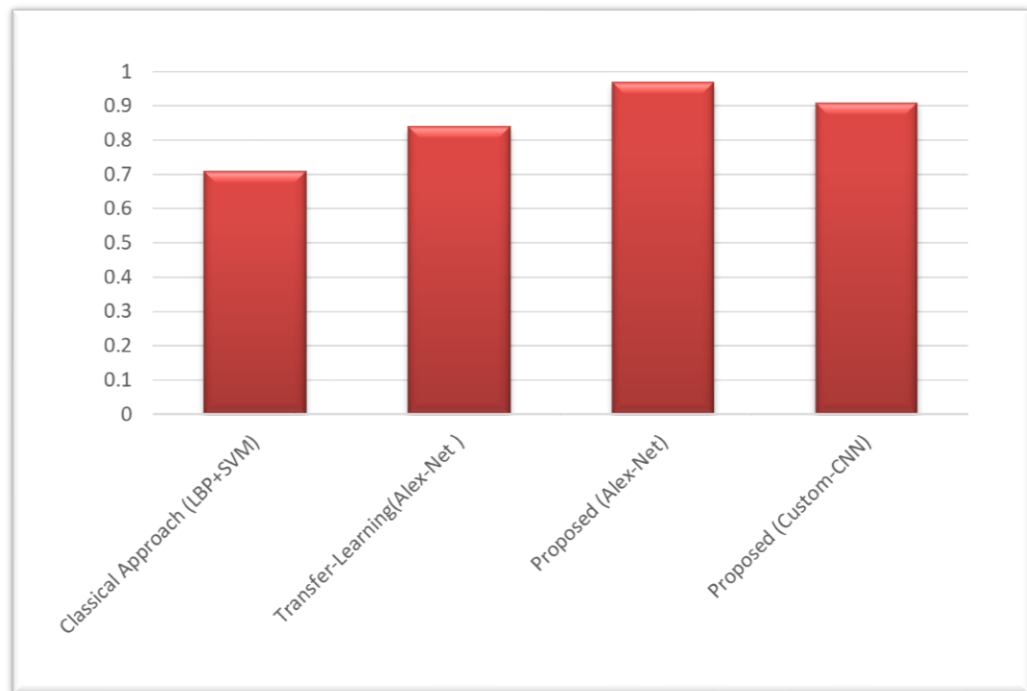
Figure 5.6: Comparison of Validation accuracy of the proposed method and Other Approaches.
