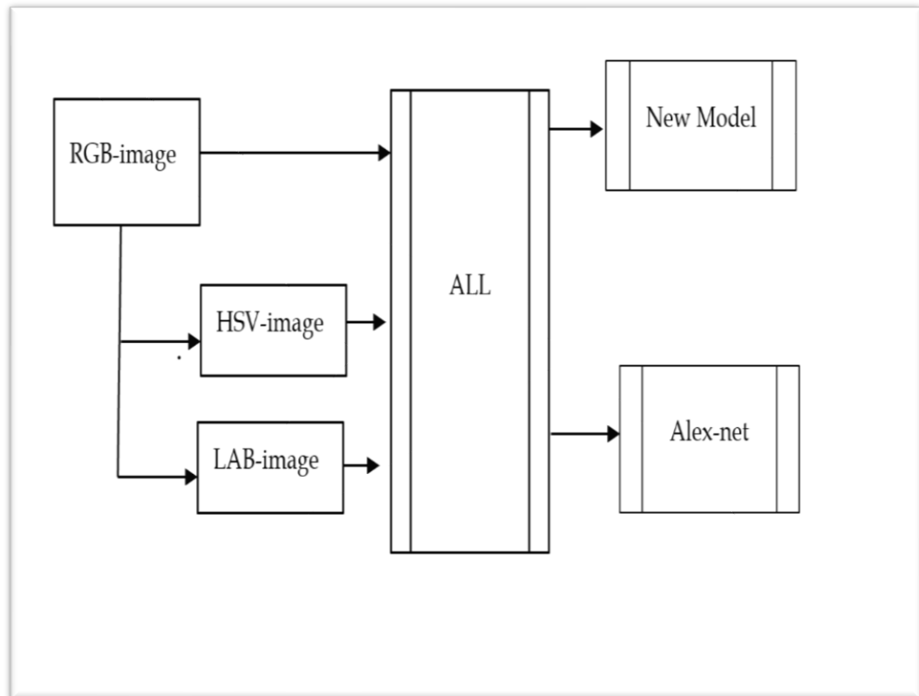
Figure 3.10: Model Architecture.
