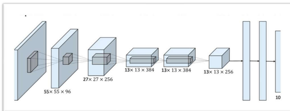
Figure 3.7: Alex-Net Architecture.
