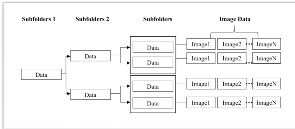
Figure 4.2: Data arrangement.
