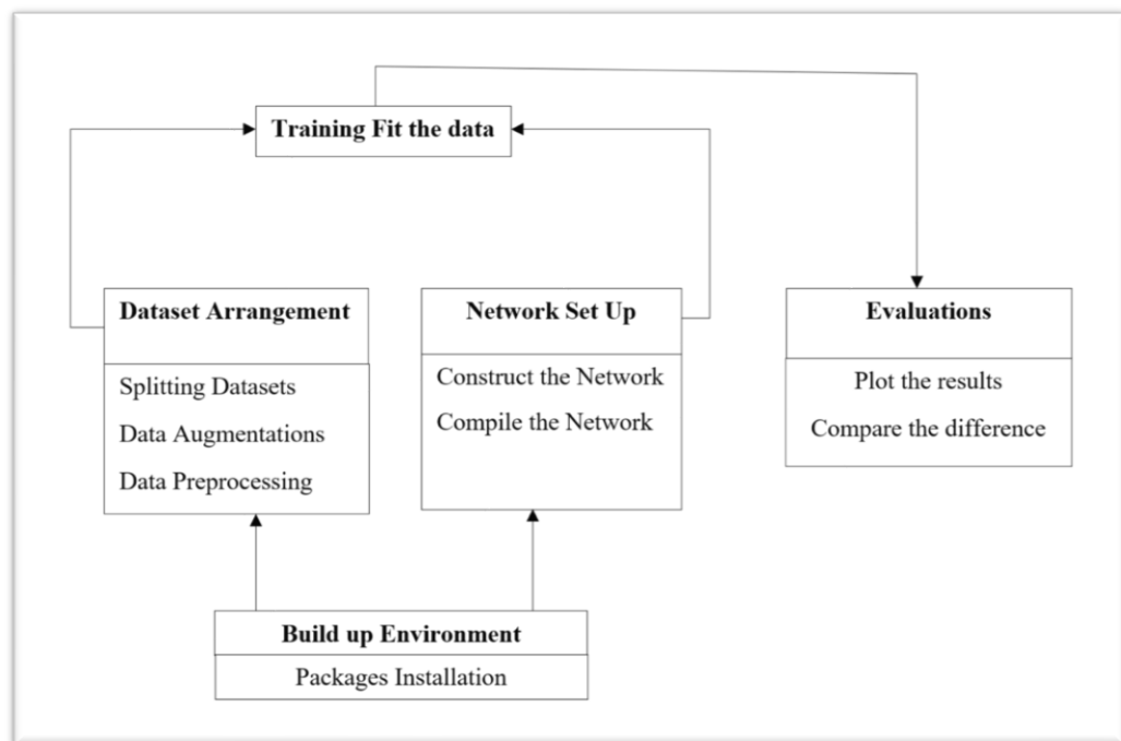
Figure 4.1: General workflow.
