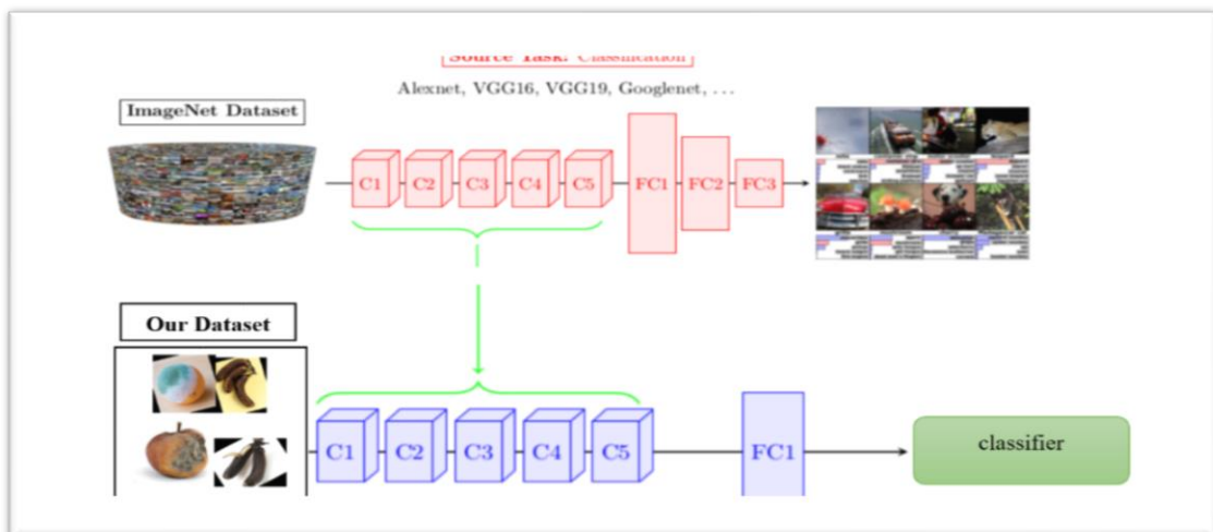
Figure 2.3: Pipeline of transfer learning.
