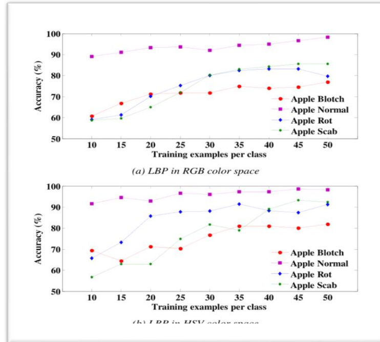
Figure 2.1: Accuracy of SVM classifier for apple diseases.
