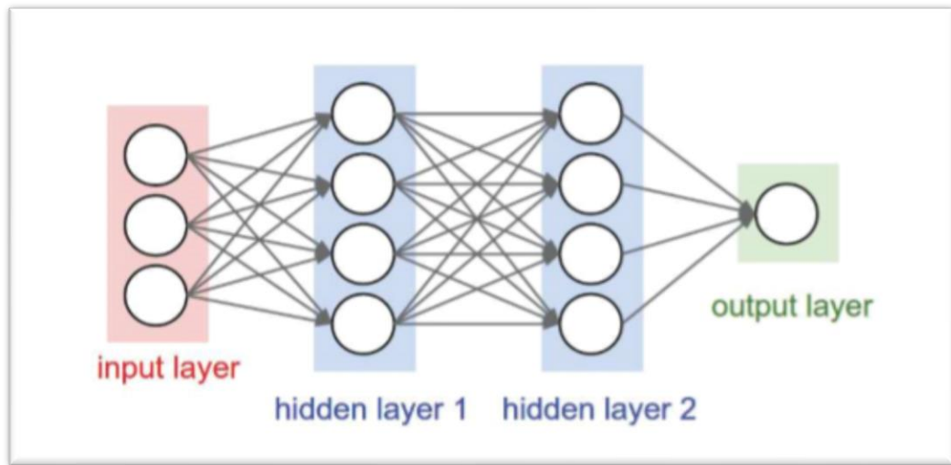
Figure 3.1: Neural network or neural networks with two hidden layers; fully connected neural network.
