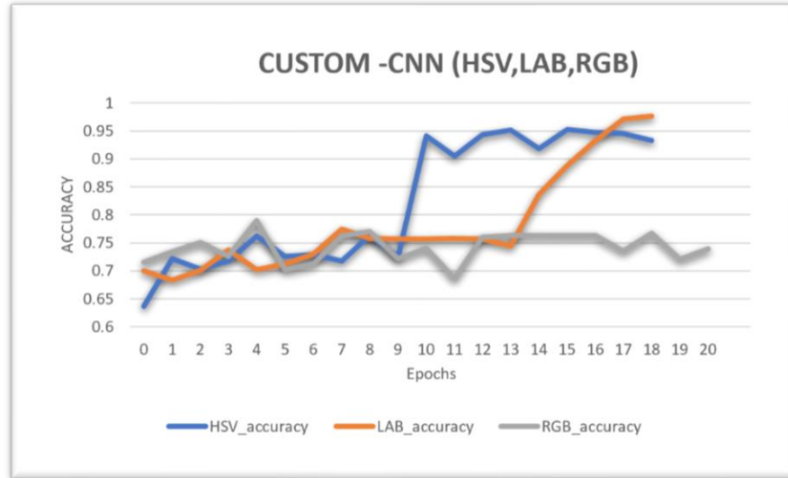
Figure 5.1: Validation Accuracy of custom-CNN on different color spaces.
