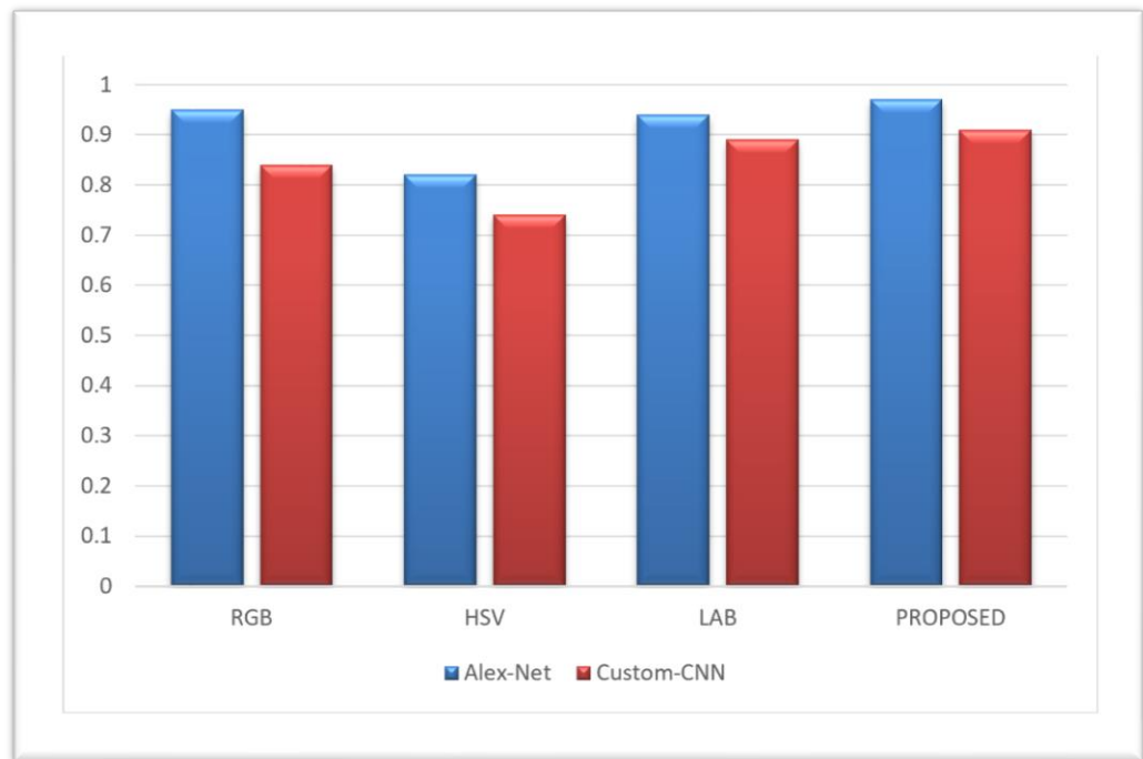
Figure 5.5: Comparison of Validation accuracy of Alex-Net and Custom-CNN.
