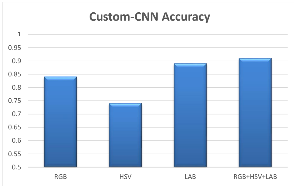
Figure 5.2: Validation Accuracy of Custom-CNN on fusion color spaces.
