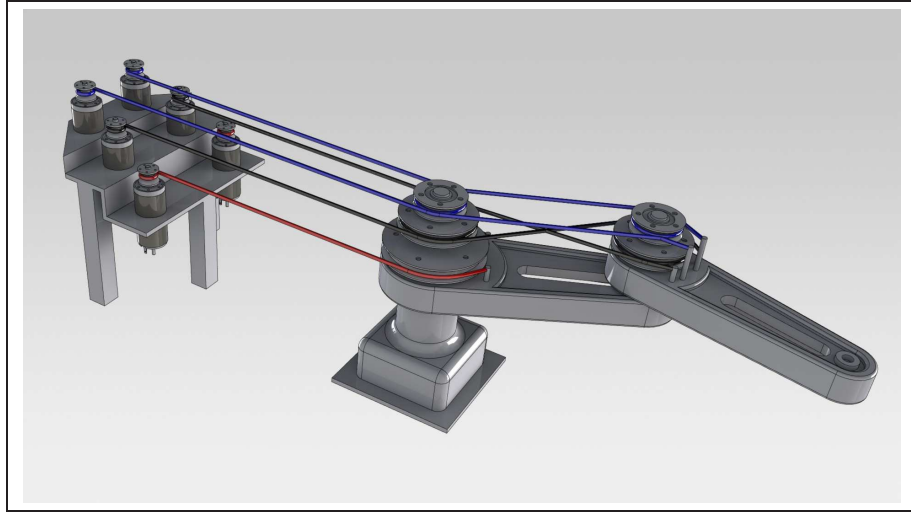
Figure 4.1: Overall view of two link planar robot driven by six tendons.
