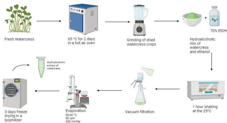
Figure 2.1. Schematic representation of watercress EtOH extraction.
